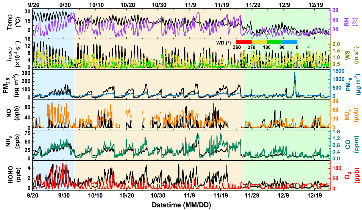
Figure 1: Hourly time series of meteorological parameters (Temp, RH, WS, WD, j_{\text{HONO}} ) and chemical species (HONO, \text{O}_3 , NO, \text{NO}_2 , \text{NH}_3 , CO, \text{PM}_{2.5} , \text{PM}_{10} ) concentrations from 20 September to 23 December 2022. The blue, yellow and green shades represent DHP, PEP and CLP, respectively. (DHP: Double-High Pollution Period, characterized by double-high levels of both \text{O}_3 and \text{PM}_{2.5} ; PEP: \text{PM}_{2.5} Episodic-cycle Pollution Period, characterized by periodic cycle of \text{PM}_{2.5} pollution; CLP: Clean Low Pollution Period, characterized by relatively low pollutant concentrations.) The color bar in the second subfigure represents wind direction (WD) in degrees.
