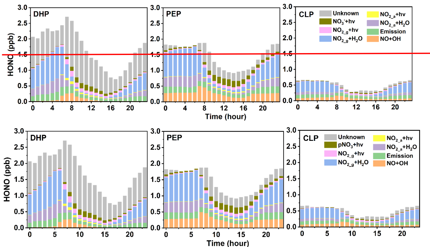
Figure 4: The diurnal variations of the \text{HONO}_{\text{sim},0} from different sources during the DHP, PEP and CLP.
