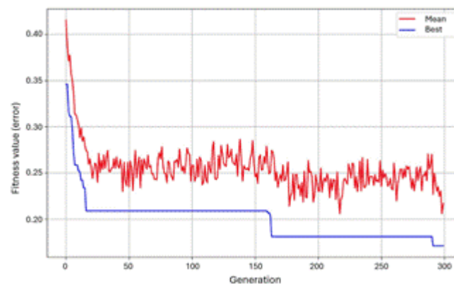
Figure 7. Genetic Algorithm Convergence: the curves show the population’s average performance (Mean) and the best individual’s performance (Best) across an evolution of 300 generations.
