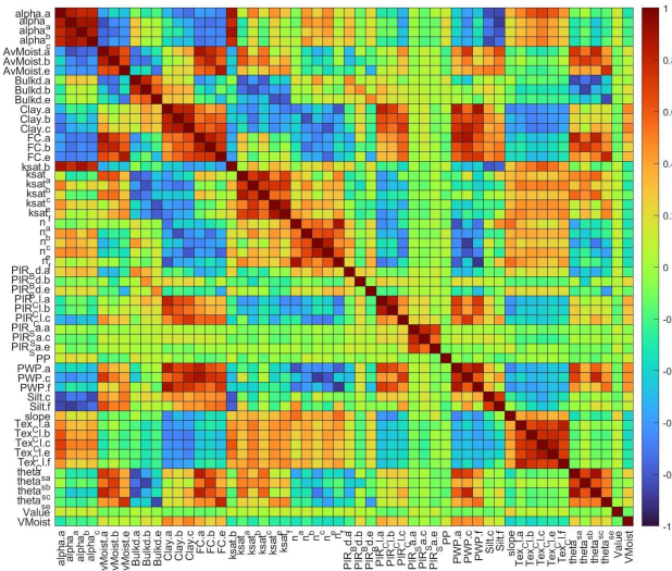
Figure 4. Correlation matrix for the 53 less correlated variables (correlation under the threshold of |0.9| ). These less correlated variables are presented in Table 3.
