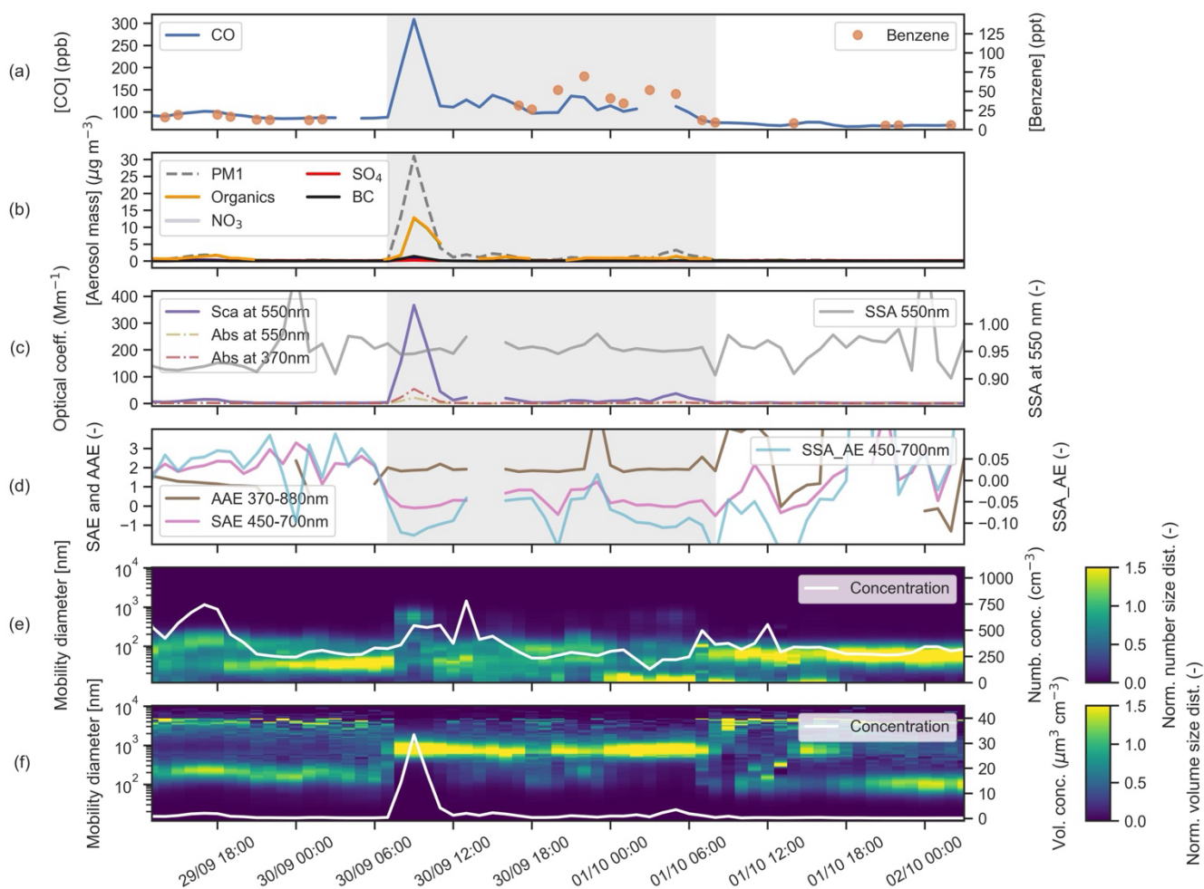
Figure 3: Time series of gas and aerosol properties measured in situ in the smoke plume as it passed over JFJ on September 30 and October 1, 2023: (a) concentrations of carbon monoxide (CO) and benzene in the gas phase; (b) the mass concentrations of all particles with diameters less than 1 \mu\text{m} (PM1) as well as the organic components (Organics), nitrate ( \text{NO}_3 ), sulphate ( \text{SO}_4 ), and black carbon (BC); (c) scattering coefficients 550 nm and absorption coefficients at 370 and 550 nm, and single scattering albedo (SSA) at 550 nm; (d) scattering Ångström exponents (SAE) from 450 – 700 nm, absorption Ångström exponents (AAE) from 370 – 880 nm,
