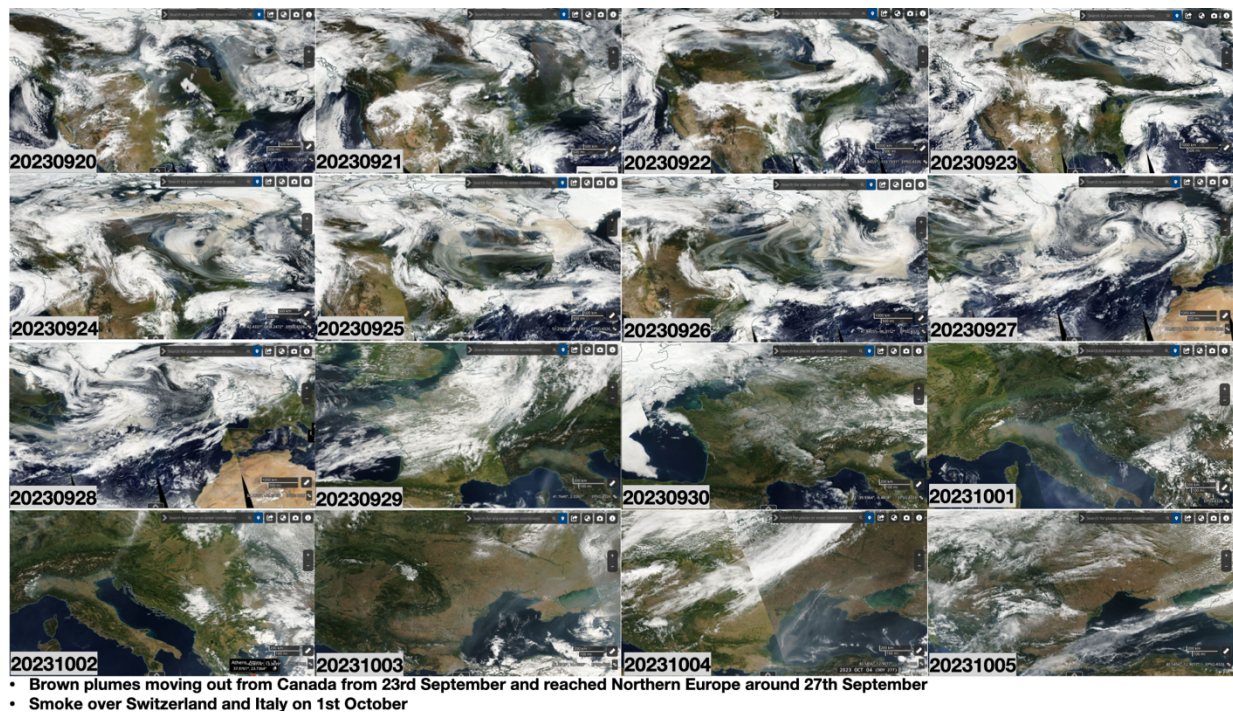
750 Figure C1: MODIS true colour images tracing the plume. Imagery credits: © Land Atmosphere Near real-time Capability for EOS (LANCE) system and Global Imagery Browse Services (GIBS), operated by NASA Earth Observing System Data and Information System (EOSDIS).
