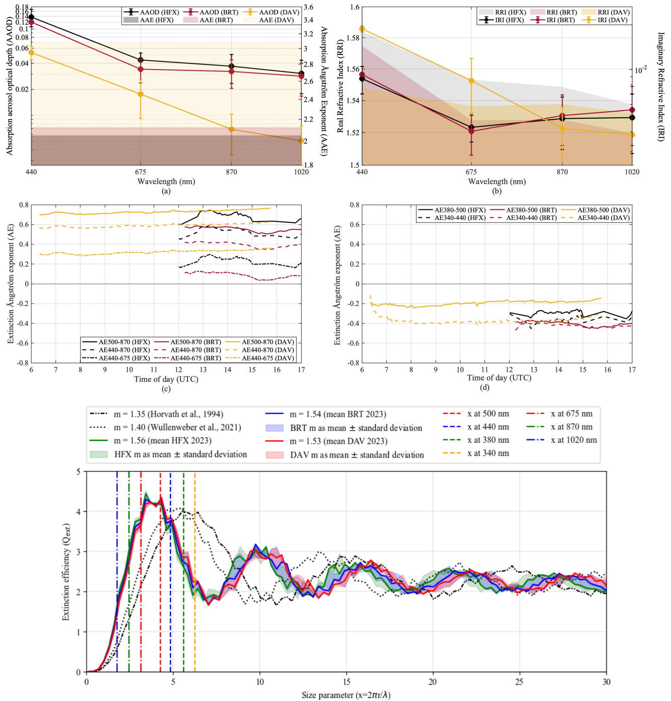
Figure 9: Average (a) absorption AOD (shown as line) and absorption AE (shown as area) in logarithmic axis and (b) real (shown as area) and imaginary (shown as line) refractive indices and the variation of extinction AE in the spectral range that exhibited (c) positive and (d) negative values at stations HFX, BRT and DAV during the peak day of the event based on data availability from AERONET inversion products. (e) Extinction efficiency for specific refractive index and size parameter at wavelength in the range 340-1020 nm from Mie scattering with homogeneous spherical particles.
