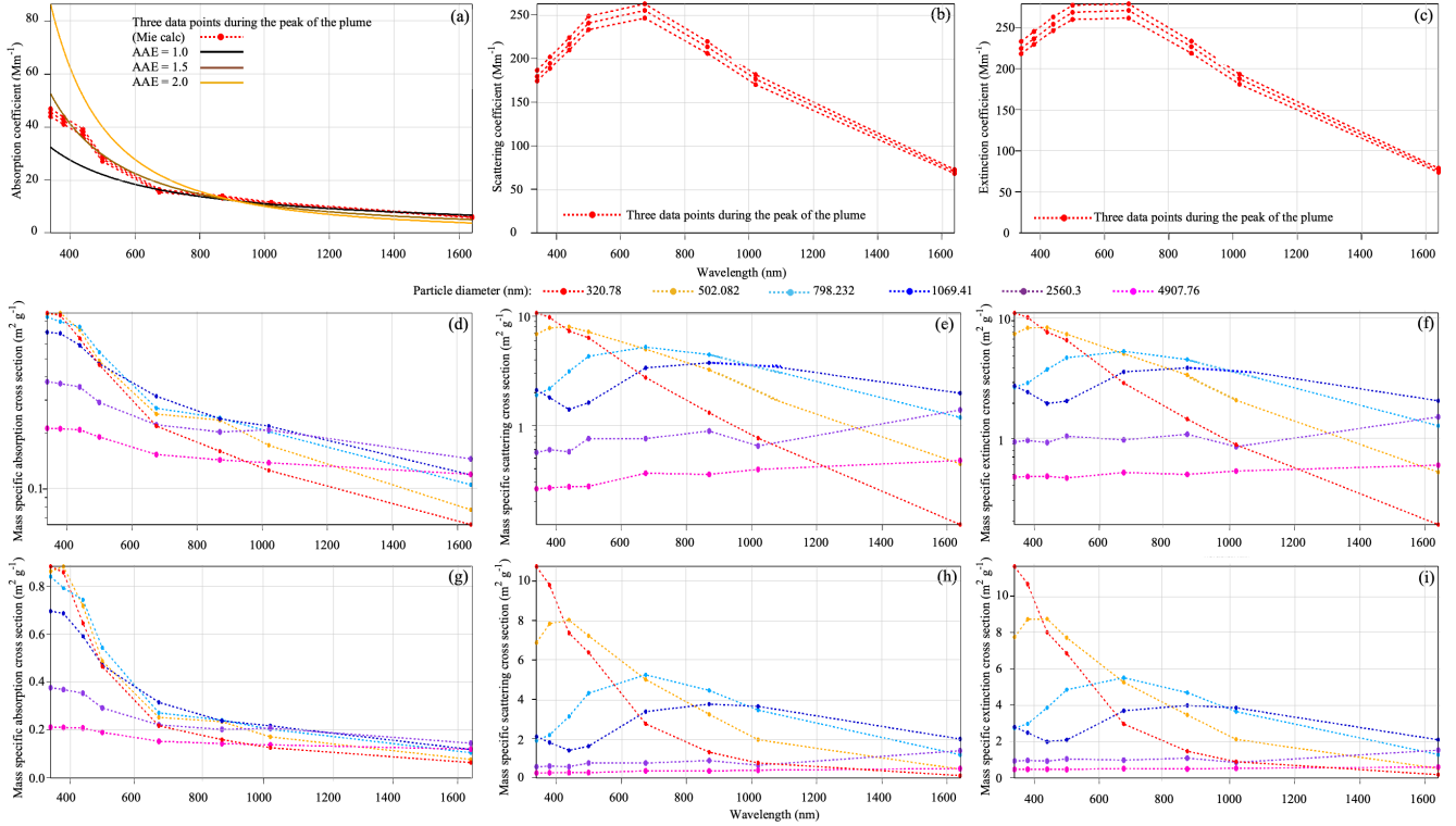
Figure 5: Absorption (a), scattering (b), and extinction (c) spectral profiles calculated at three points during the peak of the plume using Mie theory and the assumption of homogeneous spheres with size distributions constrained by the in situ measurements and a single, effective refractive index given by the corresponding AERONET retrieval. Panels (d), (e), and (f) show the absorption, scattering and extinction profiles, respectively, of monodisperse homogeneous spheres of various sizes, to assess the sensitivity of these profiles to particle diameter. Panels (g), (h), and (i) show the same curves on a linear y-axis.
