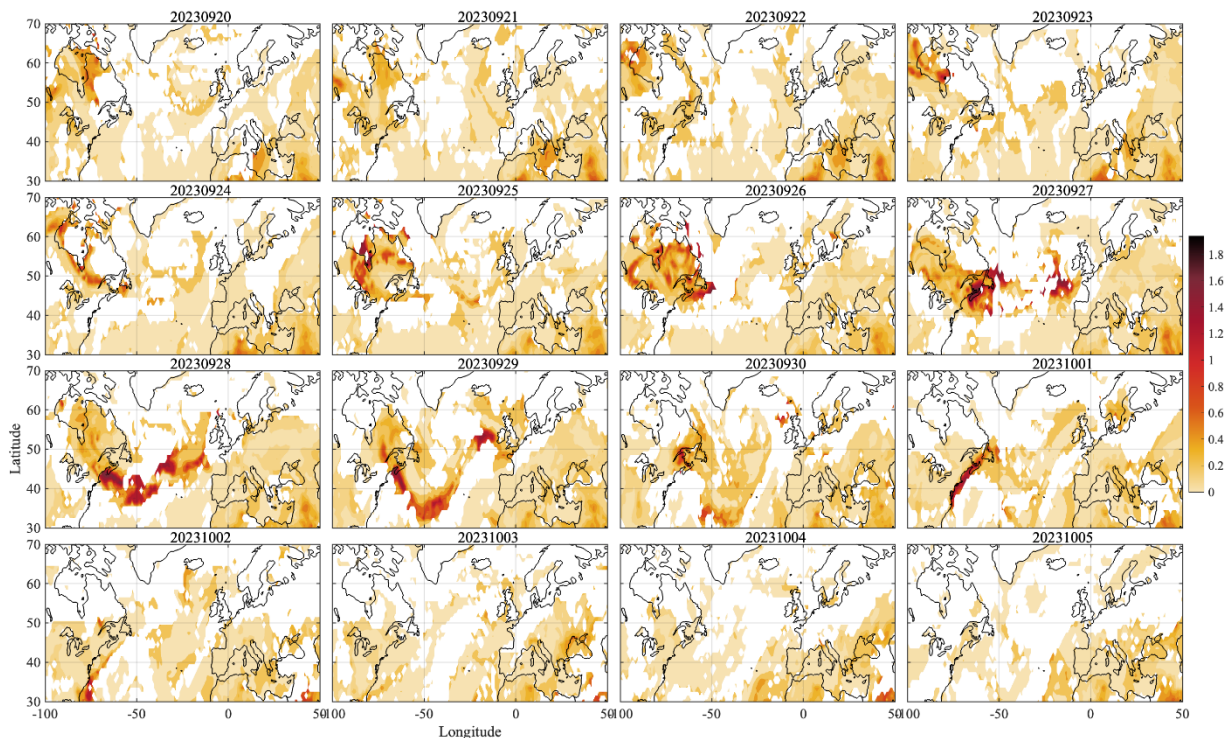
Figure A4: MODIS AOD at 550 nm during 20 September and 05 October 2023.
