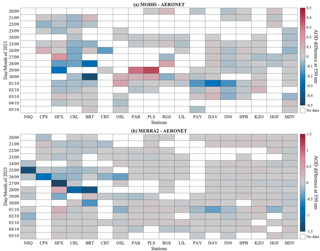
615 Figure 10: Daily mean AOD difference of AERONET AOD from (a) MODIS and (b) MERRA2 AOD at 550 nm for all stations from 20 September to 05 October 2023. AERONET AOD at 500 nm is interpolated to 550 nm using Ångström power law for comparability.
