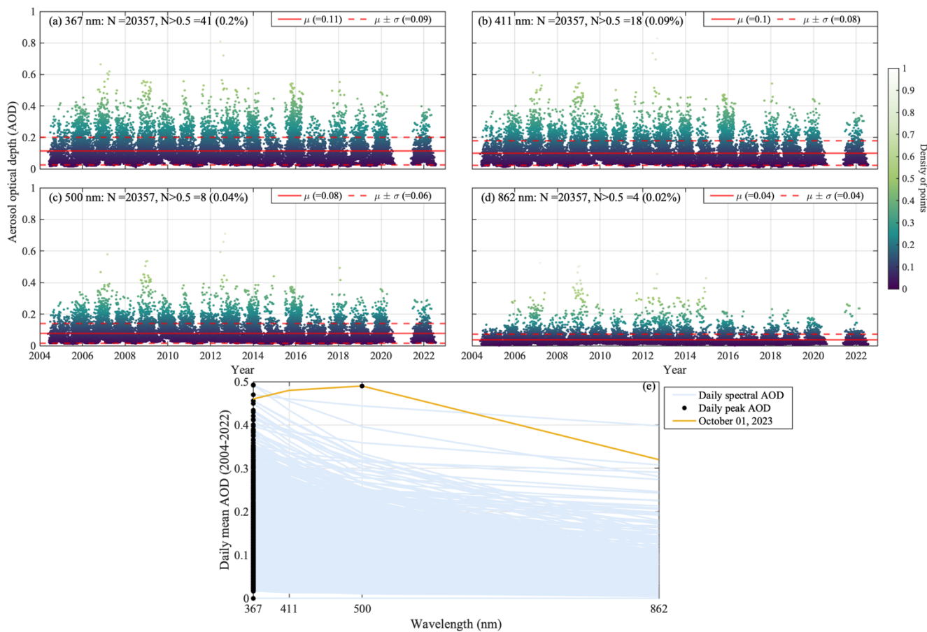
740 Figure B1: (a-d) Climatological AOD variation at 367, 411, 500 and 862 nm and, (e) Daily mean spectral AOD and (e) daily spectral maxima (black dots) between 2004-2022 from GAWPFR 01 October 2023 (yellow) at DAV
