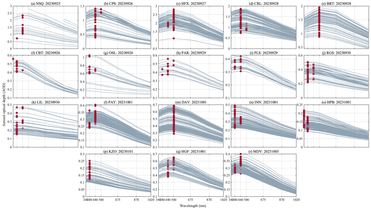
Figure 7: (a-r) Spectral variation (curvature) of AOD on the peak day of the event at the respective stations (blue lines). Red dots indicate the peak AOD value at one time instance. Each grey curve here represents instantaneous spectral values.
