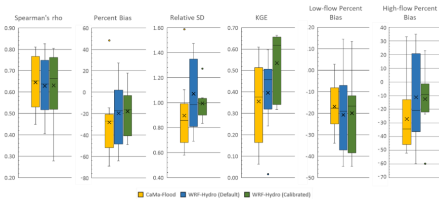
505 Figure 8: Performance metrics for each model experiment (with Adige basin excluded). The X represents the mean value.
