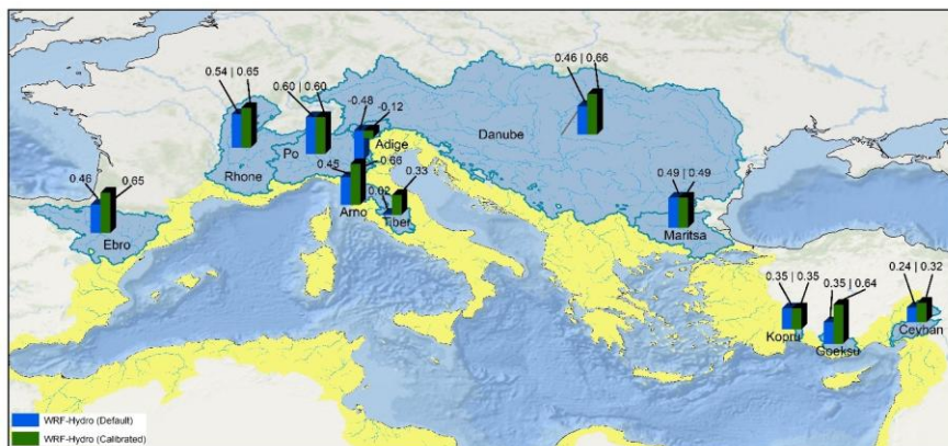
450 Figure 5: Comparison of KGE values between calibrated and non-calibrated WRF-Hydro model across the selected basins.
