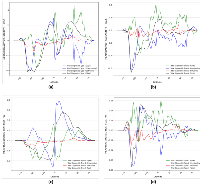
Figure 11. (a) Salinity transport ( \text{kg/s} ) partitioned into type for antwater 60S in 950\text{-}1150 . (b) Salinity transport anomaly ( \text{kg/s} ) partitioned into type for antwater 60S relative to piControl . (c-d) Same as above for northward heat transport (PW).
