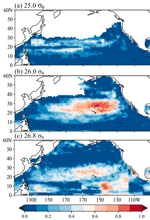
Figure S2. Coefficient of determination for linear regression lines along the isopycnal surface of 25.0 (a), 26.0 (b), and 26.8 \sigma_\theta (c).
