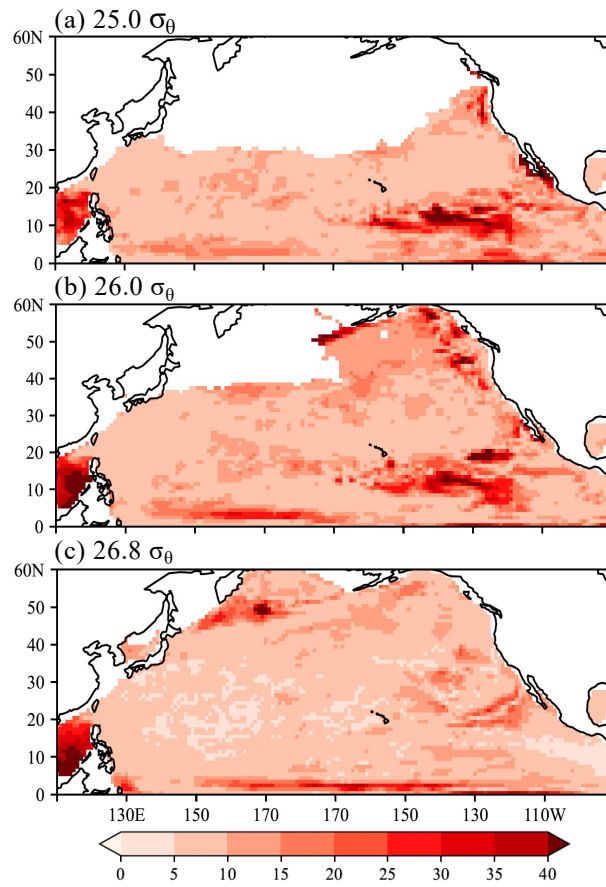
Figure S1. Uncertainty estimates of dissolved oxygen concentration ( \mu\text{mol/kg} ) along the isopycnal surface of 25.0 (a), 26.0 (b), and 26.8\sigma_\theta (c). The uncertainty data is based on GOBAI- \text{O}_2 data [ Sharp et al. 2023 ].
