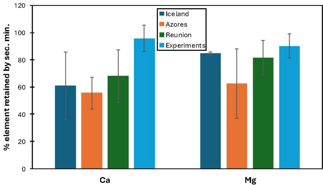
Fig. 2: Estimates of the proportion of Ca and Mg from weathered basalt ending up in secondary precipitates (notably clay minerals), for Iceland, Azores (Pogge Von Strandmann et al., 2010) , Reunion (Louvât and Allègre, 1997). The basalt weathering experiments are from Pogge von Strandmann et al. (2019). The overall method of the mobility calculation comes from Gislason et al. (1996). The error bars are the variability in the different rivers. 410
