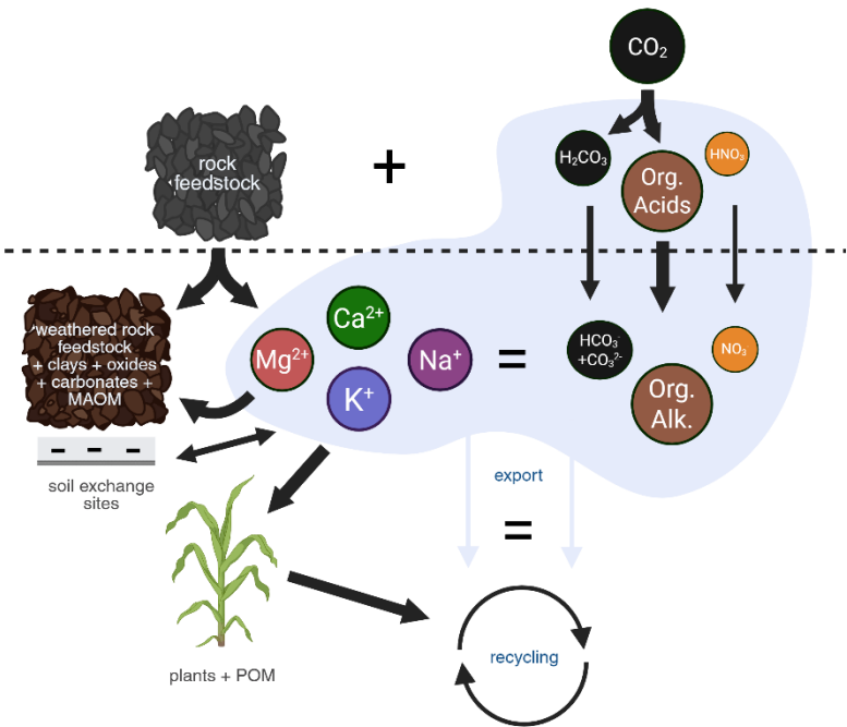
Fig. 1: Cations released from rock feedstock (cation alkalinity) is balanced by the sum of carbonate alkalinity, organic alkalinity and e.g. nitrate from fertilizer nitrification. The relative contribution of the acids is indicated by the thickness of the arrows. Note that their relative importance can vary in different soils and under different conditions. Most of the cations will be incorporated into the crop and clay minerals. The latter stabilize soil organic matter as a transient pool of MAOM. Created in BioRender. Reershemius, T. (2025) https://BioRender.com/9vz62gz
