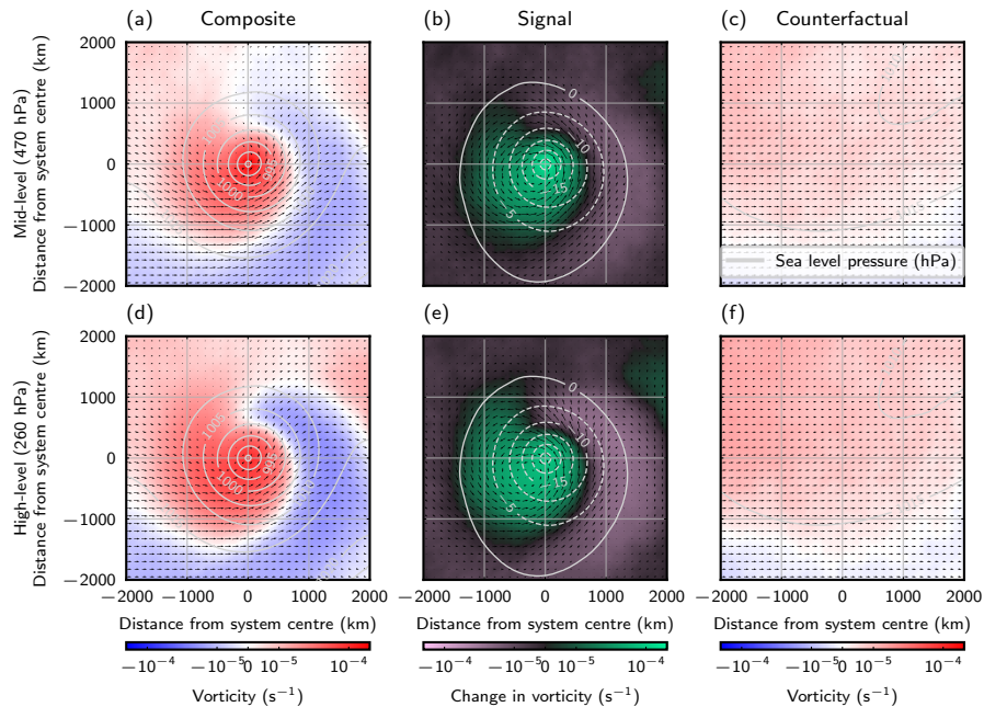
Figure B1. Composite, signal, and counterfactual (as Fig. 3) of the relative vorticity. Data is shown for the two vertical levels presented in Figs 1 and 3.
