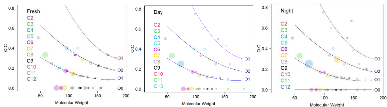
187 Figure S11: Average VOCs/IVOCs per experiment phase as detected by the Tenax tubes in 188 terms of the molecule oxygenation and the molecular weight (experiment DN4). Color 189 indicates the carbon number, while the depicted lines the oxygen number. The size is 190 proportional to the concentration on a logarithmic scale.
