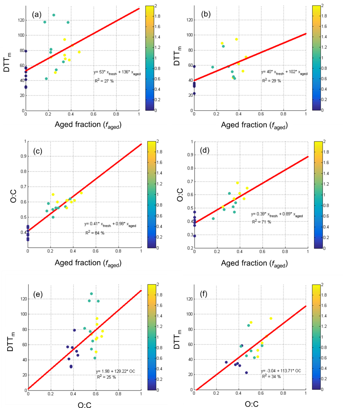
193 Figure S12: (a, b) Correlation between WS-OP, expressed as DTT m activity (pmol min -1 194 \mu\text{g}^{-1} ), and the aged fraction of OA for DN (a) and ND (b) oxidation cycles. (c, d) Correlation 195 between the O:C ratio and the aged fraction of OA for DN (c) and ND (d) oxidation cycles. (e, 196 f) Correlation between WS-OP and the O:C ratio for DN (e) and ND (f) oxidation cycles. Color 197 bars on the right of each diagram indicate oxidation stages, where 0, 1, and 2 correspond to 198 fresh aerosol, first-stage oxidation, and second-stage oxidation, respectively. For fresh OA, the 199 aged fraction is zero.
