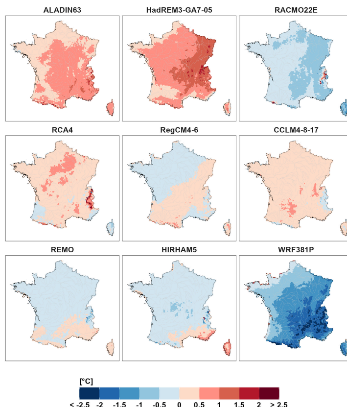
Figure 10. Main effects (i.e. deviations from the ensemble mean) of individual climate models for summer temperature changes (2071-2099 relative to 1976-2005). (A) GCMS. (B) RCMs.
