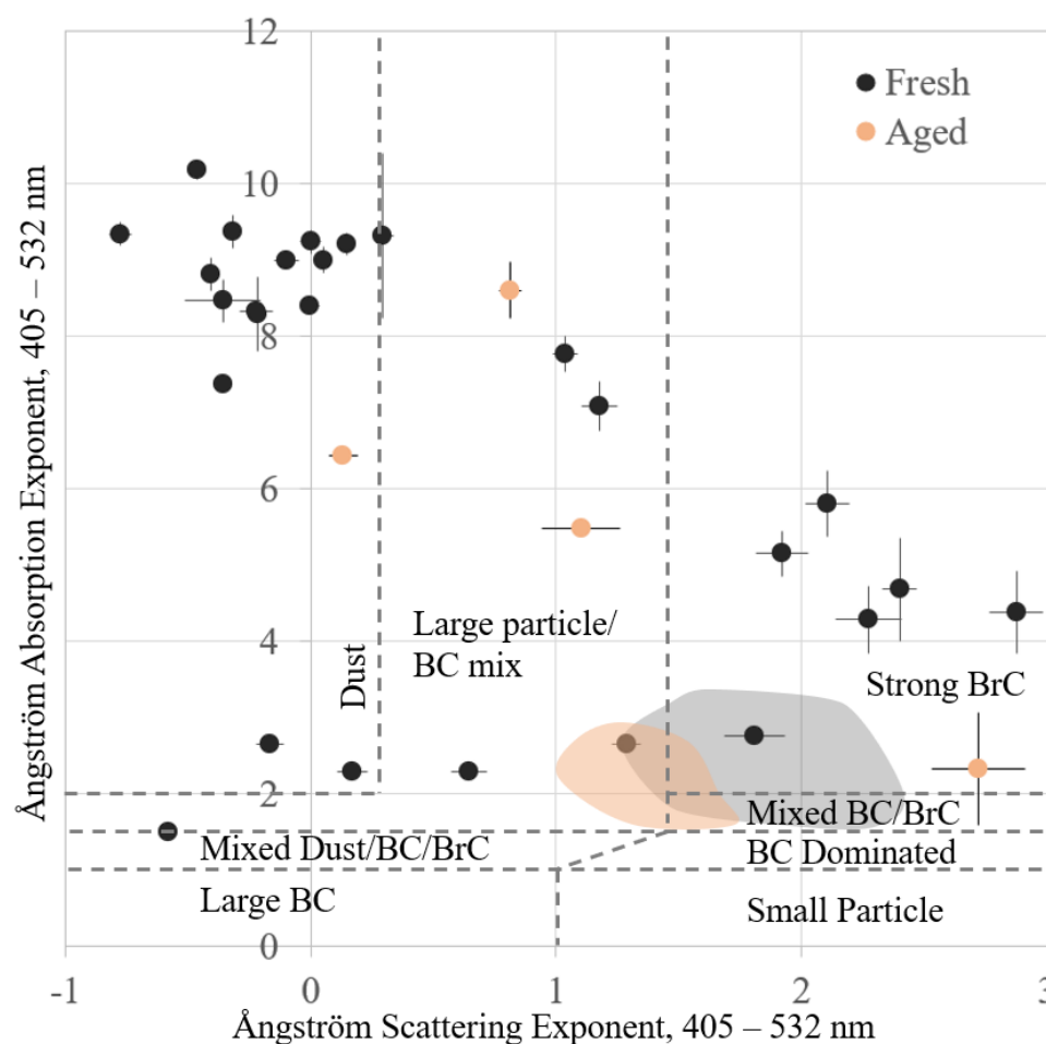
Figure 4. The Ångström matrix plot (ASE vs AAE) for fresh and PAM-aged observations in this work and previous work on similar fuels (in shaded areas) (McRee et al., 2024).
