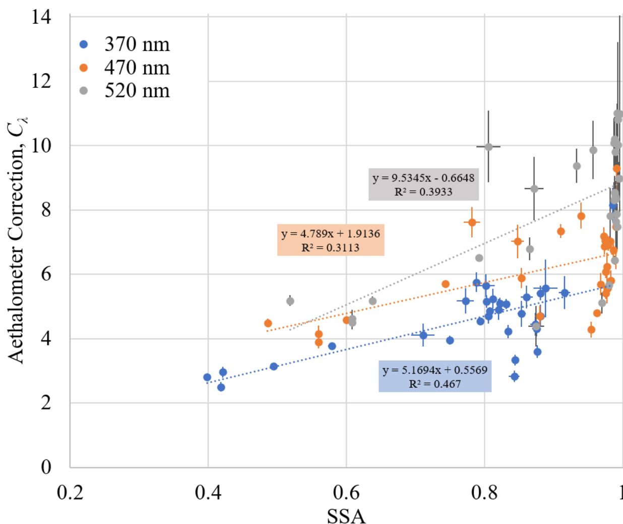
Figure 3. The aethalometer correction factor C_\lambda plotted against SSA at three wavelengths. PAM oxidation experiments were included. Results of a linear fit are shown.
