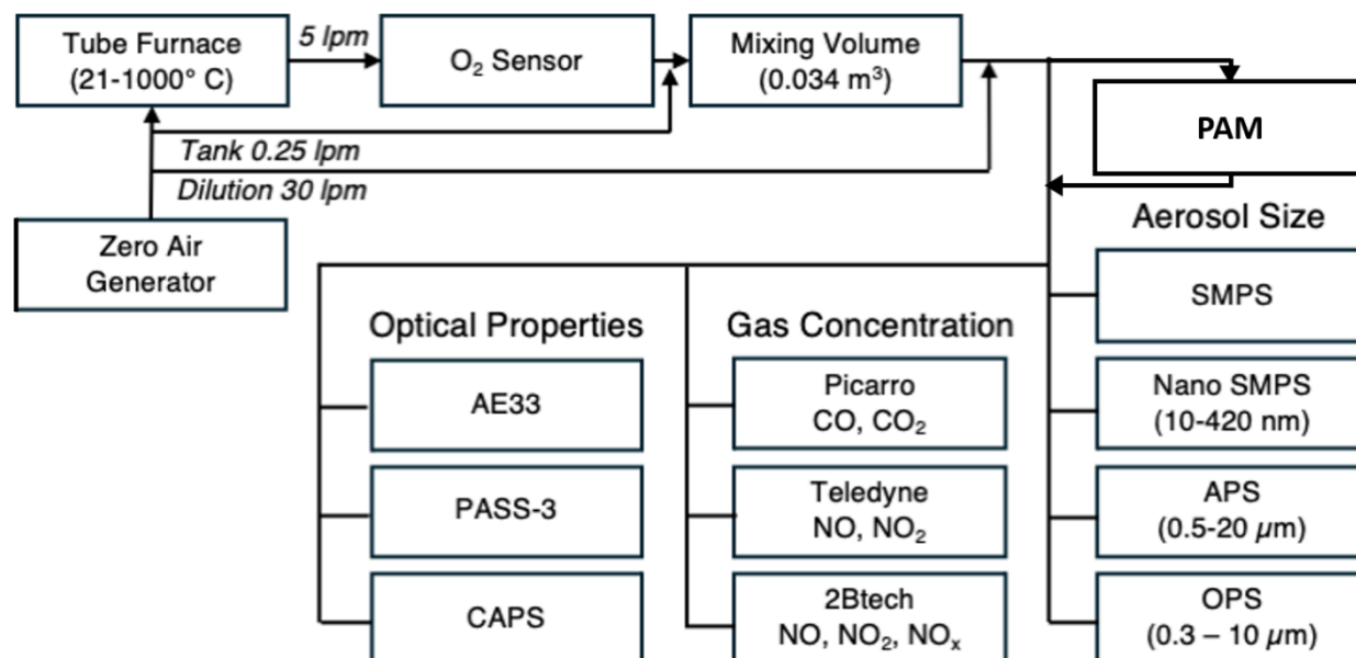
Figure 1. A diagram of the system at LANL used for generating and characterizing BB aerosol.
