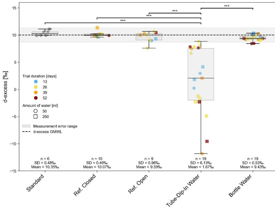
Figure 7: Deuterium excess from experiment 2 as an indicator of isotope fractionation on \text{H}_2\text{O} through different time steps within the evaporation experiment. Significant differences between groups, determined via Dunn's post-hoc test, are indicated by horizontal lines with corresponding significance levels p < 0.05 (*), p < 0.01 (**), p < 0.001 (***)
