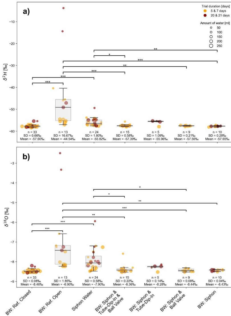
220 Figure 5: \delta^2\text{H} (a) and \delta^{18}\text{O} (b) isotopic signature [‰] from experiment 1, indicating isotope fractionation of \text{H}_2\text{O} over different time steps in the evaporation experiment. Significant differences between groups, determined via Dunn's post-hoc test, are indicated by horizontal lines with corresponding significance levels, p < 0.05 (*), p < 0.01 (**), p < 0.001 (***)).
