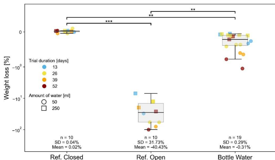
235 Figure 6: The relative weight difference between the start and end of experiment 2, expressed as a percentage on a logarithmic scale, was used as an indicator of evaporation. The exposure time ranged from 13 to 52 days. The initial water volumes in the 250 mL SCHOTT glass bottles varied between 50 and 250 mL. The tested evaporation barrier, the tube-dip-in system, is shown in relation to closed and open bottles serving as references. Significant differences between groups, determined via Dunn's post-hoc test, are indicated by horizontal lines with corresponding significance levels p < 0.05 (*), p < 0.01 (**), p < 0.001 (***)
