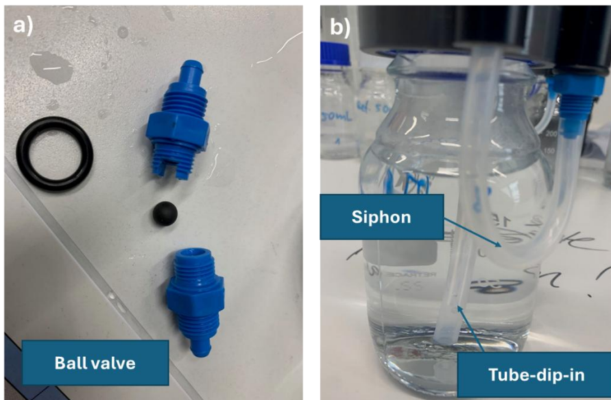
Figure 2: (a) Tested evaporation barriers: Ball-valve which is consisting of a floating plastic ball inside a cone sealed with an O-ring; (b) Siphon outside the bottle and a tube-dip-in, respectively, both are minimizing the atmospheric contact of the inflow.
