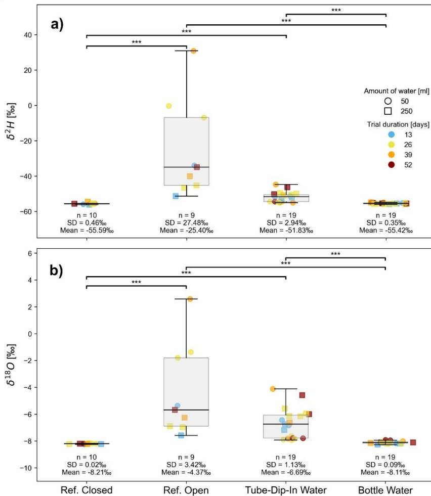
270 Figure 8: \delta^2\text{H} (a) and \delta^{18}\text{O} (b) isotopic signature [‰] from experiment 2 as an indicator of isotope fractionation on \text{H}_2\text{O} through different time steps within the evaporation experiment. Significant differences between groups, determined via Dunn's post-hoc test, are indicated by horizontal lines with corresponding significance levels p < 0.05 (*), p < 0.01 (**), p < 0.001 (***)
