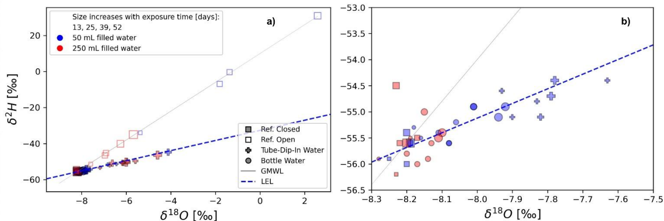
310 Figure 10: Dual water isotope plot showing isotope fractionation during experiment 2 using tube-dip-in as the evaporation barrier. Both diagrams (a and b) display the same results on different scales. Label sizes correspond to the exposure time, which varies between 13, 25, 39 or 52 days. Colors represent different water volumes (50 mL vs. 250 mL). The star labels indicate water samples from the tube-dip-in. The equation of the local evaporation line (LEL) is \delta^2\text{H} = 2.8 \cdot \delta^{18}\text{O} - 32.6 , R^2 = 0.52 , p\text{-value} < 0.001
