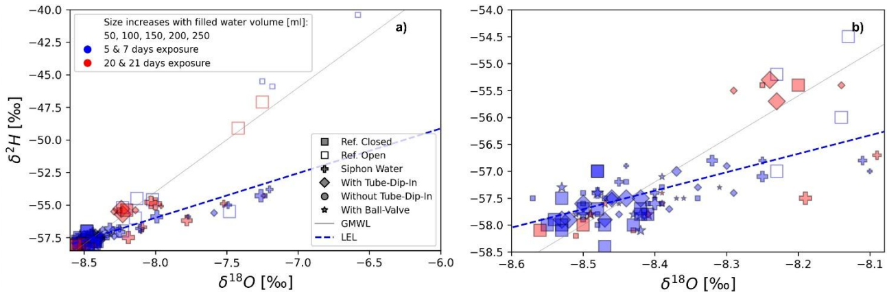
300 Figure 9: Dual water isotope plot showing isotope fractionation during experiment 1 using different evaporation barriers (siphon, ball valve, and tube-dip-in). Both diagrams (a and b) display the same results on different scales. The label sizes correspond to the filled water volume, which varies between 50, 100, 150, 200, or 250 mL. Colors represent different exposure times, with blue indicating short exposure and red indicating long exposure. The equation of the local evaporation line (LEL) is \delta^2\text{H} = 3.4 \cdot \delta^{18}\text{O} - 28.6 with R^2 = 0.52 and p\text{-value} < 0.001
