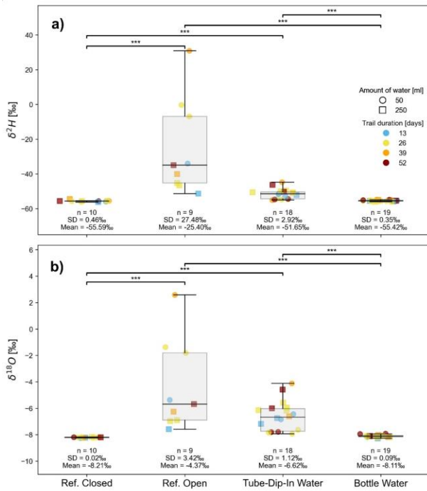
Figure 8: \delta^{2}H (a) and \delta^{18}O (b) isotopic signature [‰] from experiment 2 as an indicator of isotope fractionation on H_2O through different time steps within the evaporation experiment. Significant differences between groups, determined via Dunn's post-hoc test, are indicated by horizontal lines with corresponding significance levels p < 0.05 (*), p < 0.01 (**), p < 0.001 (***)
