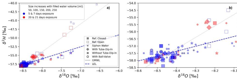
500 Figure 9: Dual water isotope plot showing isotope fractionation during experiment 1 using different evaporation barriers (siphon, ball valve, and tube-dip-in). Both diagrams (a and b) display the same results on different scales. The label sizes correspond to the filled water volume, which varies between 50, 100, 150, 200, or 250 mL. Colors represent different exposure times, with blue indicating short exposure and red indicating long exposure. The equation of the local evaporation line (LEL) is \delta^2\text{H} = 3.4 \cdot \delta^{18}\text{O} - 28.6 , with R^2 = 0.52 and p\text{-value} < 0.001 .
