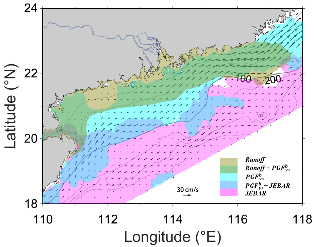
505 Figure 10. Schematic map of the regions controlled by different impact factors ( Runoff , PGF_{y*}^b and JEBAR ) during summer in the NSCS. The arrows depict the mean summer shelf circulation.
