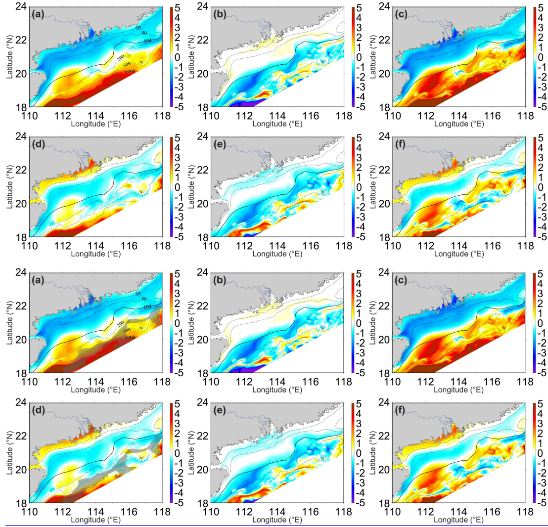
Figure 8. Regression maps of horizontal components ( \text{m}^2 \text{s}^{-2} ) in the JEBAR term during the summer of positive MVPC1 years, under different runoff conditions: (a–c) correspond to positive PC1 years, and (d–f) to negative PC1 years. Panels show (a, d) the full baroclinic gradient term ( \frac{g}{\rho_0} \int_{-H}^0 z(\rho - \bar{\rho}) dz ), (b, e) the contribution from
