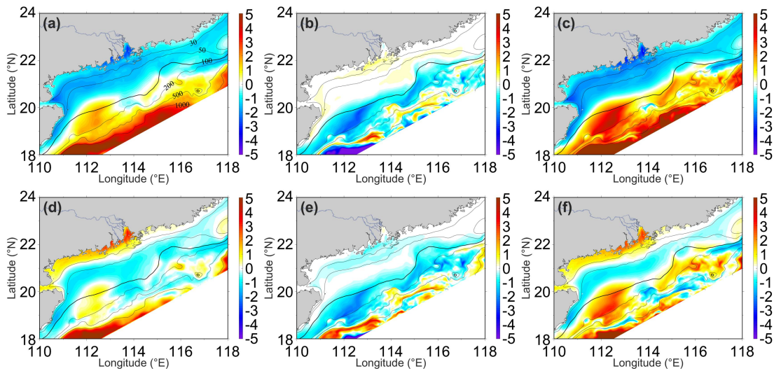
Figure 8. Regression maps of horizontal components ( \text{m}^2 \text{s}^{-2} ) in the JEBAR term during the summer of and
