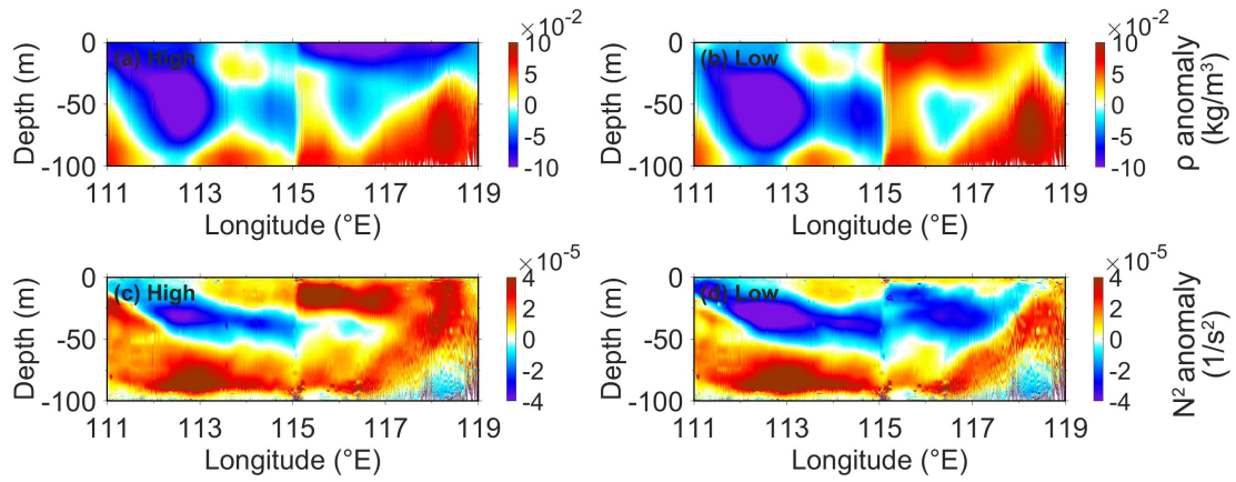
Figure A26. Regression maps of hydrographic anomaly profiles along the 100 m isobath during summer and negative MVPC1 years (Table 1), under different runoff conditions: (a, c) correspond to positive PC1 years, and (b, d) to negative PC1 years (Table 2). Panels show (a, b) density anomalies ( \text{kg m}^{-3} ) and (c, d) buoyancy frequency squared anomalies ( \text{s}^{-2} ). The two-stage regression approach is detailed in the section 3.2.
