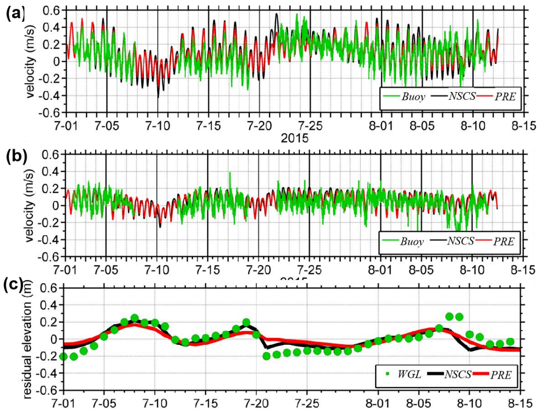
Figure A1. Time series of depth-averaged velocities—(a) zonal and (b) meridional—at the buoy/ADCP station, and (c) residual (de-tided) sea level at Waglan Island (WGL) during July–August 2015. Observations are shown in green, the NSCS simulation (this study) in black, and the PRE simulation from Liu et al. (2020) in red. Units: \text{m s}^{-1} for (a–b) and m for (c).
