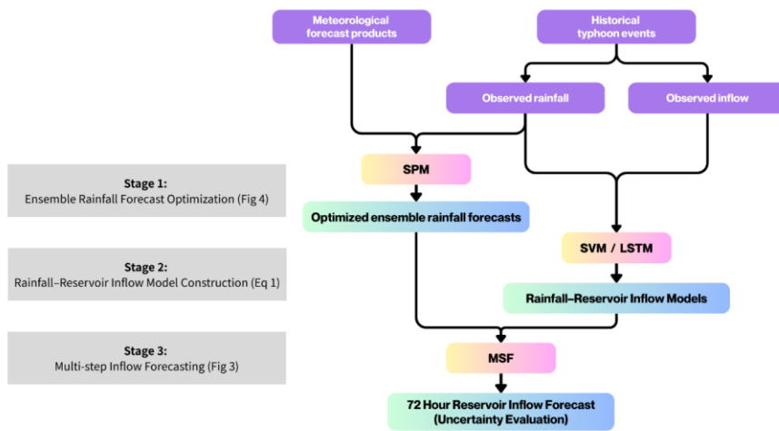
Figure 2 Schematic diagram of the proposed three-stage framework for 72-hour reservoir inflow forecasting, integrating ensemble rainfall forecasts with machine learning models (SVM and LSTM) via the Switch Prediction Method (SPM) and Multi-Step Forecasting (MSF).
