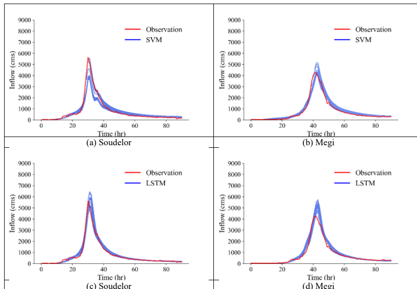
505 Figure 10 Multi-step inflow forecasts using observed rainfall for Typhoons Soudelor and Megi. The results validate both SVM and LSTM models for capturing temporal hydrological dynamics.
