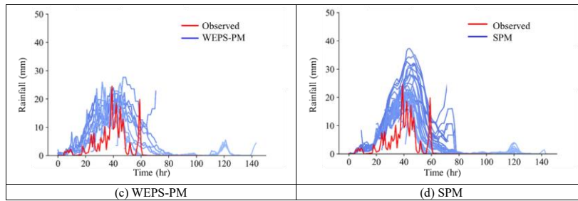
Figure 8 Comparison of meteorological forecast products (QPF, ETQPF and WEPS-PM) and the SPM-generated forecast for Typhoon Lekima.
