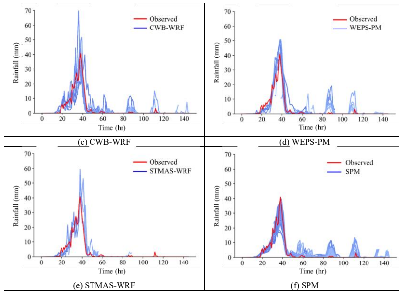
460 Figure 6 Comparison of meteorological forecast products (QPF, ETQPF, CWB-WRF, WEPS-PM and STMAS-WRF) and the SPM-generated forecast for Typhoon Megi.
