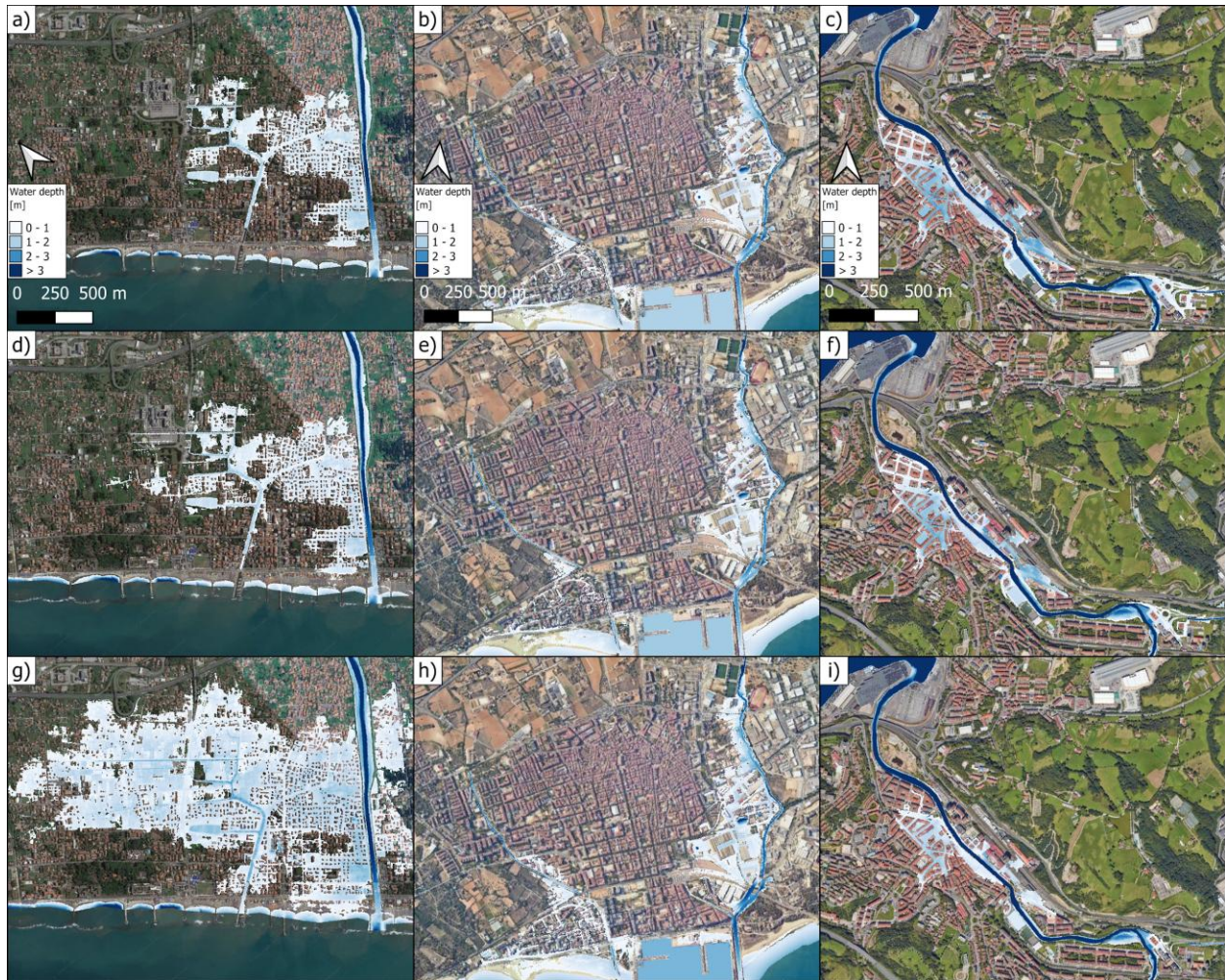
Fig S2 Hazard maps associated to the 100 years return period riverine flood event for the city of Massa: Historical a), RCP4.5 2011-2060 d), RCP8.5 2051-2100 g); for the city of Vilanova: Historical b), RCP4.5 2011-2060 e), RCP8.5 2051-2100 h); for the city of Oarsoaldea: Historical c), RCP4.5 2011-2060 f), RCP8.5 2051-2100 i). Base map: Google Satellite imagery (© Google 2024; Imagery © CNES / Airbus, Maxar Technologies, Airbus)
