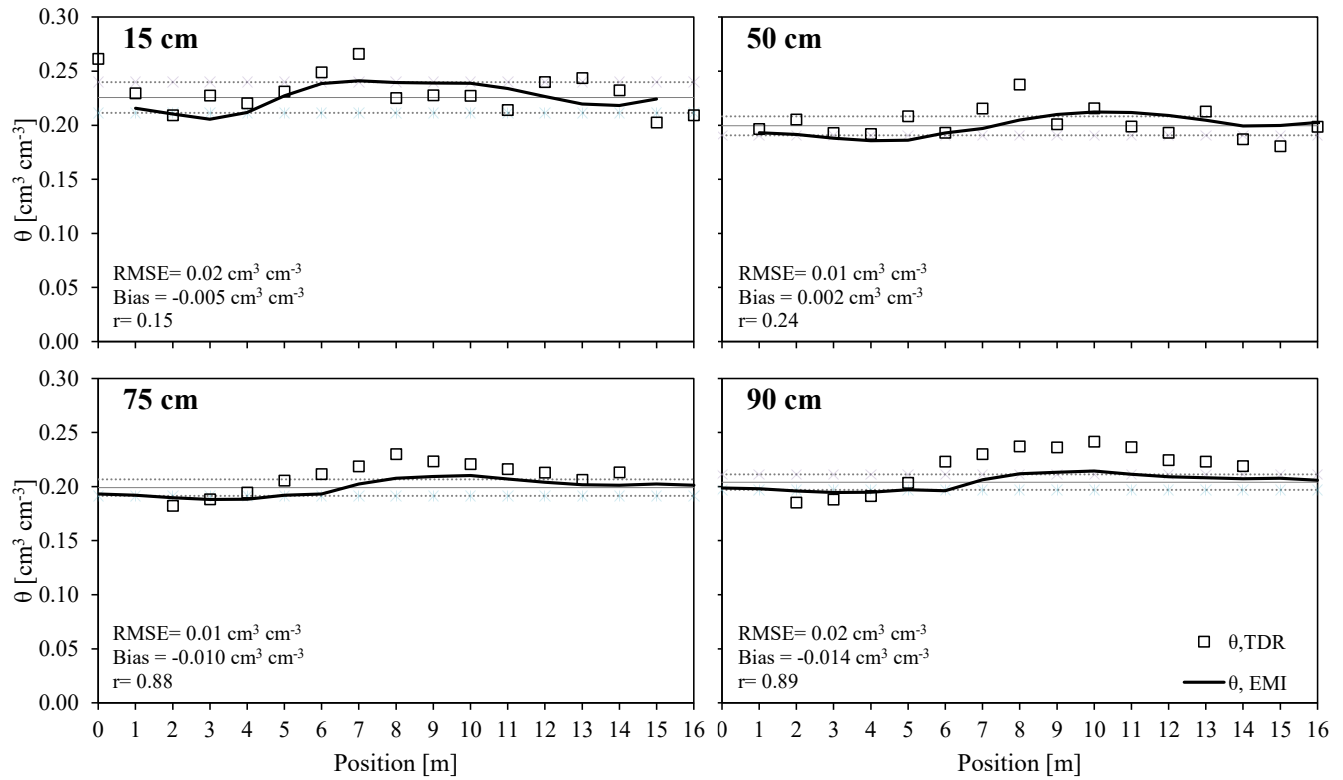
Figure 10: Spatial distribution of soil water content within the trench for four depths (15, 50, 75 and 90 cm) as measured by TDR ( \theta_{\text{TDR}} ) and estimated by EMI, ( \theta_{\text{EMI}} ) in the non-saline transect. The \theta_{\text{TDR}} data are represented by empty square. \theta_{\text{EMI}} data for each position are represented by a continuous thick solid line. Horizon-wise mean of \theta_{\text{EMI}} value is represented by a thin solid line while dashed lines represents the horizon-wise \theta_{\text{EMI}} mean \pm SD.
