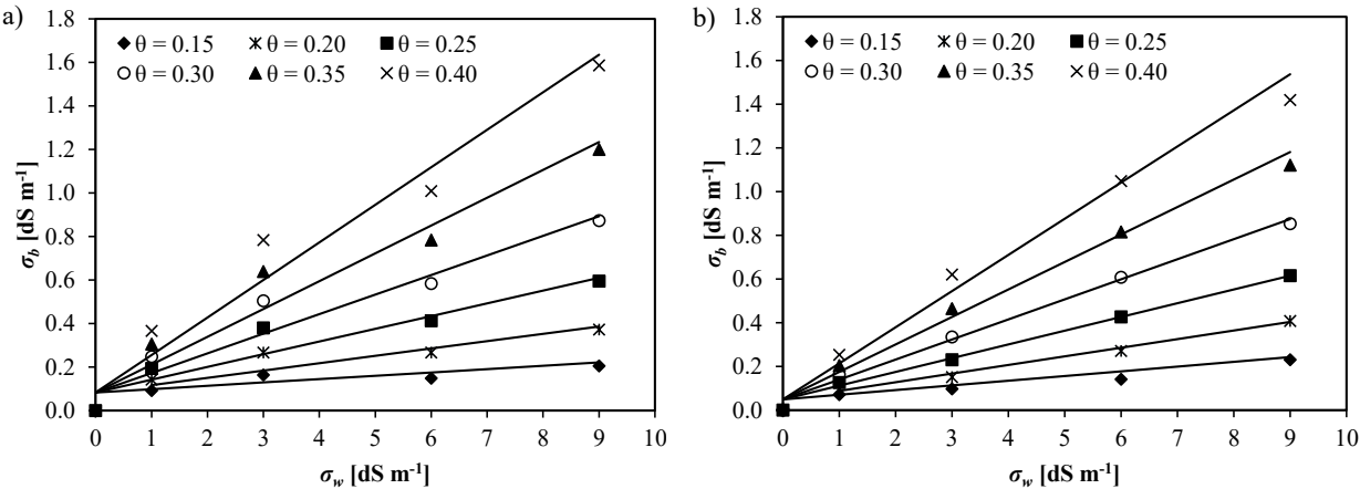
335 Figure 6: Bulk electrical conductivity ( \sigma_b ) measured by TDR vs. pore water electrical conductivity ( \sigma_w ) measured by an EC meter for six levels of soil water content ( \text{cm}^3 \text{ cm}^{-3} ). The continuous lines represent the fitted Rhoades model (Eqs. 1 and 2) for a) topsoil and b) subsoil.
