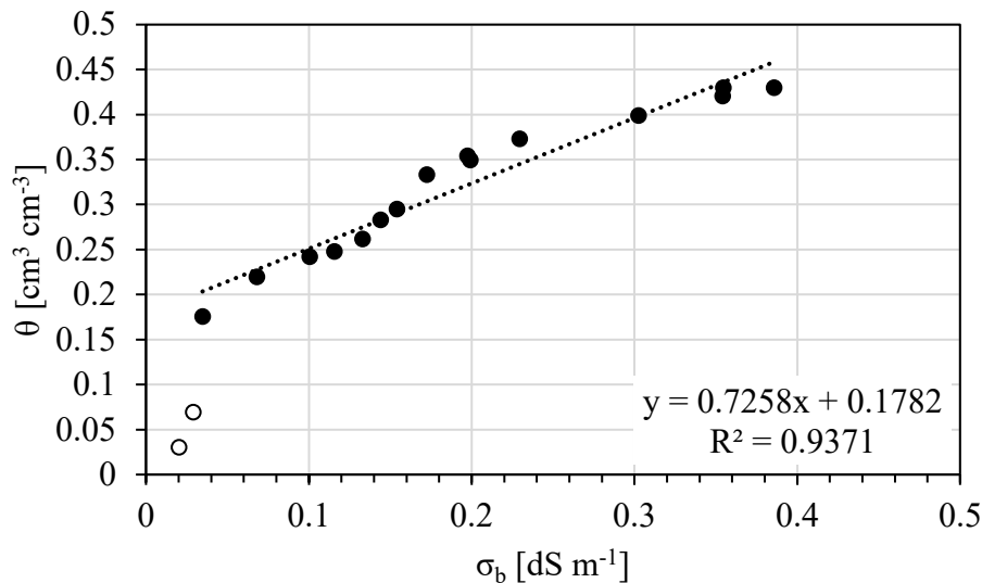
Figure 5: Soil specific linear relationship between the \sigma_b and volumetric soil water content for whole soil profile. The filled circle indicates the \theta – \sigma_b pairs from measured values, the dotted line represents the linear regression while the circles whit the white background are the pairs excluded from the calibration of the linear relationship.
