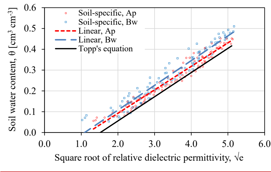
Figure 4: Soil specific linear relationship between the square root of relative dielectric permittivity and volumetric soil water content for the Ap and Bw horizons.
