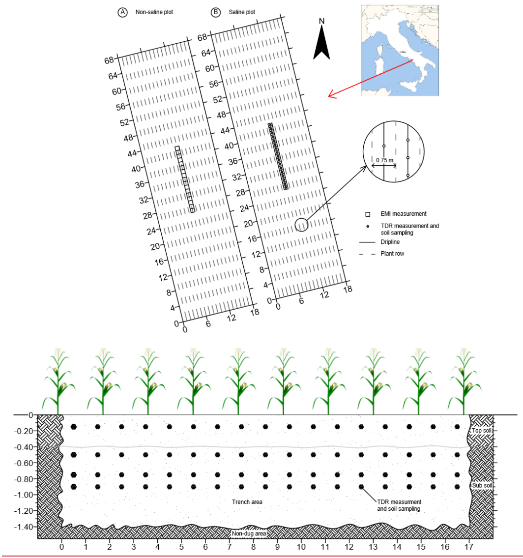
Figure 1: Schematic view of the experimental field (top panel) and front view of the trench showing measurement points (bottom panel). Map of Italy source:
