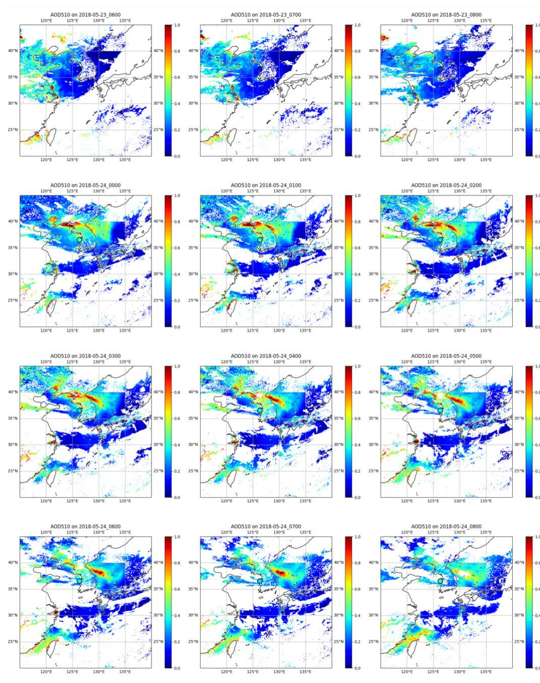
Figure 10: AHI/GRASP AOD510 nm distribution for the pollution event during 23 rd -24 th May, 2018. The AERONET site Anmyon (South Korea) is marked with a black circle.
