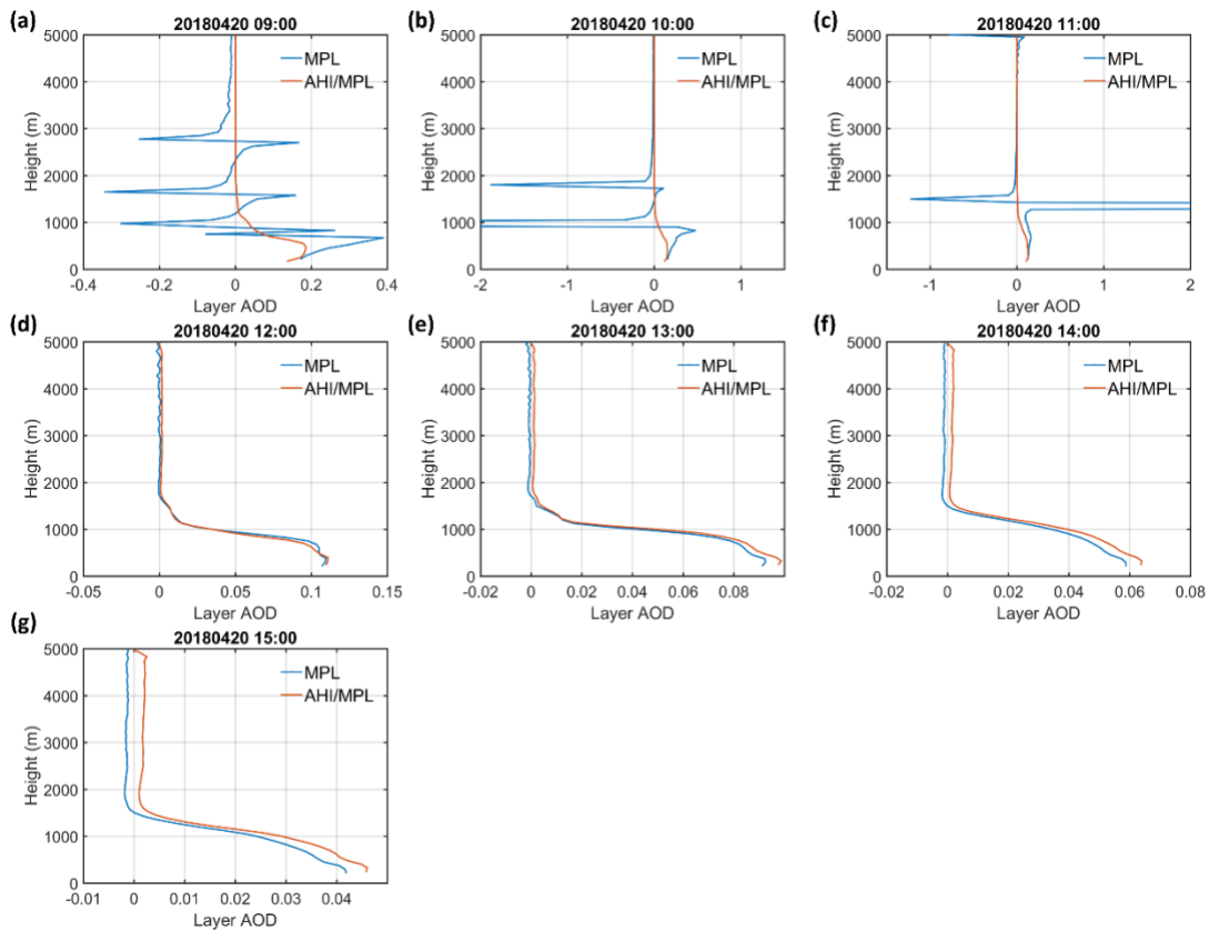
Figure 25: Same as Figure 23, but for 20 th April, 2018 (LST).
