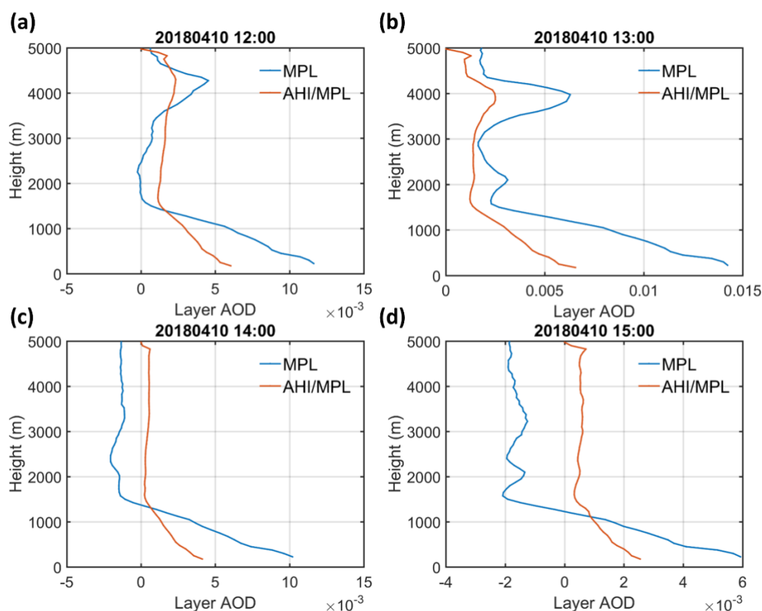
Figure 23: Aerosol vertical profiles retrieved from AHI+MPL/GRASP and Fernald method for 10 th April, 2018 (LST).
