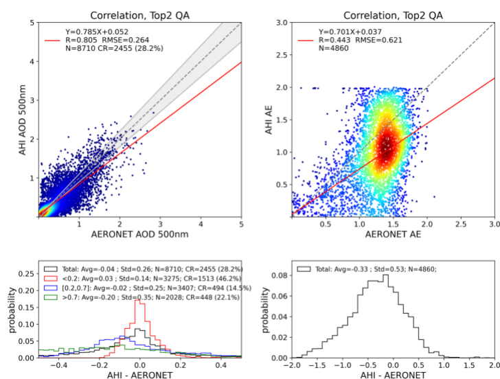
Figure 2: Validation of AHI/JAXA operational products against AERONET measurements for AOD at 500nm and Angstrom exponent (AHI at 400-600nm, AERONET at 440-870nm for the year 2018. The 1:1 reference lines and linear regression lines are indicated by grey dashed lines and red lines. The GCOS requirements for AOD: max (10%; 0.04) are indicated by the grey envelopes. The probability density functions of biases (AHI/JAXA–AERONET) are present in the lower panels for different AOD conditions: the black, red, blue and green solid lines represent all AOD, AOD < 0.2, 0.2 ≤ AOD ≤ 0.7 and AOD > 0.7, respectively.
