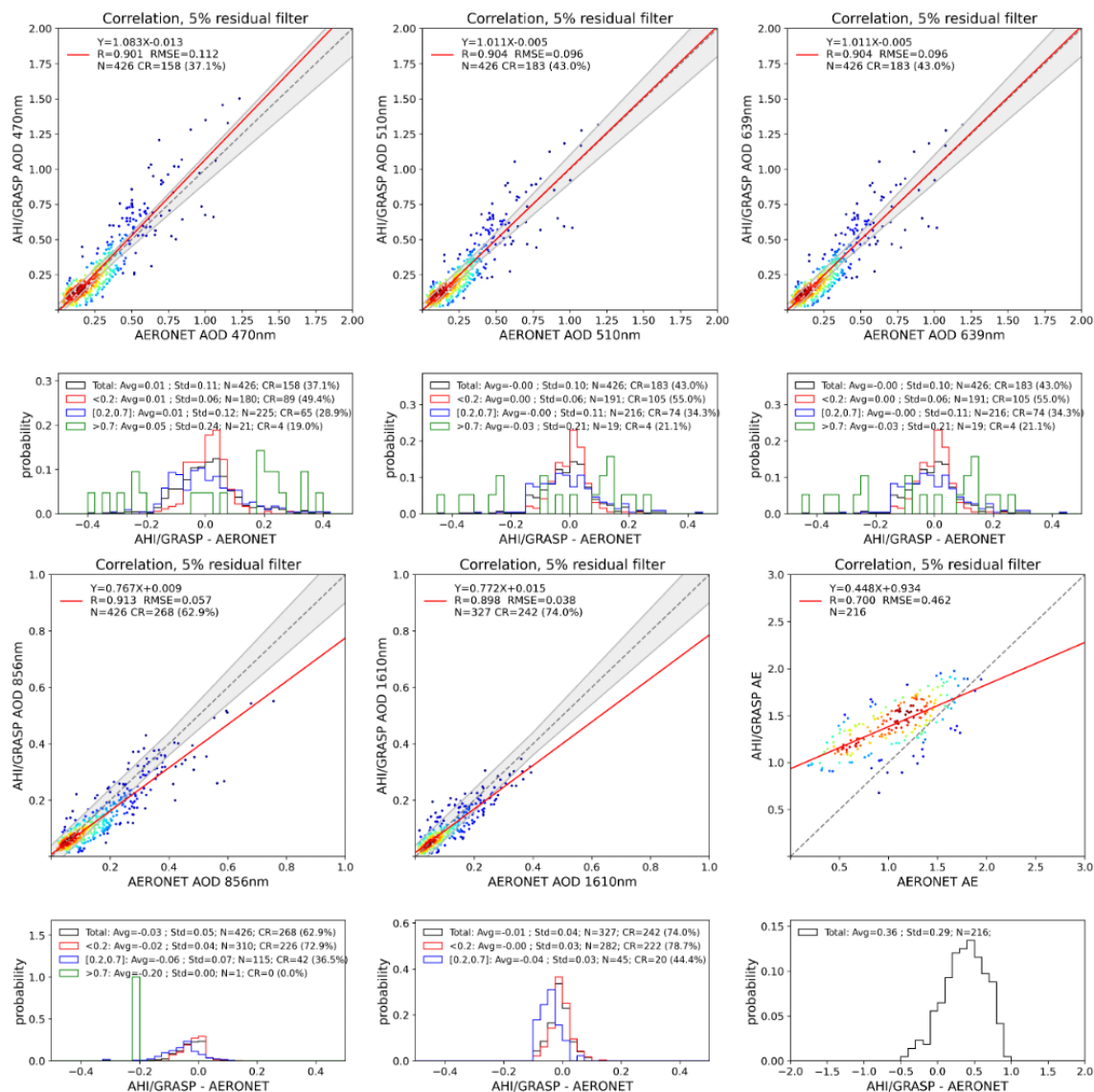
Figure 6: Same as Figure 3, but for over Ocean for May 2018.
