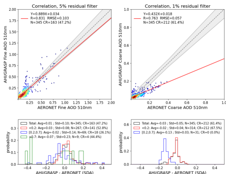
520 Figure 7: Same as Figure 5, but for over Ocean for May 2018.
