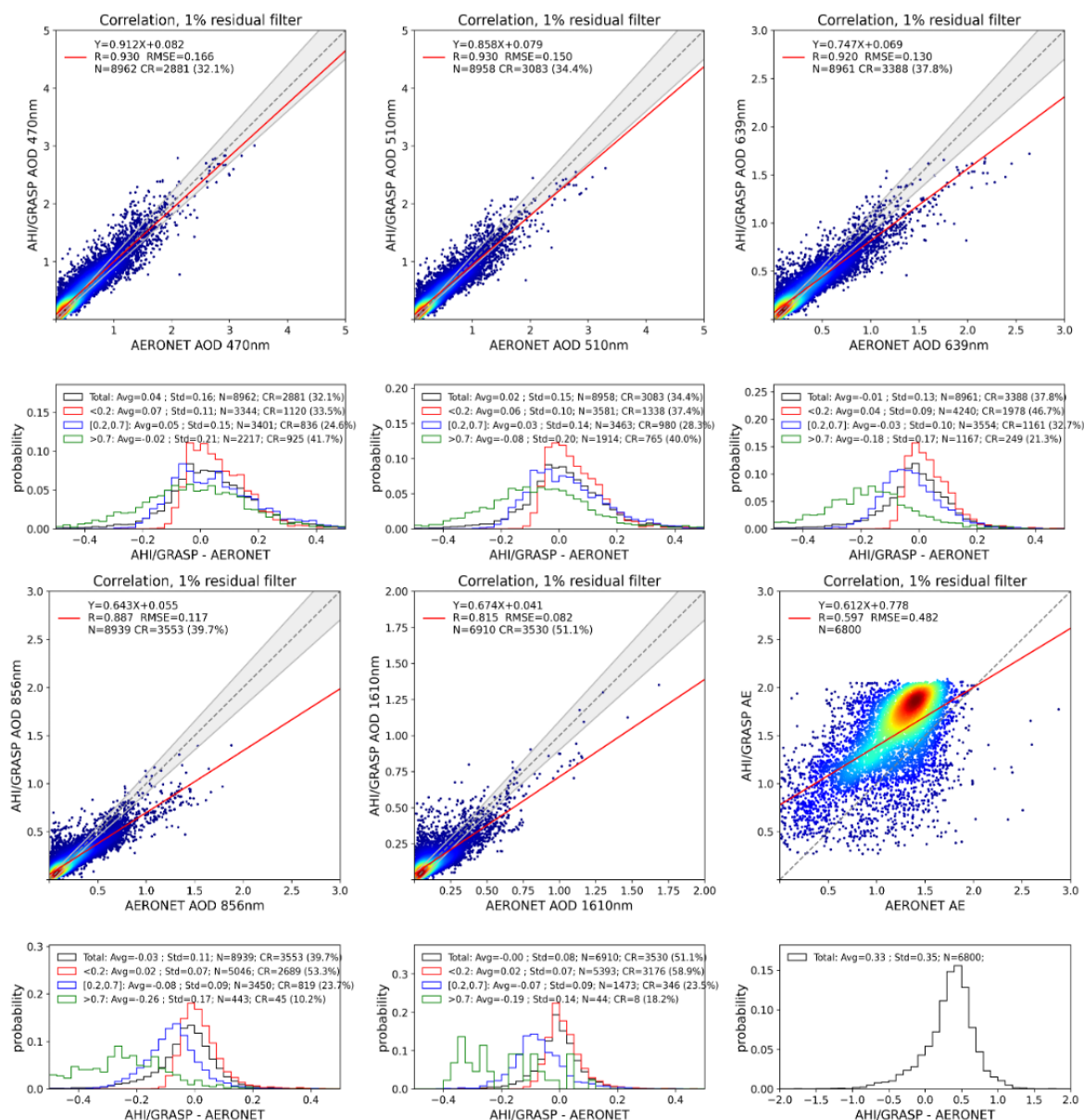
Figure 3: Validation of AHI/GRASP retrievals against AERONET measurements for AOD at 470nm, 510nm, 639nm, 856nm, 1610nm and Angstrom exponent at 470-856nm in 2018 over land. The AERONET AODs are interpolated using the Angstrom Exponent. The 1:1 reference lines and linear regression lines are indicated by grey dashed lines and red lines. The GCOS requirements for AOD: max (10%; 0.04) are indicated by the grey envelopes. The probability density functions of biases (AHI/GRASP–AERONET) are present in the lower panels for different AOD conditions: the black, red, blue and green solid lines represent all AOD, AOD < 0.2, 0.2 ≤ AOD ≤ 0.7 and AOD > 0.7, respectively.
