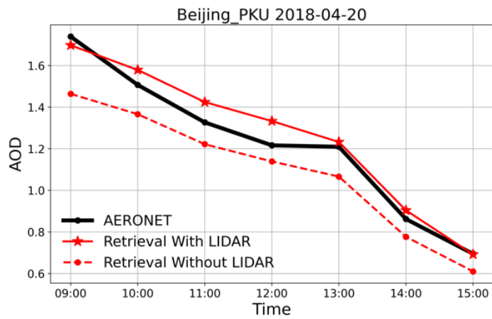
Figure 24: Same as Figure 22, but for 20 th April, 2018 (LST)
