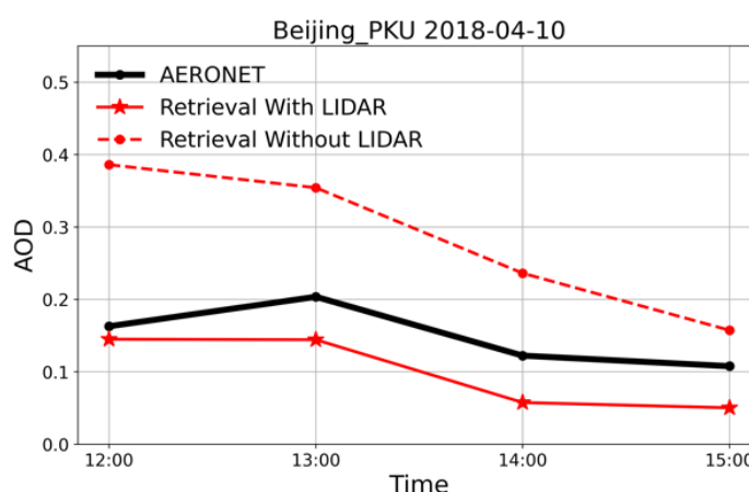
Figure 22: Diurnal cycles of AHI/GRASP (Red dashed line), AHI+MPL/GRASP (Red solid line) and AERONET AOD (Black solid line) for 10 th April, 2018 (LST).
