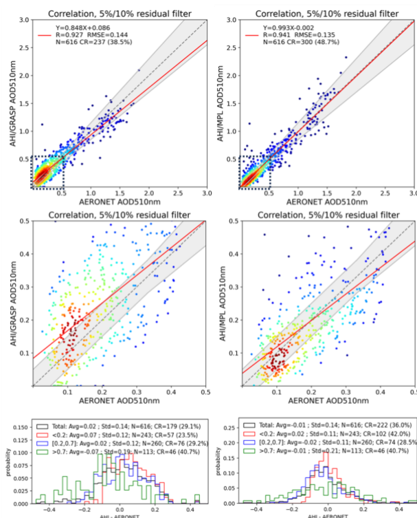
725 Figure 21: Validation of AHI/GRASP (left column) and AHI+MPL/GRASP (right column) retrievals against AERONET measurements at Beijing-PKU site for AOD at 510nm in 2018. The AERONET AODs are interpolated using the Angstrom Exponent. The middle panels show the zoom-in validations for low AOD conditions (AOD<0.5) and the bottom panels show the probability density functions of biases for different AOD conditions.
