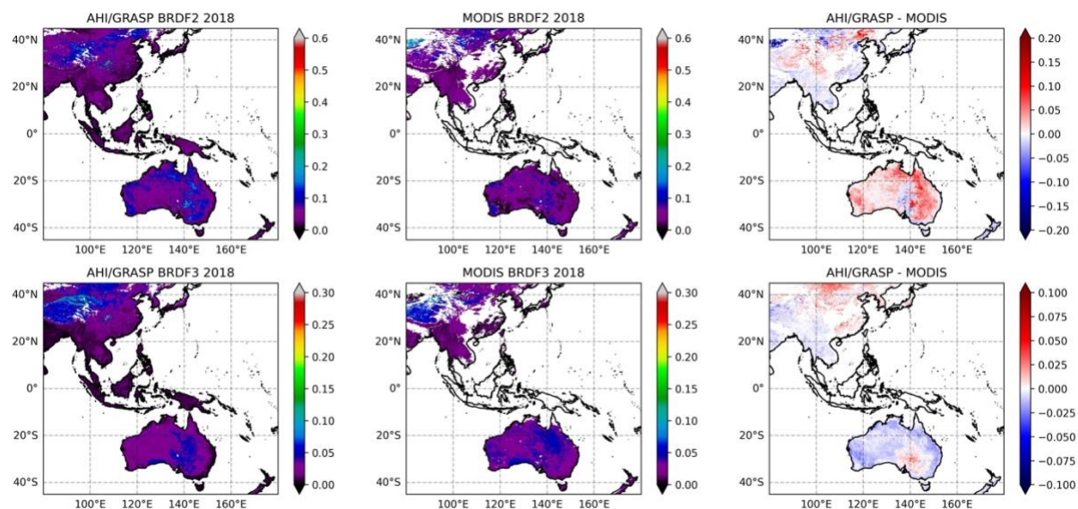
635 Figure 16: Same as Figure 6 but for Ross-LI BRDF2 and 3 (volumetric and geometric parameters) at 639 nm.
