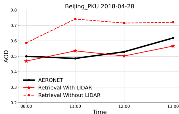
Figure 26: Same as Figure 22, but for 28 th April, 2018 (LST).
