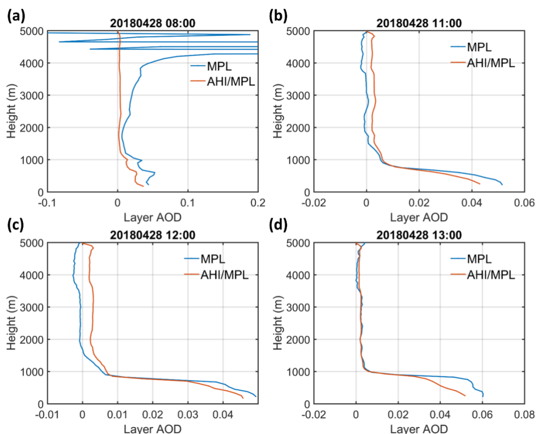
785 Figure 27: Same as Figure 23, but for 28 th April, 2018 (LST).
