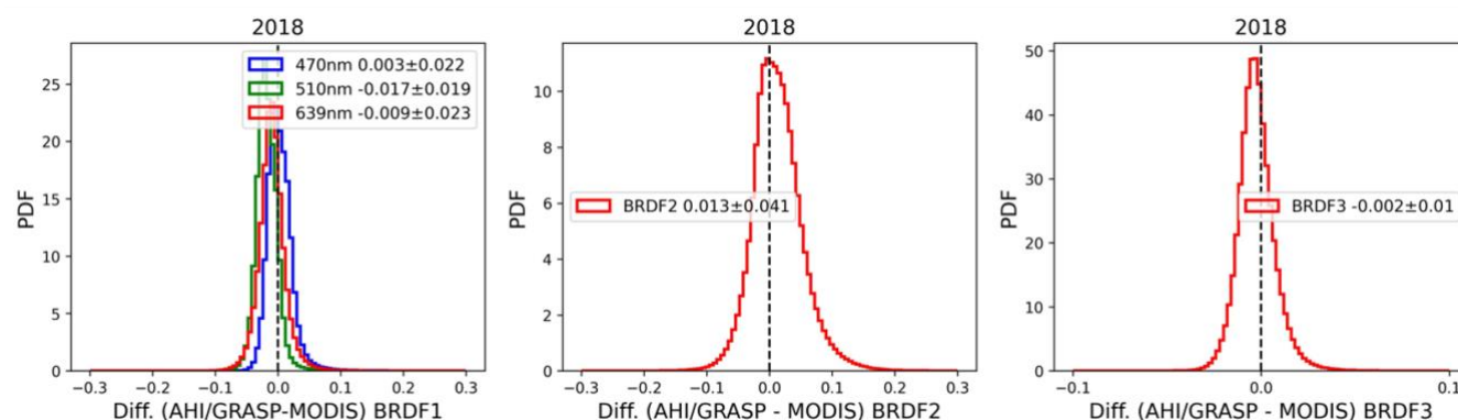
Figure 17: Comparison of AHI/GRASP daily average surface retrievals against MODIS MCD43C1 surface products for 1 st Ross-Li BRDF parameters at 470nm, 510nm and 639nm, and for 2 nd and 3 rd Ross-Li BRDF parameters (The parameters at 639nm are used). The MODIS BRDF parameters are linearly interpolated onto the AHI wavelengths.
