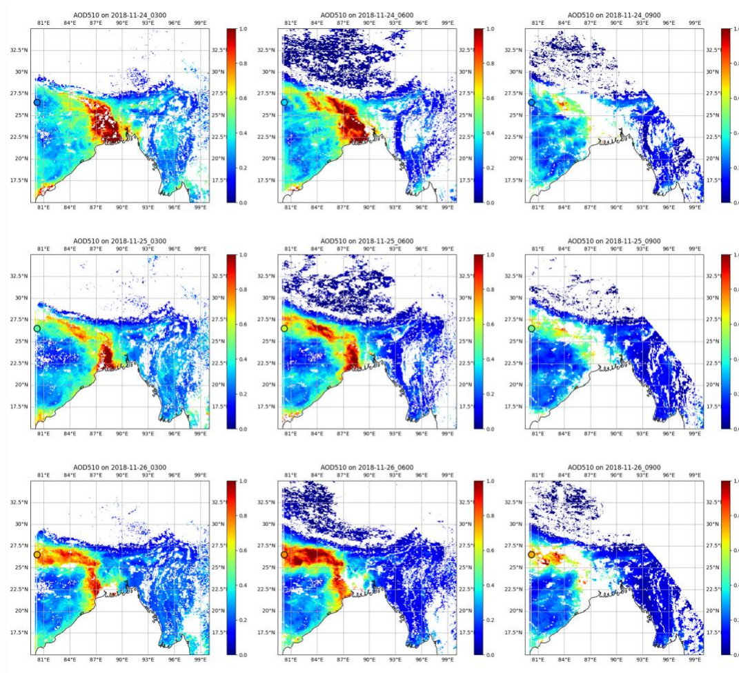
Figure 8: AHI/GRASP AOD510 nm distribution for the pollution event during 24 th – 26 th November, 2018. The AERONET site Kanpur (India) is marked with a black circle.
