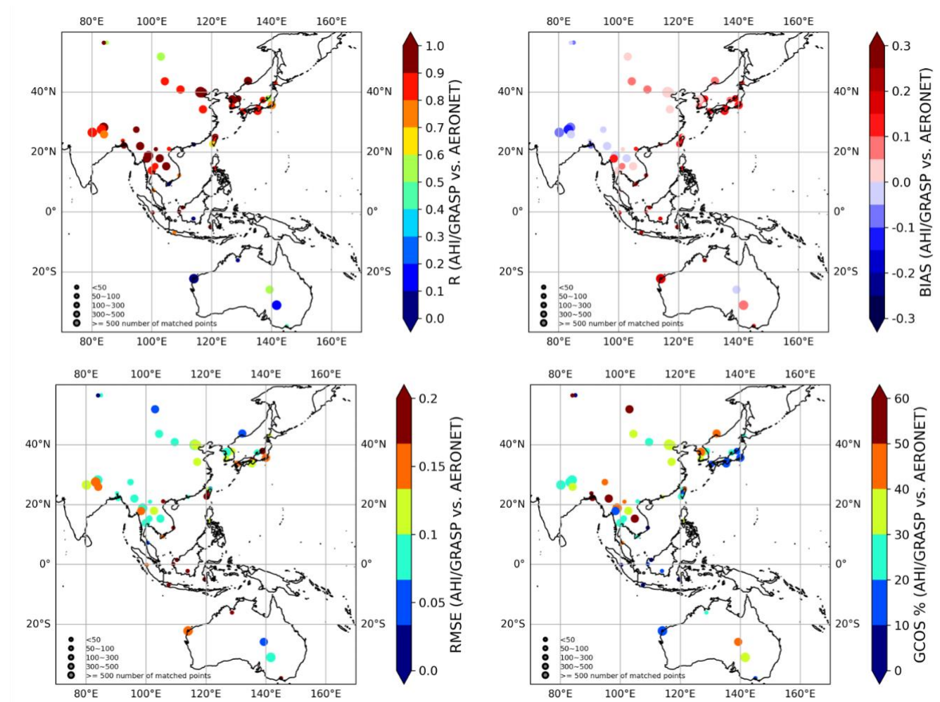
490 Figure 4: Maps of AHI/GRASP validation statistical metrics at AERONET over land stations for the year 2018 (a) R, (b) bias, (c) RMSE, (d) GCOS percentage (%) for AOD at 510nm.
