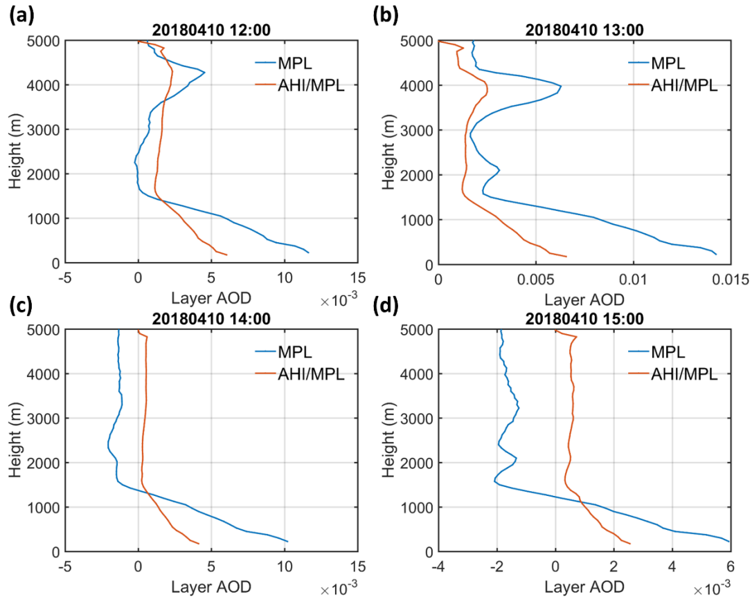
Figure 23: Aerosol vertical profiles retrieved from AHI+MPL/GRASP and Fernald method for 10 th April, 2018 (LST).
