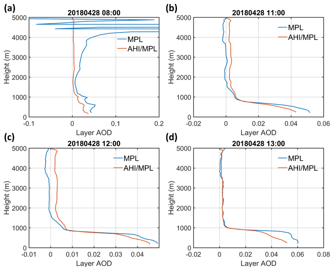
825 Figure 25: Aerosol vertical profiles retrieved from AHI+MPL/GRASP and Fernald method for 28 th April, 2018 (LST).
