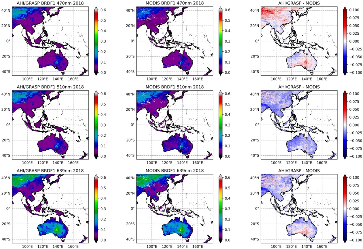
Figure 15: Spatial distribution of yearly (2018) Ross-LI BRDF1 (isotropic parameter) from AHI/GRASP, MODIS MCD43C1 and their differences at 470, 510 and 639nm.
