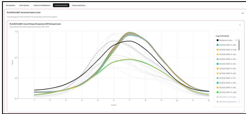
(a) Within the REF Data Explorer for Land and Land Ice, the gross primary production (GPP) annual cycle can be explored, and here, the CanESM5-1 model ensembles (above the black Reference line) and ACCESS-ESM1-5 model ensembles (below the black Reference line) are highlighted in color.
