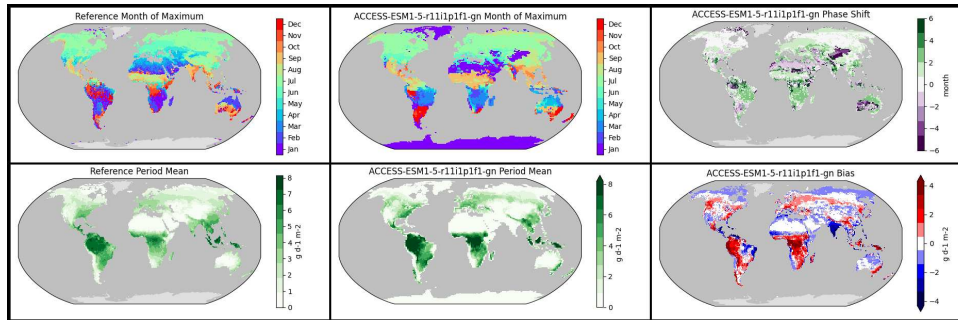
(c) Within the REF Diagnostics for Land and Land Ice, the month of maximum GPP (i.e., the phase of the annual cycle) is shown spatially (top row) for the Reference (first column), the ACCESS-ESM1-5 model ensemble (second column), and the difference between the model ensemble and Reference (third column). Similarly, the spatial distribution of the annual integrated GPP from the ACCESS-ESM1-5 model ensemble (second column) is compared to the Reference (first column) and the resulting bias (third column) in the bottom row.
