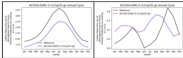
(b) Within the REF Diagnostics for Land and Land Ice, the GPP annual cycles for global land (left) and tropical land only (right) regions for a single ensemble member from the ACCESS-ESM1-5 model are displayed.
