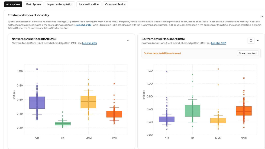
(a) Spatial RMSE of the simulated vs. observed leading Empirical Orthogonal Function (EOF1) describing the spatial pattern of the Northern and Southern Annular Modes for a large number of historical GCM runs obtained from CMIP6
