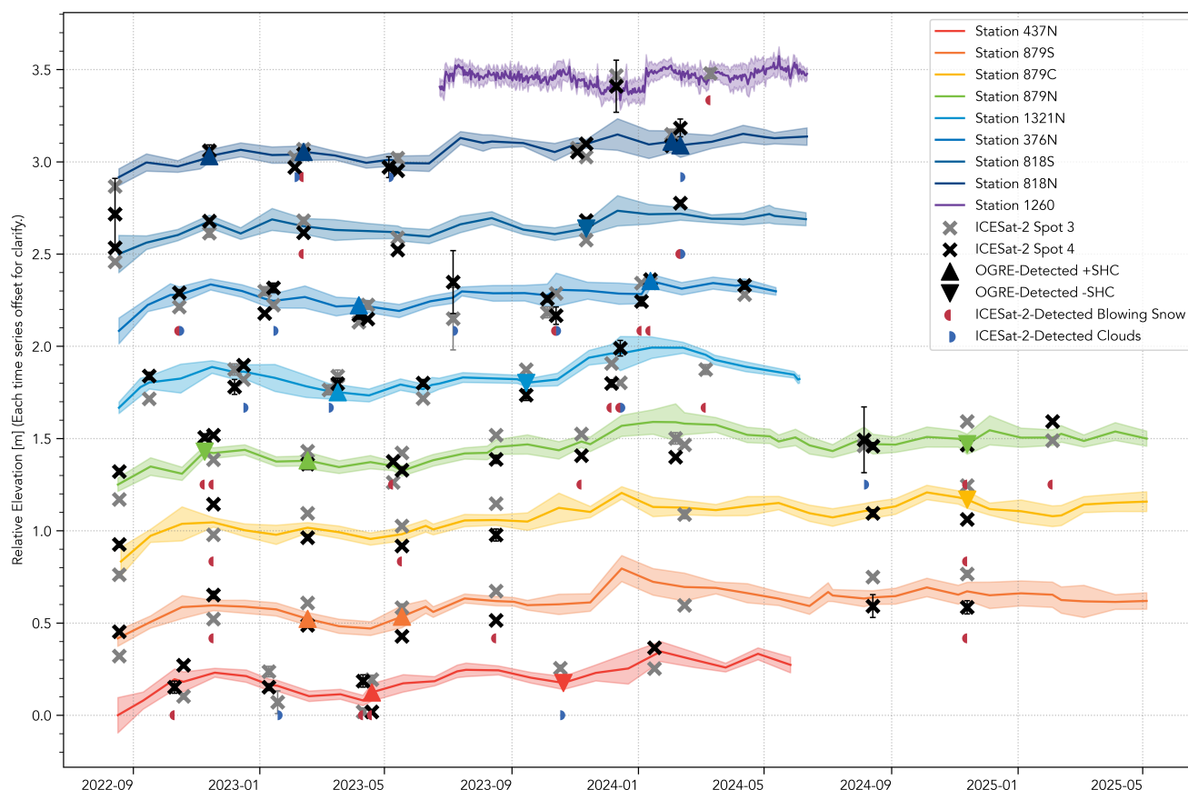
Figure 4. Time series of OGRE surface elevations compared to adjacent ATL06 surface elevations. Each OGRE time series is vertically offset by +0.4 m for clarify and annotated to indicate periods of active positive or negative surface height change (SHC) corresponding to ICESat-2 overflights. The 1- \sigma shaded regions surrounding each OGRE time series represent the spread in H_r estimates, which are influenced in part by surface roughness. Elevations and uncertainties are derived from monthly or bi-monthly estimates (or daily estimates for Station 1260), but are connected with lines for visual continuity. ICESat-2 elevations falling within each hemispherical footprint of each OGRE station are averaged together, and the error bars are taken to be the spread in these data, or in the case of only a single elevation, the ATL06 estimated error of that point. Each overpass is annotated with a marker when blowing snow or clouds were detected.
