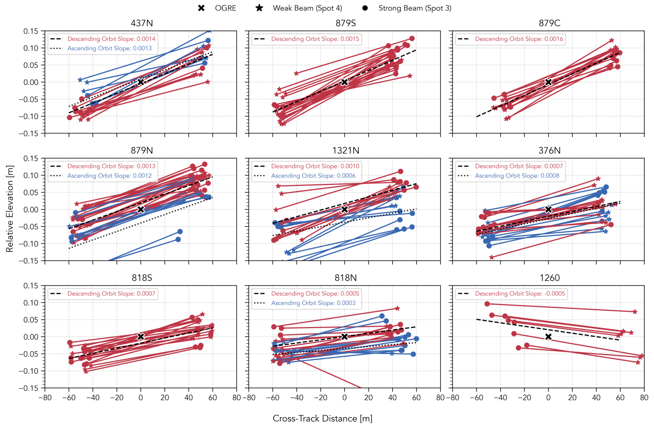
Figure 3. ICESat-2 beam pair elevations relative to OGRE-derived surface elevations. Any beam pair found within the 60 m search radius of the OGRE is plotted and colored by the orbit direction. The end-cap markers are stars for the weak beam spot and circles for the strong beam, which indicate the satellite's yaw configuration.
