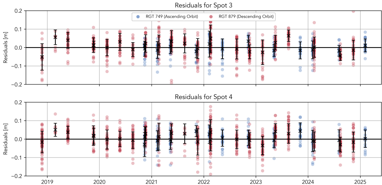
Figure 2. Spot 3 and Spot 4 residuals relative to kinematic GPS data. Residuals derived from descending overflight comparisons are in red, and residuals derived from ascending comparisons are in blue. We also show the median residual between the GPS survey and ICESat-2 ATL06 heights for each overflight in black, with the vertical bars indicating uncertainties expressed as the standard deviation of the residuals from that day.
