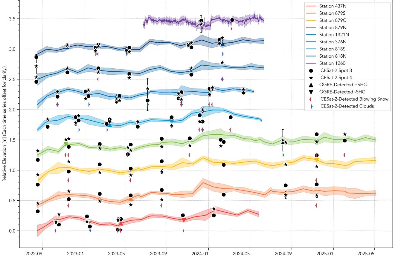
Figure 4. Time series of OGRE surface elevations compared to adjacent ATL06 surface elevations. Each OGRE time series is vertically offset by +0.4 m for clarity and annotated to indicate periods of active positive or negative surface height change (SHC) corresponding to ICESat-2 overpasses. The 1\sigma shaded regions surrounding each OGRE time series represent the spread in H_R estimates, which are influenced in part by surface roughness. Elevations and uncertainties are derived from monthly or semimonthly estimates (or daily estimates for Station 1260), but are connected with lines for visual continuity. ICESat-2 elevations falling within each hemispherical footprint of each OGRE station are averaged together, and the error bars are taken to be the spread in these data, or in the case of only a single elevation, the ATL06 estimated error of that point. Each overpass is annotated with a marker when blowing snow or clouds were detected.
