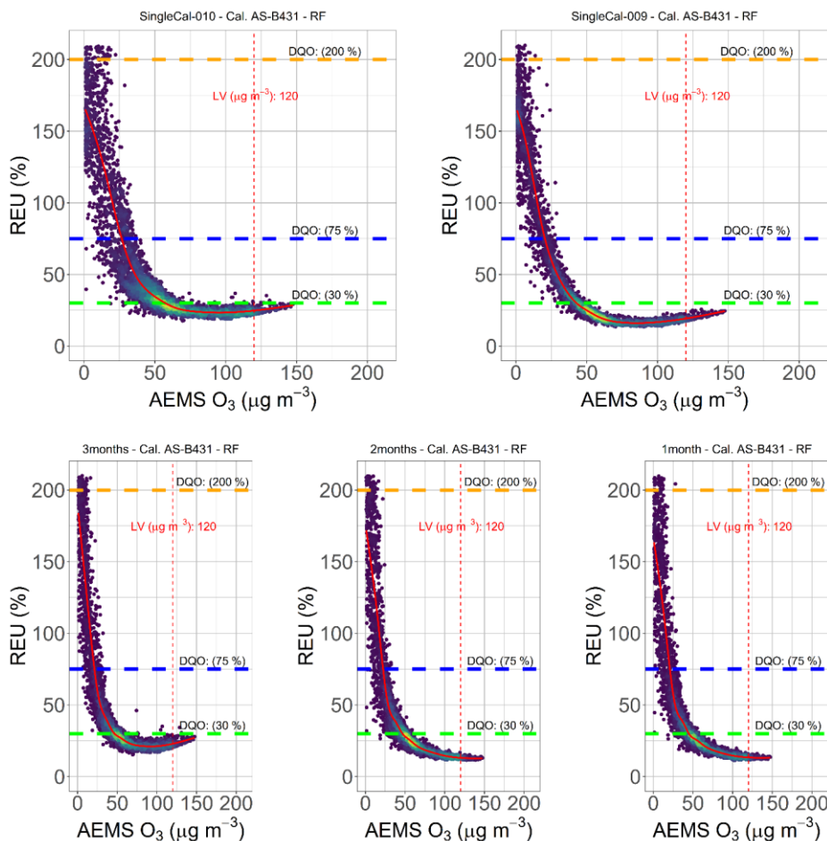
Figure 10. Calculated REU values for RF calibrated O 3 LCS hourly data belonging to the TP s (TP1–TP7, 10 June 2022–11 January 2023) of AELCM009 and AELCM010. The calibration variants are ST s (top row, left: AELCM010, right: AELCM009) and ET s (bottom row). The ET s is characterized by ET variants of 1, 2 and 3 months for each AELCM box. Horizontal dashed lines describe the DQOs (O 3 Class 1 DQO = 30 %, Class 2 DQO = 75 % and Class 3 DQO = 200 %). The vertical dashed line describes the limit value for O 3 (LV = 120 μg m -3 ). The fitted smooth curve (red) is based on a generalized additive model (GAM). Data density is shown through colour, where darker colours express lower data density and brighter colours express higher data density.
