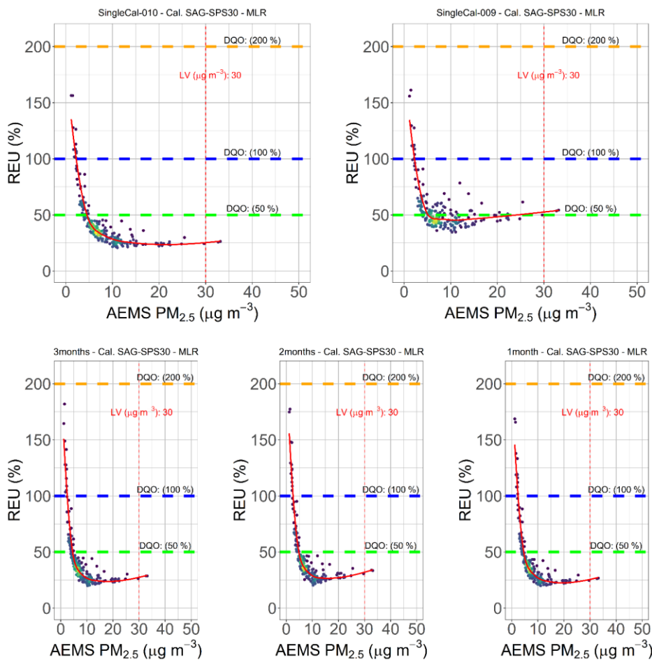
1280 Figure 1L. Calculated REU values for MLR calibrated PM_{2.5} LCS daily data belonging to the TP_s (TP1–TP7, 11 June 2022–6 January 2023) of AELCM009 and AELCM010. The calibration variants are ST_s (top row, left: AELCM010, right: AELCM009) and ET_s (bottom row). The ET_s is characterized by ET variants of 1, 2 and 3 months for each AELCM box. Horizontal dashed lines describe the DQO_s ( PM_{2.5} Class 1 DQO = 50\% , Class 2 DQO = 100\% and Class 3 DQO = 200\% ). The vertical dashed line describes the limit value for PM_{2.5} ( LV = 30\ \mu g\ m^{-3} ). The fitted smooth curve (red) is based on locally estimated scatterplot smoothing (LOESS). Data density is shown through colour, where darker colours express lower data density and brighter colours express higher data density.
