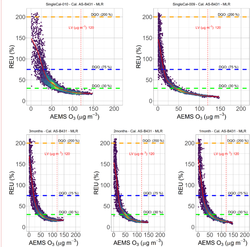
Figure 9. Calculated REU values for MLR calibrated O 3 LCS hourly data belonging to the TPs (TP1–TP7, 10 June 2022–11 January 2023) of AELCM009 and AELCM010. The calibration variants are ST 1 (top row, left: AELCM010, right: AELCM009) and ET 1 (bottom row). The ET 1 is characterized by ET variants of 1, 2 and 3 months for each AELCM box. Horizontal dashed lines describe the DQOs (O 3 Class 1 DQO = 30 %, Class 2 DQO = 75 % and Class 3 DQO = 200 %). The vertical dashed line describes the limit value for O 3 (LV = 120 µg m -3 ). The fitted smooth curve (red) is based on a generalized additive model (GAM). Data density is shown through colour, where darker colours express lower data density and brighter colours express higher data density.
