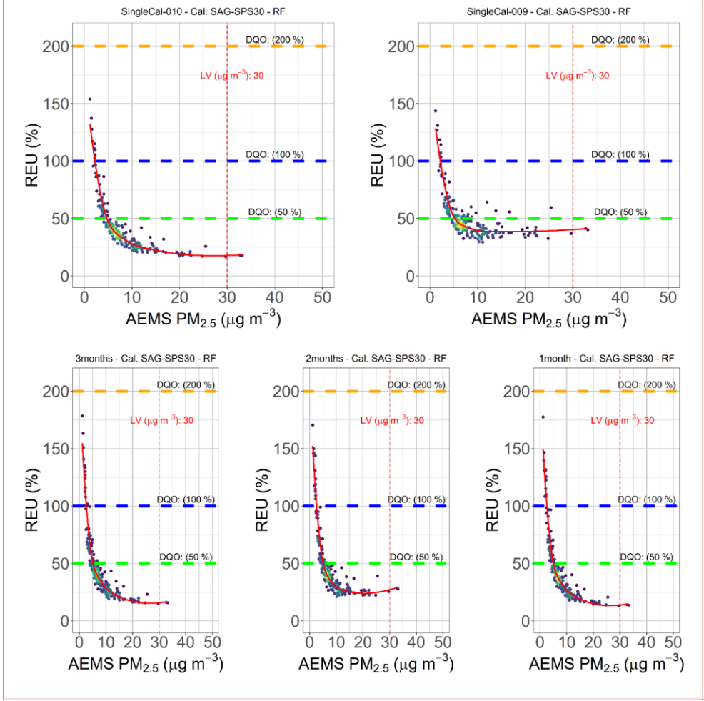
Figure 12. Calculated REU values for RF calibrated PM 2.5 LCS daily data belonging to the TP s (TP1–TP7, 11 June 2022–6 January 2023) of AELCM009 and AELCM010. The calibration variants are ST s (top row, left: AELCM010, right: AELCM009) and ET s (bottom row). The ET s is characterized by ET variants of 1, 2 and 3 months for each AELCM box. Horizontal dashed lines describe the DQO s (PM 2.5 Class 1 DQO = 50 %, Class 2 DQO = 100 % and Class 3 DQO = 200 %). The vertical dashed line describes the limit value for PM 2.5 (LV = 30 µg m -3 ). The fitted smooth curve (red) is based on locally estimated scatterplot smoothing (LOESS). Data density is shown through colour, where darker colours express lower data density and brighter colours express higher data density.
