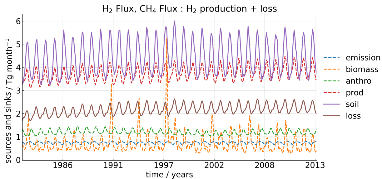
Figure A2. Globally averaged monthly hydrogen sources and sinks from 1982 – 2013. ‘emission’ refers to the natural hydrogen emissions both from the ocean and land. ‘prod’ and ‘loss’ refers to the atmospheric chemical production and loss of H 2 respectively.
