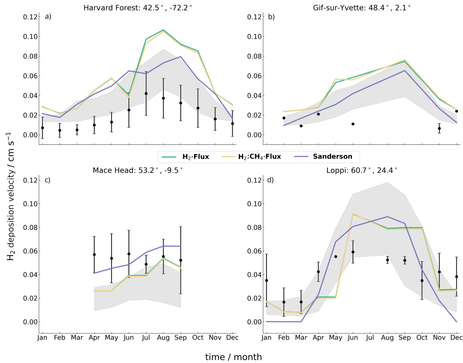
Figure 3. Monthly mean observed hydrogen deposition velocities averaged across years where possible (points) compared with (green) TR-H 2 -flux, (yellow) TR-H 2 CH 4 -flux, and (purple) Sanderson simulated velocities for a) Harvard Forest (2010 – 2012; Meredith et al., 2017), b) Gif-sur-Yvette (2011; Belviso et al., 2013), c) Mace Head (1995 – 2008; Simmonds et al., 2011), and d) Loppi (2004 – 2006; Lallo et al., 2008). Error bars show one standard deviation across years. Shaded areas show the range of deposition velocities from CMIP6 model inputs calculated in Brown et al. (2025).
