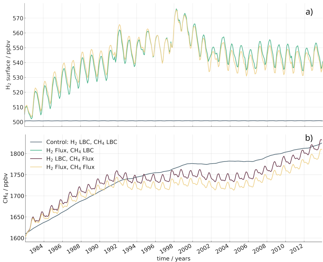
Figure 7. a) Globally averaged surface hydrogen from the (grey) control, (green) TR- H_2 -flux, and (yellow) TR- H_2CH_4 -flux simulations from 1982 to 2013. Both the control and the TR- CH_4 -flux simulation have hydrogen set to 500 ppbv at the surface. b) Globally averaged surface methane from the (grey) control, (red) TR- CH_4 -flux, and (yellow) TR- H_2CH_4 -flux simulations
