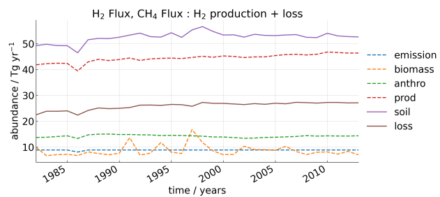
Figure A2. Globally averaged hydrogen sources and sinks from 1982 – 2013. ‘emissions’ refers to the natural hydrogen emissions both from the ocean and land. ‘prod’ and ‘loss’ refers to the atmospheric chemical production and loss of H 2 respectively.
