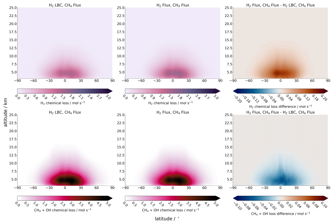
Figure A3. Zonally averaged (top) \text{H}_2 chemical loss and (bottom) \text{CH}_4 loss via OH for (left) TR- \text{CH}_4 -flux simulation, (middle) TR- \text{H}_2\text{CH}_4 -flux simulation, and (right) difference between the two ( \text{CH}_4 -flux – TR- \text{H}_2\text{CH}_4 -flux) averaged between 2008 – 2013. Red (blue) shows an increase (decrease) from the TR- \text{CH}_4 -flux. Note the non-linearity of scales.
