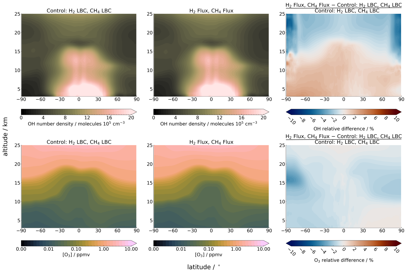
Figure 6. Zonally averaged (top) OH concentration and (bottom) ozone mixing ratio for the (left) control simulation, (middle) TR-H 2 CH 4 -flux simulation, and (right) the relative difference between the two ((TR-H 2 CH 4 -flux - Control)/Control) averaged between 2008 - 2013. Red (blue) shows an increase (decrease) from the control.
