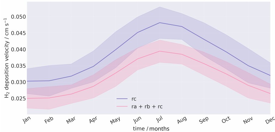
Figure 1. Monthly, land averaged hydrogen deposition velocity for simulation TR-H 2 -flux (H 2 Flux; CH 4 LBC) between 1982-2013 with all resistances (pink) and with only hydrogen deposition velocity (purple). Shaded areas indicate two standard deviations.
