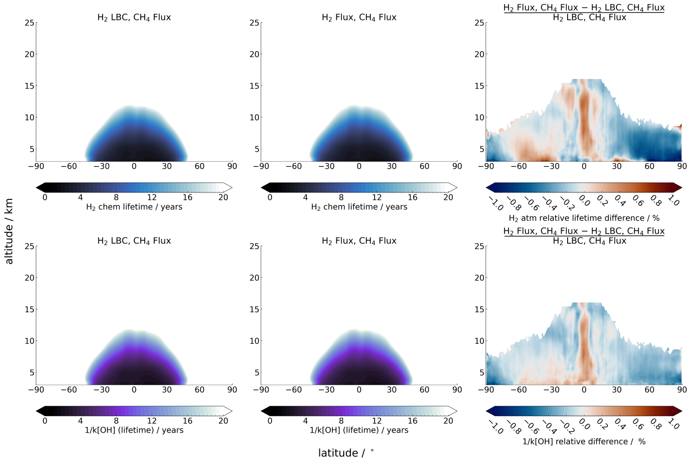
Figure 8. Zonally averaged (top) H 2 chemical loss lifetime and (bottom) CH 4 lifetime via OH for (left) TR-CH 4 -flux simulation, (middle) TR-H 2 CH 4 -flux simulation, and (right) relative difference between the two (CH 4 -flux – TR-H 2 CH 4 -flux) averaged between 2008 – 2013. Red (blue) shows an increase (decrease) in lifetimes from the TR-CH 4 -flux. The stratosphere has been masked out to reduce noise.
