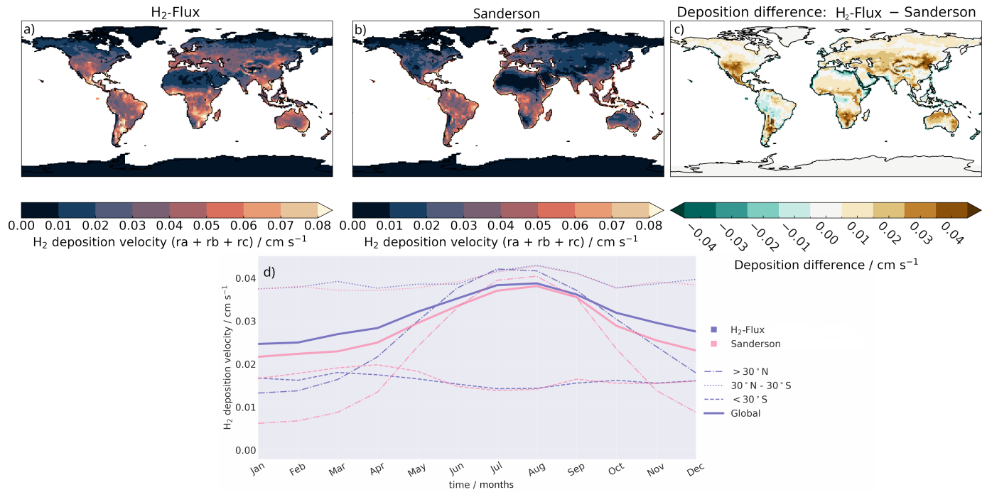
Figure 2. Annually averaged hydrogen deposition velocity in 1982 for a) TR-H 2 -flux using deposition scheme adapted from Paulot et al. (2021), b) Sanderson et al. (2003) deposition (H 2 Flux; CH 4 LBC), and c) difference between the two schemes (a – b). d) Land-averaged monthly mean hydrogen deposition velocities of (purple) TR-H 2 -flux and (pink) Sanderson for 1982. Linestyles indicate 30° latitude bands into which data have been divided, with the thickest line showing the global-averaged deposition.
