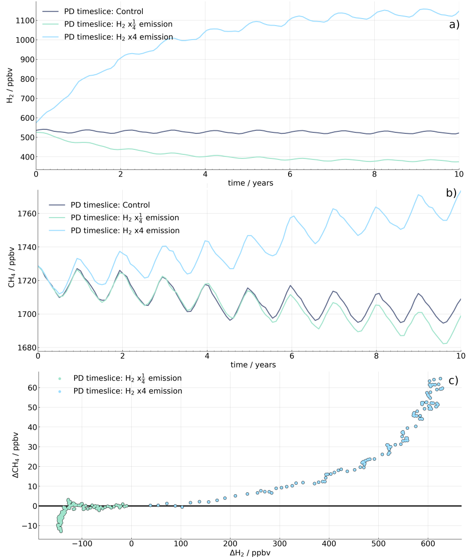
Figure 9. Global monthly averaged a) H_2 and b) CH_4 surface mixing ratios of the (dark blue) control, (green) \frac{1}{4} H_2 emissions, and (light blue). c) Difference between the control PD timeslice and the perturbed H_2 emissions simulations (perturbed emissions – control). Black line indicates no difference from the control. Timeslices are for 2020.
