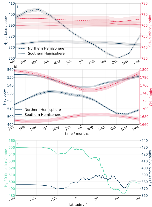
Figure 10. Five-year hemispherical averages of surface hydrogen (blue) and methane (red) mixing ratios for a) 1850 (TS-H 2 CH 4 -PI simulation) and b) 2020 (TS-H 2 CH 4 -PD simulation). Dashed lines show the northern hemisphere, while dotted lines show the southern. Shaded areas show one standard deviation calculated from the last five years of the simulation. c) Zonally averaged surface hydrogen mixing ratio for (blue) PI and (green) PD simulations (averaged over five years).
