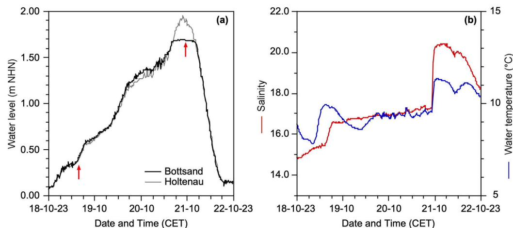
375 Figure 4. Water level (a), temperature, and salinity (b) during the Centennial Flood at Bottsand and Holtenau. The red arrows in (a) mark the salinity rises.
