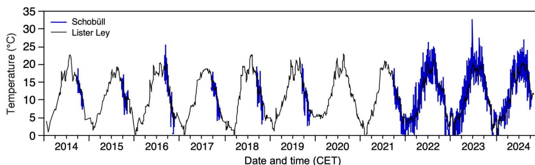
480 Figure 8. High water temperatures off Schobüll and surface water temperatures at Lister Ley monitoring station during the years 2014 through 2024.
