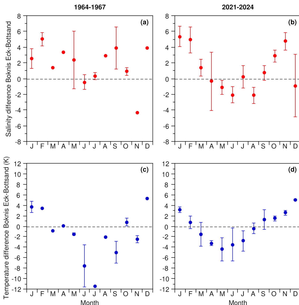
425 Figure 7. Mean monthly salinity (a, b) and temperature (c, d) differences between Bottsand lagoon and Boknis Eck. Dots: mean values, error bars: range of values.
