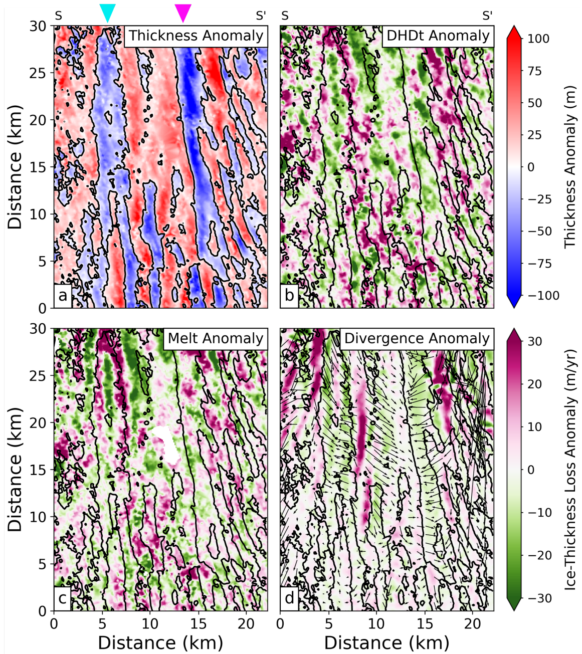
Figure 6. High-pass filtered anomaly of thickness (a), Lagrangian thickness change (b), basal melt (c) and ice flux divergence and velocity (d) within the black rectangle in Figure 2a. All variables are from 2015. The pink and cyan arrows indicate Channels 1 and 2, respectively, as discussed in the text.
