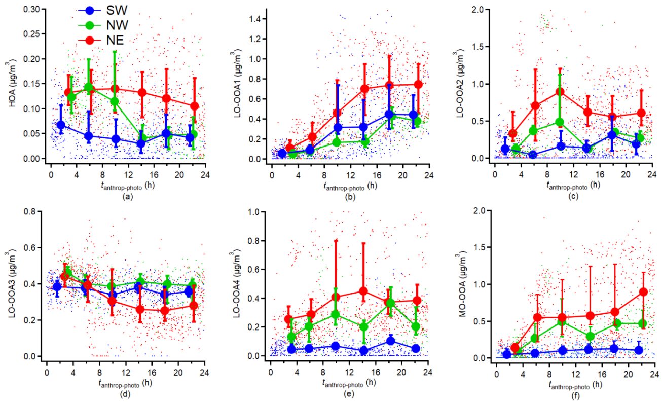
Figure 8: Variations in (a-f) HR-AMS PMF-derived factors normalised or non-normalised concentrations. The results are averaged into four-hour intervals along t_{\text{anthrop-photo}} and the error bar indicates the 25th and 75th percentiles, respectively.
