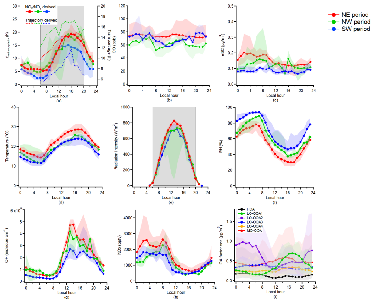
Figure 3: Diurnal variation of the (a) Relative anthropogenic photochemical age ( t_{\text{anthrop-photo}} ) derived from \text{NO}_x/\text{NO}_y ratio and trajectory-derived transport age; (b) CO mixing ratio; (c) eBC mass concentration; (d) Temperature; (e) Radiation Intensity; (f) RH; (g) OH concentration; (h) \text{NO}_x concentration; (i) PMF OA factors. The grey shades in (a) and (e) indicate the periods for the photochemical aging analysis. The lower and upper whiskers in the figure are the 25th and 75th percentiles, respectively.
