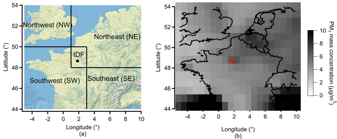
885 Figure 1: (a) Classification of the potential air mass source regions; (b) ECMWF CAMS EAC4 (ECMWF Atmospheric Composition Reanalysis 4) reanalysis PM 1 spatial distribution during the ACROSS campaign period. The dot in the figure represents the location of the Rambouillet measurement site. (the map information is from © Google Maps).
