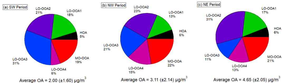
905 Figure 6: Pie charts for the mass fractions of different PMF OA factors during the three different airmass dominated periods. Values are reported as mean \pm standard deviation.
