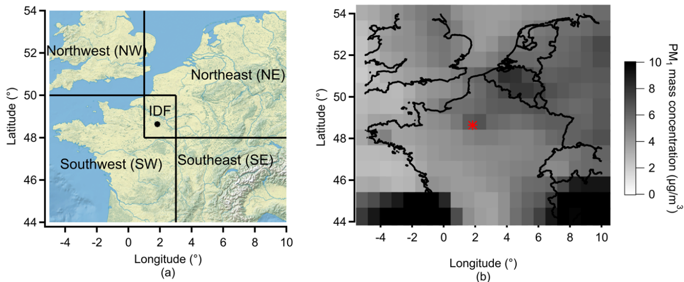
880 Figure 1: (a) Classification of the potential air mass source regions; (b) ECMWF CAMS EAC4 (ECMWF Atmospheric Composition Reanalysis 4) reanalysis PM 1 spatial distribution during the ACROSS campaign period. The dot in the figure represents the location of the Rambouillet measurement site. (the map information is from © Google Maps).
