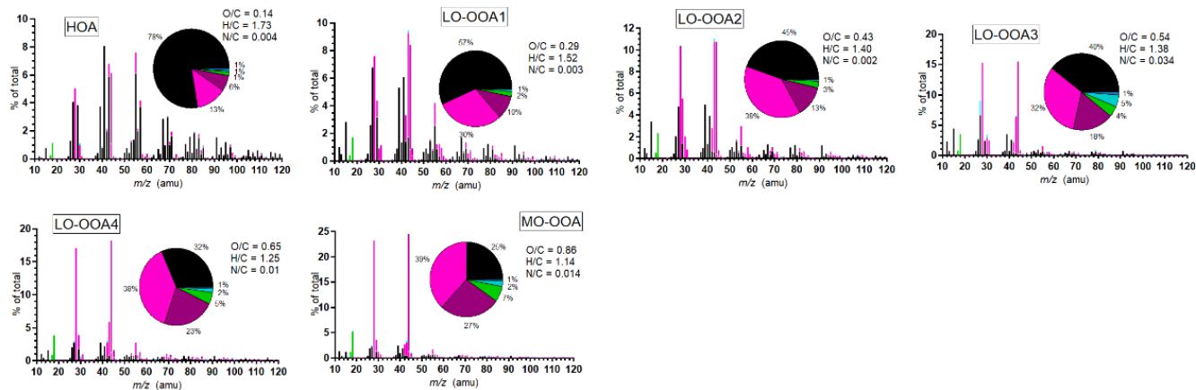
Figure 4: Average mass spectra for the PMF OA factors.
