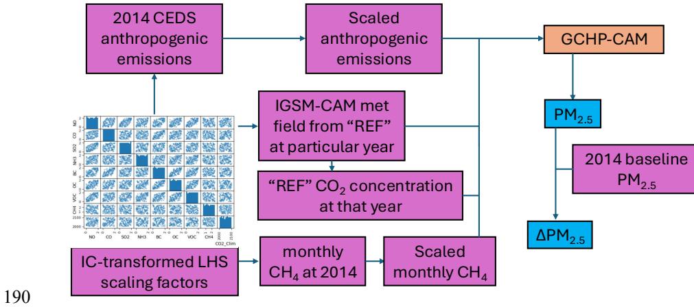
Fig. 2 Schematic of generating the training set by GCHP-CAM perturbation experiments using an Iman-Conover (IC) transformed Latin Hypercube Sampled (LHS) scaling factors. The orange box represents existing modelling systems, purple boxes represent data sets, and blue boxes represent output of the perturbation experiments.
