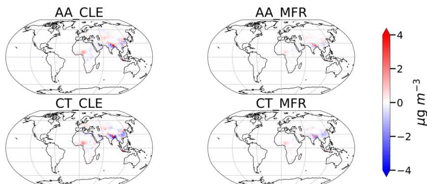
535 Fig. 18 Changes in absolute error (relative to GCHP-CAM output \Delta\text{PM}_{2.5} ) when an alternate set of L_i ( L_{\text{NH}_3} = L_{\text{NO}_x} = 1 grid cell, L_{\text{VOC}} = 2 grid cells, L_{\text{SO}_2} = 3 grid cells, L_{\text{BC}} = L_{\text{OC}} = 7 grid cells, L_{\text{CO}} = 15 grid cells, informed by the atmospheric lifetime of each pollutant i ( \tau_i )) is applied to train the GW-GPR. Red (positive) indicates that using the alternate set of L_i worsens the performance (increasing error), blue (negative) indicates the opposite.
