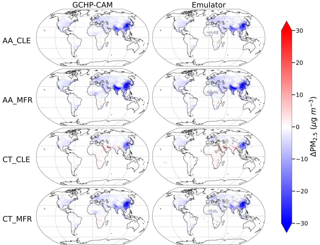
415 Fig. 10 Spatial patterns of GCHP-CAM and emulator predicted \Delta\text{PM}_{2.5} for each of the 4 IGSM-GAINS-TAPS scenarios at 2050 (relative to 2014). Only results in grid cells with population density > 1 person \text{km}^{-2} are shown. The hatches show where GCHP-CAM output does not fall within the 95% confidence interval of emulator prediction.
