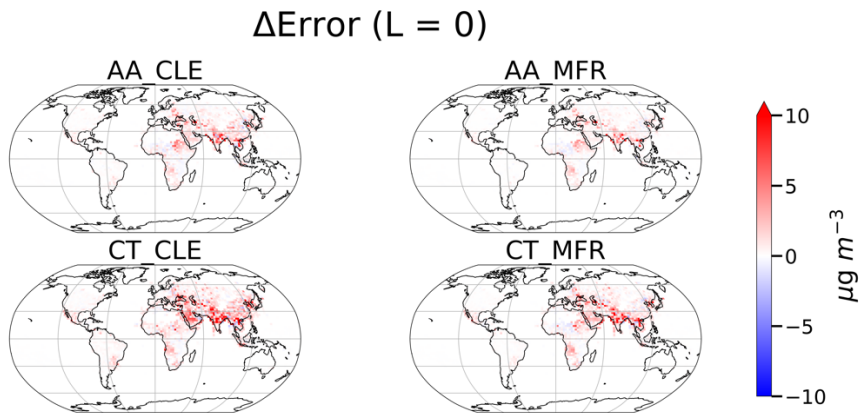
Fig. 15 Changes in absolute error (relative to GCHP-CAM output \Delta\text{PM}_{2.5} ) when no geographic weighting of pollutant emissions is implemented. Red (positive) indicates that turning off dispersion worsens the performance (increasing error), blue (negative) indicates the opposite.
