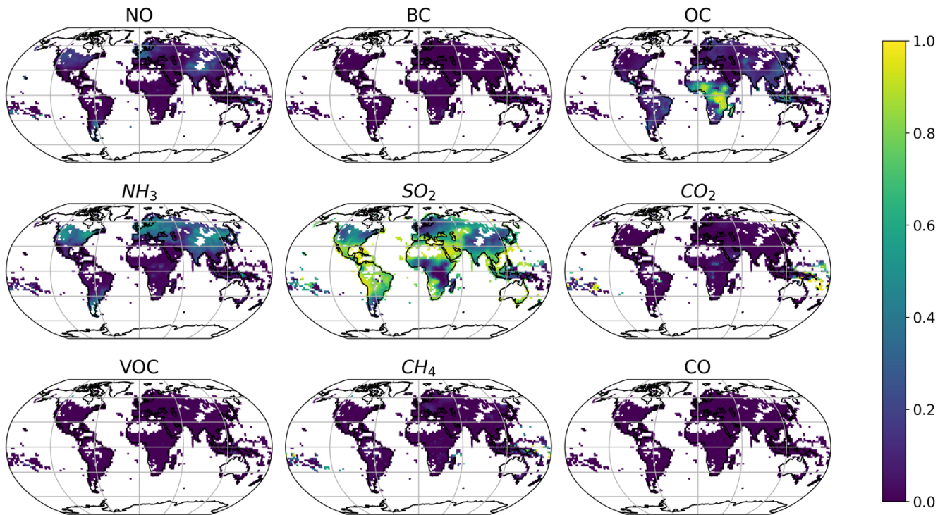
395 Fig. 9 Spatial patterns of Sobol Total Sensitivity Indices (0-1) for each predictor for \Delta\text{PM}_{2.5} . The indices indicate the fraction of output variance attributable to each input variables at each grid cell.
