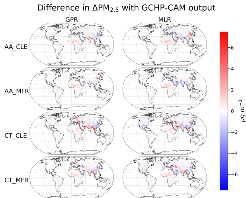
Fig. 12 GPR and MLR emulator errors relative to GCHP-CAM simulated \Delta\text{PM}_{2.5} over the 4 IGSM-GAINS-TAPS scenarios at 2050 (relative to 2014). Both emulators use the same geographic weighting scheme for pollutant emissions.
