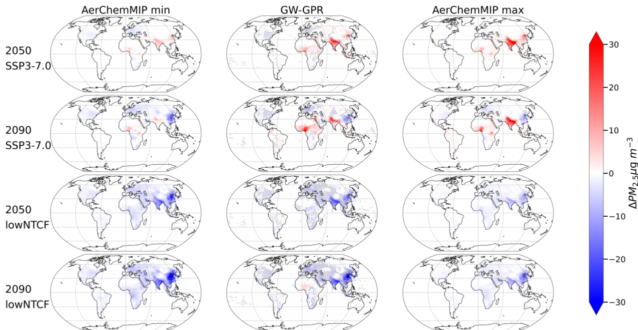
565 Fig. 20 Multimodel minimum and maximum magnitude of \Delta\text{PM}_{2.5} simulated by models in AerChemMIP, and GW-GPR emulator predicted \Delta\text{PM}_{2.5} in 2050 and 2090 under SSP3-7.0 and SSP3-7.0-lowNTCF (abbreviated as lowNTCF in plot labels). Dots in the middle (GW-GPR) column indicate the grid cells where prediction of GW-GPR do not fall between the minimum and maximum of AerChemMIP simulation output.
