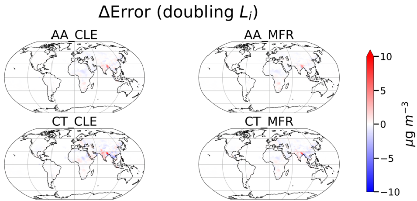
Fig. 17 Changes in absolute error (relative to GCHP-CAM output \Delta\text{PM}_{2.5} ) when the dispersion length scales ( L_i in Eq. 7) for all pollutants in the geographic weighing scheme are doubled. Red (positive) indicates that turning off dispersion worsens the performance (increasing error), blue (negative) indicates the opposite.
