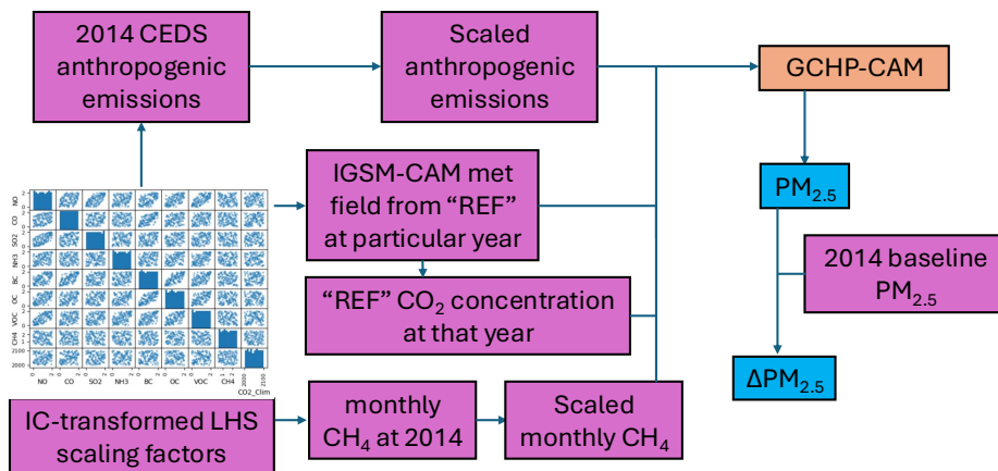
190 Fig. 2 Schematic of generating the training set by GCHP-CAM perturbation experiments using an Iman-Conover (IC) transformed Latin Hypercube Sampled (LHS) scaling factors. The orange box represents existing modelling systems, purple boxes represent data sets, and blue boxes represent output of the perturbation experiments.
