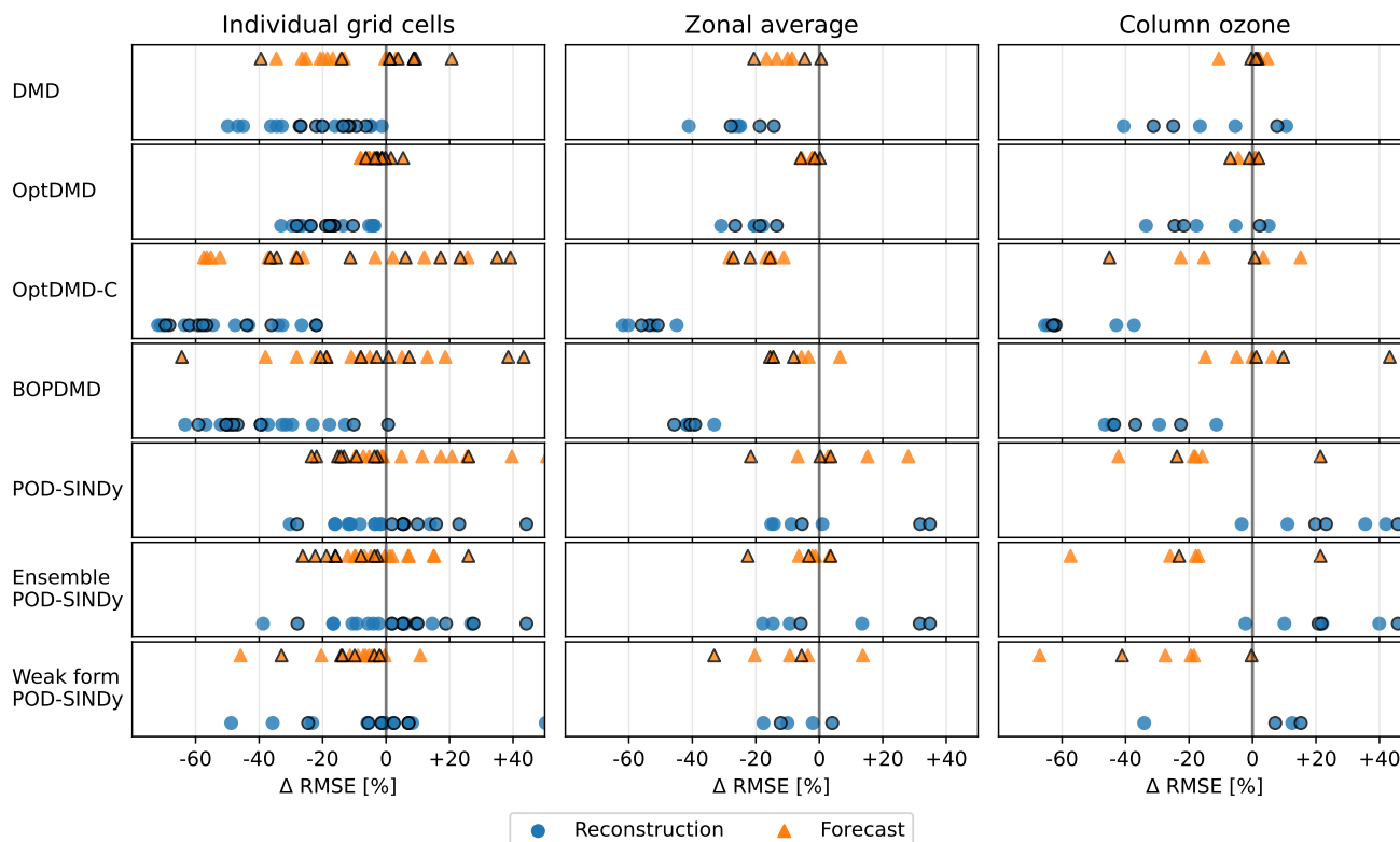
Figure 5. Change in the reconstruction (blue) and forecast (orange) RMSE with respect to reconstruction and forecasts using the temporal mean over all datasets for the methods used in this work. The left column shows the reconstruction of individual grid cells at altitudes of 1, 16, and 26 km (Table B1), the middle column the zonal average (Table 1), and the rightmost column the estimation of column ozone (Table 2). Markers with a black border denote the S1, S2, or S3 datasets.
