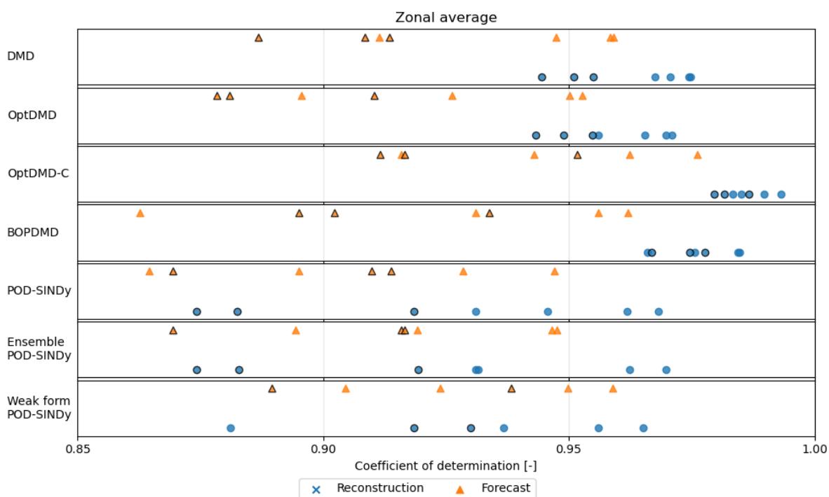
Figure C2. Comparison of the coefficient of determination for the zonal-average ozone response reconstructions (blue) and forecasts (orange) across all datasets for the individual methods.
