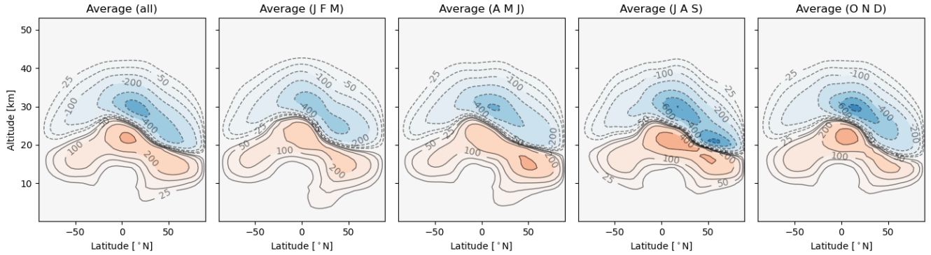
Figure 2. Average ozone response of the TAC204 dataset over different timespans. The leftmost plot shows the average response over all 5 years of data, and the other four show averages taken over 3-monthly snapshots from the entire dataset. For example, the rightmost figure (Average (O N D)) shows the average ozone response for the months of October, November, and December across the 5 years of data.
