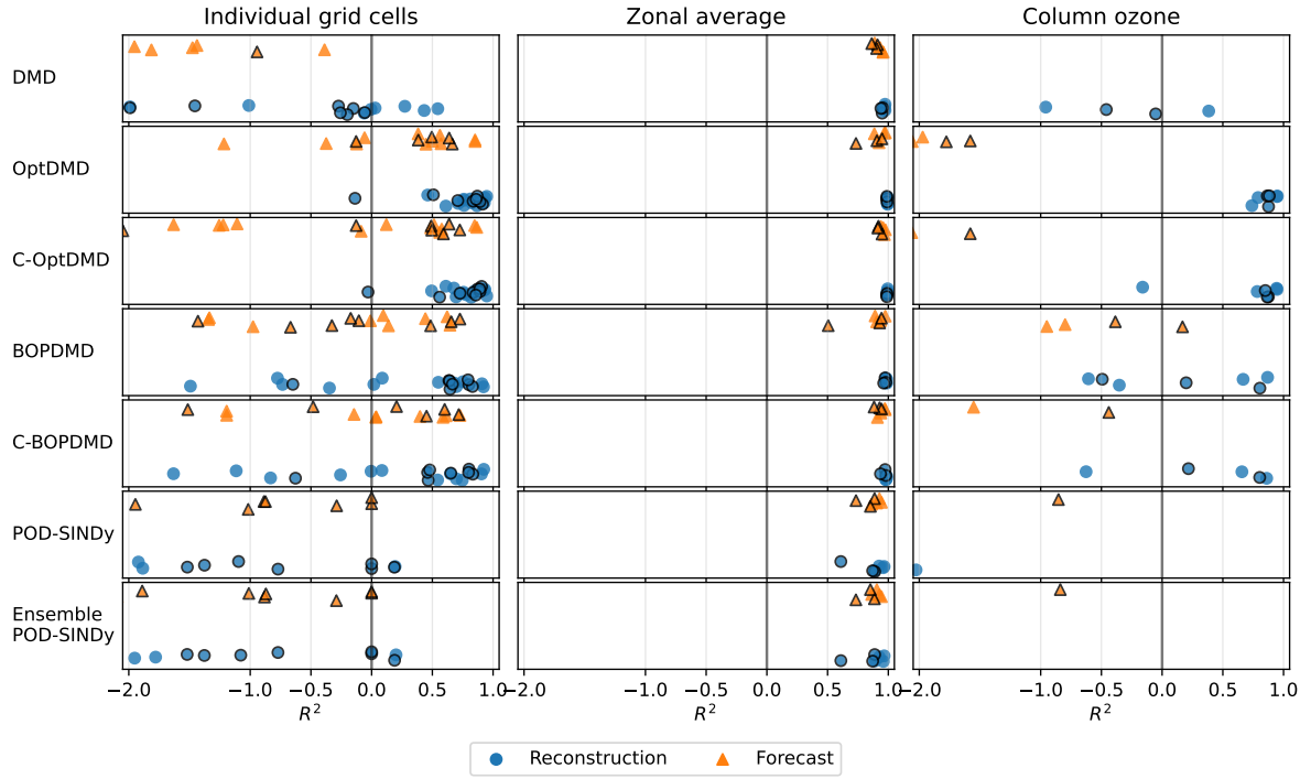
Figure C9. Comparison of the coefficient of determination for the single-cell (left), zonal-average (middle), and column ozone response ( right ). Reconstructions (blue) and forecasts (orange) are shown separately for the individual methods across all datasets.
