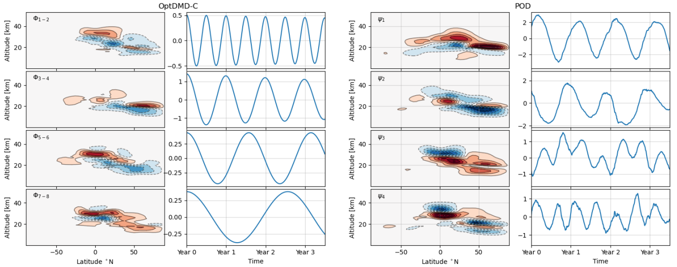
Figure 3. Spatial modes 1 to 4 and associated time coefficients of the C-OptDMD (left) and the POD method (right) extracted from the 3.5 years of fitting data from the TAC204 dataset. Modes of the C-OptDMD method are shown as pairs due to their nature as conjugate-couples. In both cases, values of the time coefficients are scaled down by a factor of 1 million kg.
