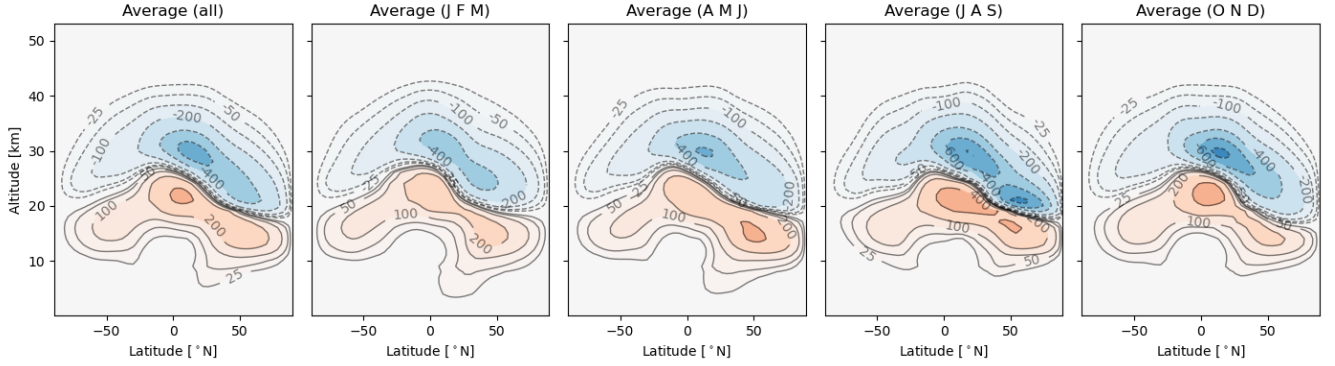
Figure 2. Average ozone response of the TAC204 dataset over different timespans in tons of ozone . The leftmost plot shows the average response over all 5 years of data, and the other four show averages taken over 3-monthly snapshots from the entire dataset. For example, the rightmost figure (Average (O N D)) shows the average ozone response for the months of October, November, and December across the 5 years of data.
