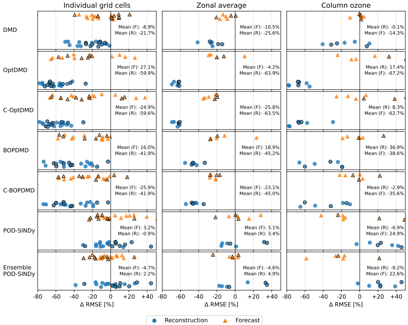
Figure 5. Change in the reconstruction (blue) and forecast (orange) RMSE with respect to reconstruction and forecasts using the temporal mean over all datasets for the methods used in this work. The left column shows the reconstruction of individual grid cells at altitudes of 1, 16, and 26 km (section B1), the middle column the zonal average (Table 1), and the rightmost column the estimation of column ozone (section 2). Markers with a black border denote the S1, S2, or S3 datasets.
