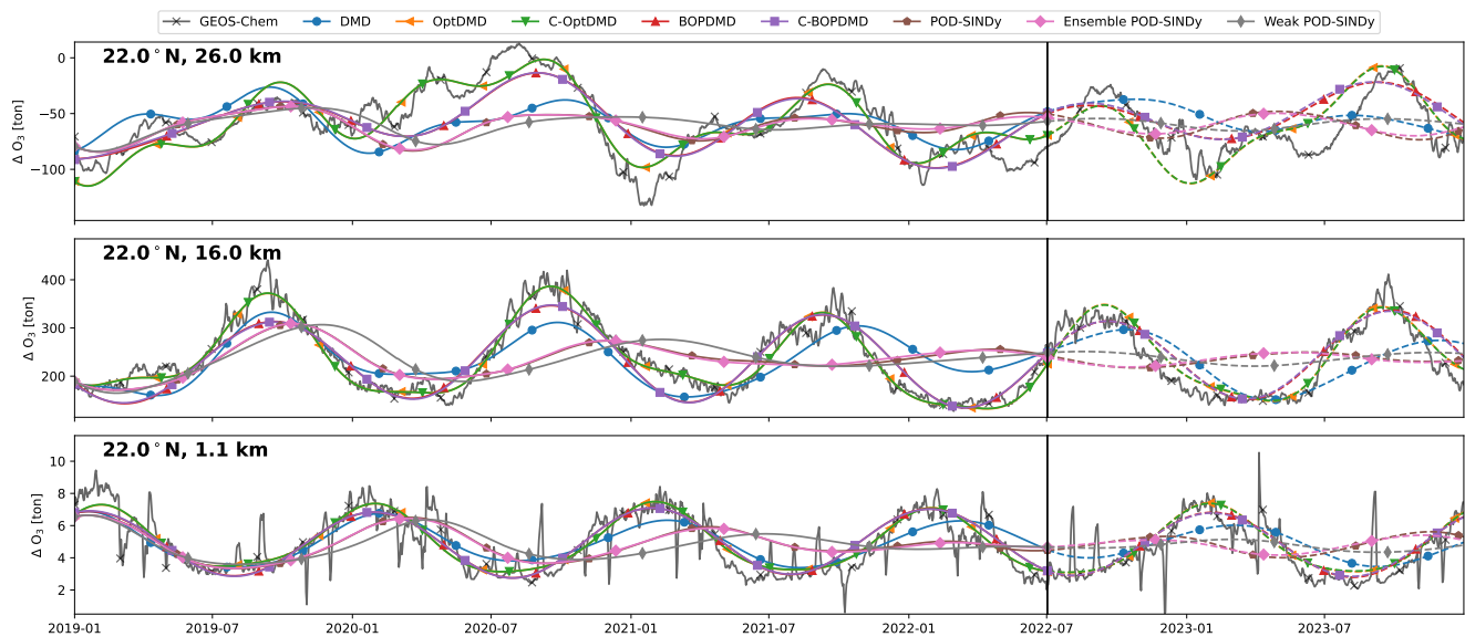
Figure C4. Same as Figure C3, but for the SAS162 dataset.
