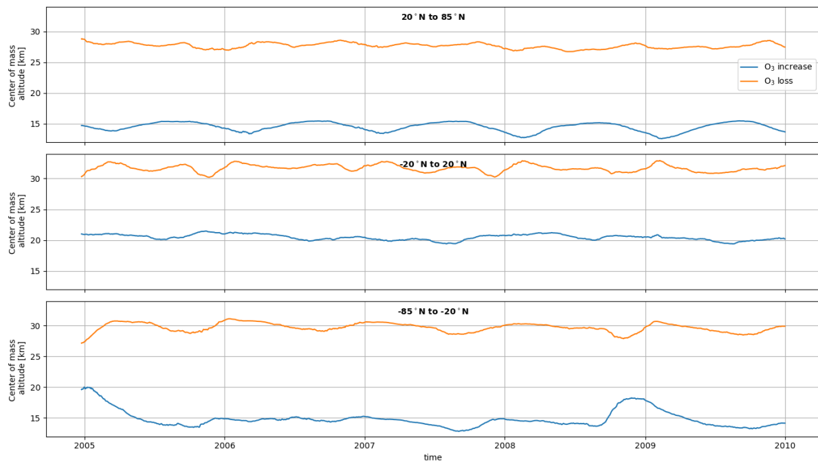
Figure C1. Altitude of the center of mass of the ozone response in the TAC204 dataset over time, calculated through a weighted average of the grid cells. Top row shows the northern hemisphere (20°N to 85°N), the middle shows the tropics (-20°N to 20°N), and the bottom row shows the southern hemisphere (-85°N to -20°N).
