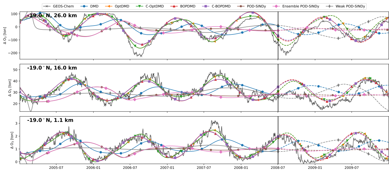
Figure C7. Same as Figure C3, but for the S2 dataset.
