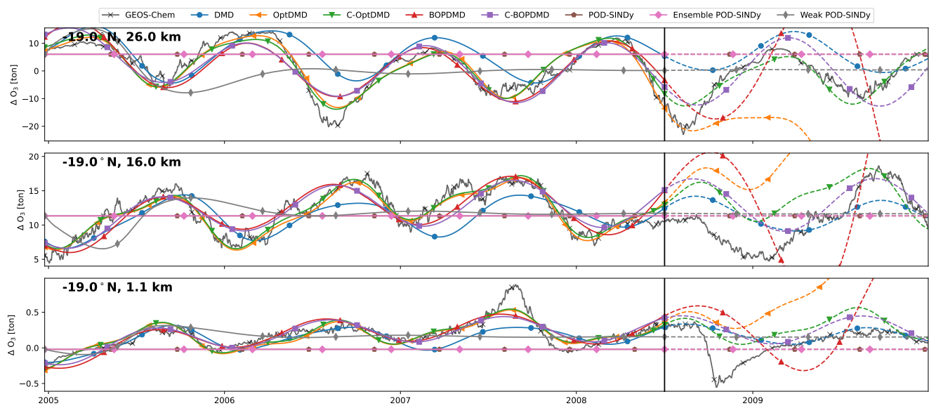
Figure C8. Same as Figure C3, but for the S3 dataset.
