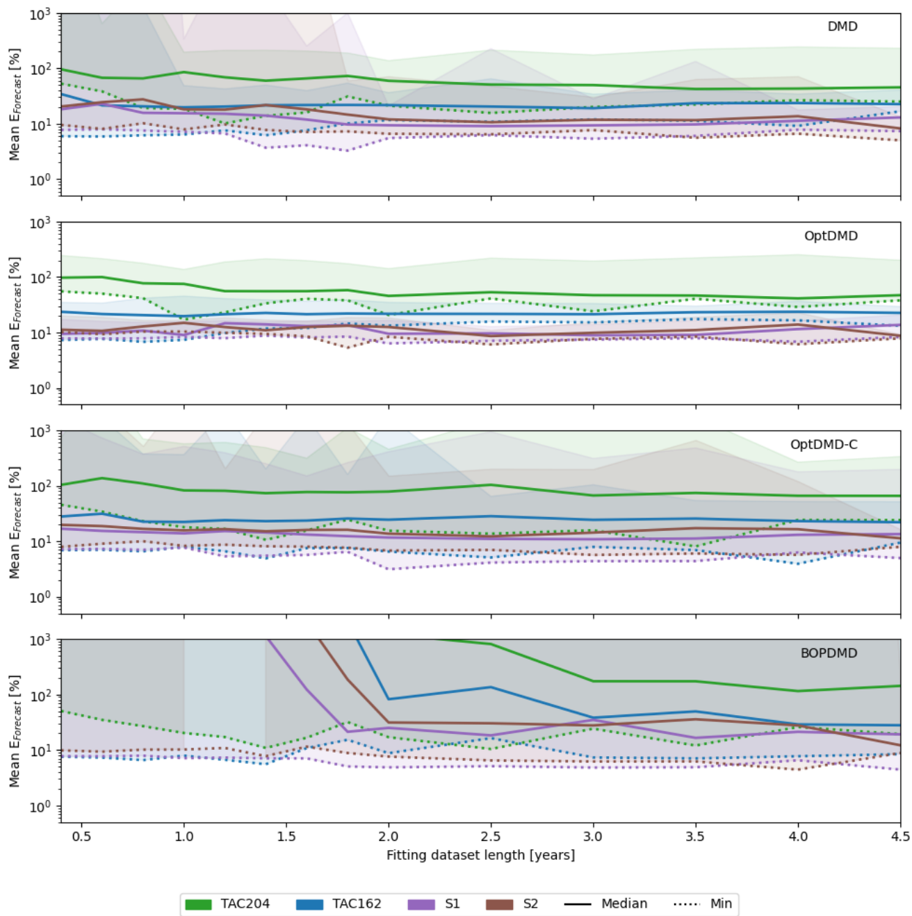
Figure A2. Results of hyperparameter sweep of DMD methods over the fitting dataset length DMD\_rank , for the TAC204, TAC162, S1, and S2 emission scenario datasets. The solid lines indicate the median O_3 column change forecast error in percent. The shaded areas mark the full range of results, and the dotted lines mark the lowest forecast errors achieved by any of the tried configurations.
