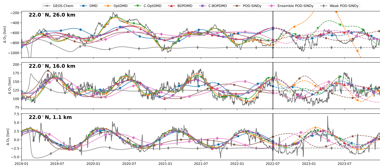
Figure C5. Same as Figure C3, but for the SAS204 dataset.
