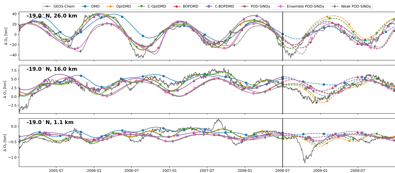
Figure C6. Same as Figure C3, but for the S1 dataset.
