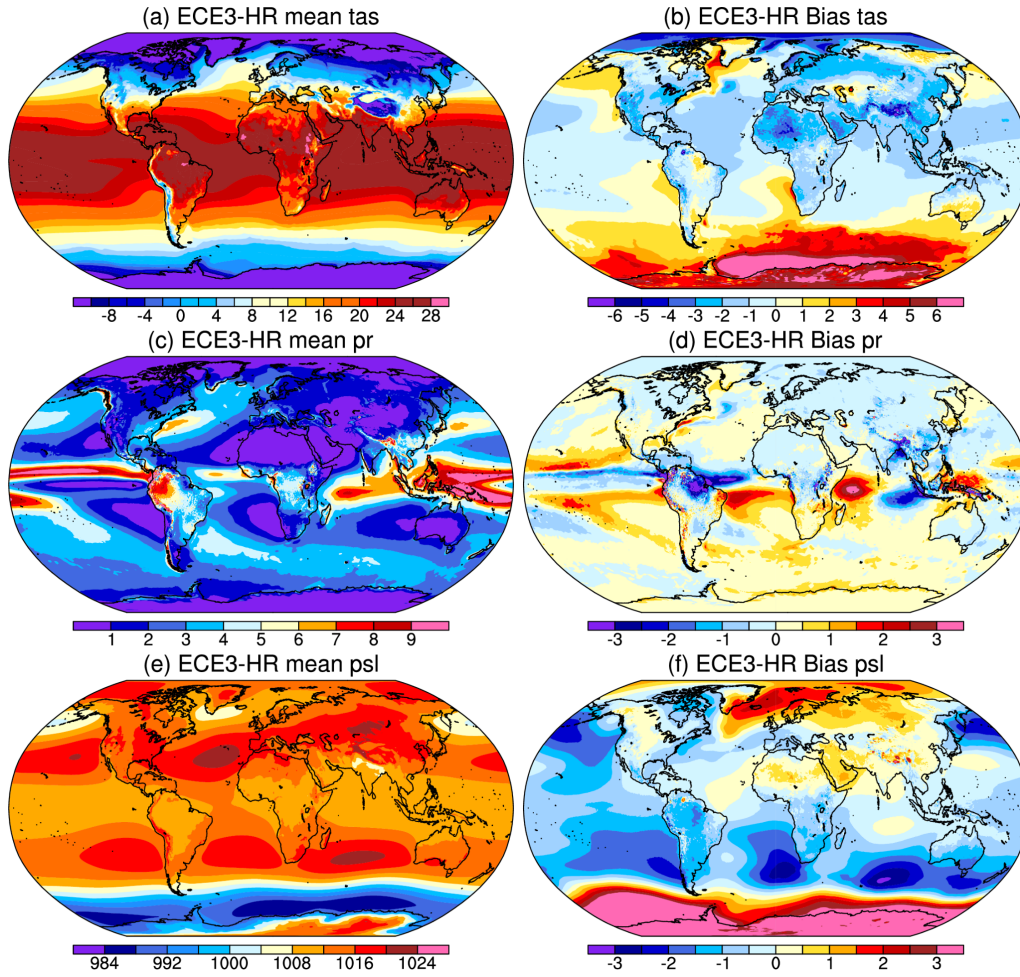
Figure 2. Annual mean (a) near-surface temperature (TAS, °C), (c) total precipitations (pr, mm/day) and (e) sea level pressure (psl, hPa) simulated by EC-Earth3-HR for the period 1980-2010, and (b), (d), (f) their respective biases compared to ERA5.
