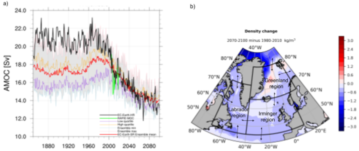
Figure 9. (a) Annual-mean AMOC strength (maximum overturning stream function between 20°–40°N at 800–1100 m depth) from 1850 to 2100 in EC-Earth3-HR (black), the 14-member EC-Earth3-SR ensemble (red is the ensemble mean, and grey shading indicates ensemble spread including minimum, maximum, and interquartile range), and RAPID-MOCHA observations (Smeed et al., 2018; green). (b) Winter mean (JFM) surface density change ( \text{kg/m}^3/\text{decade} ) between the 2070–2100 and 1980–2010 periods in the North Atlantic showing the three analysis regions used in Section 4.4: the Greenland, Irminger, and Labrador regions. These polygons represent extended areas encompassing and surrounding the respective seas. Arrows indicate the sections where inflows and outflows are calculated.
