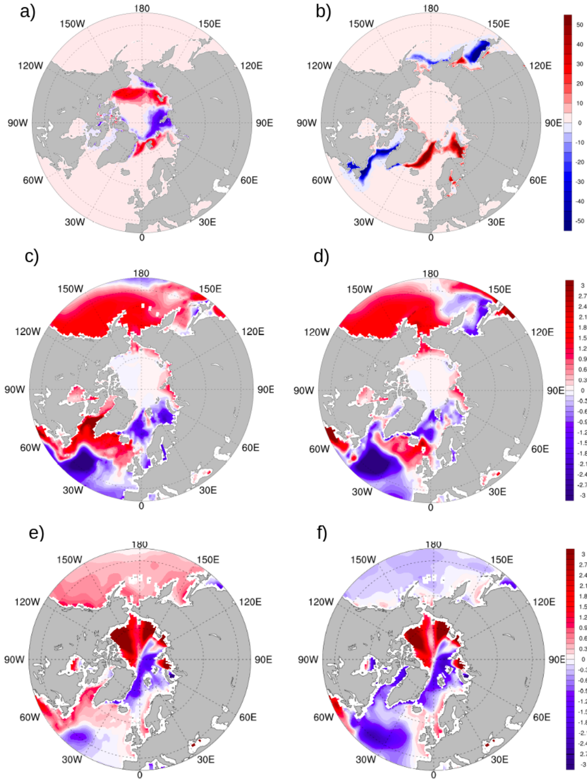
Figure 3. Mean biases over 1980–2010. (a, b) Difference in sea ice concentration (%) between the EC-Earth3-HR model and satellite observations for September and March, respectively. (c, d) Annual mean sea surface temperature (SST; °C) bias in EC-Earth3-HR and the EC-Earth3-SR ensemble mean relative to HadISST, respectively. (e, f) Sea surface salinity (SSS; psu) bias in EC-Earth3-HR and the EC-Earth3-SR ensemble mean compared to WOA18, respectively.
