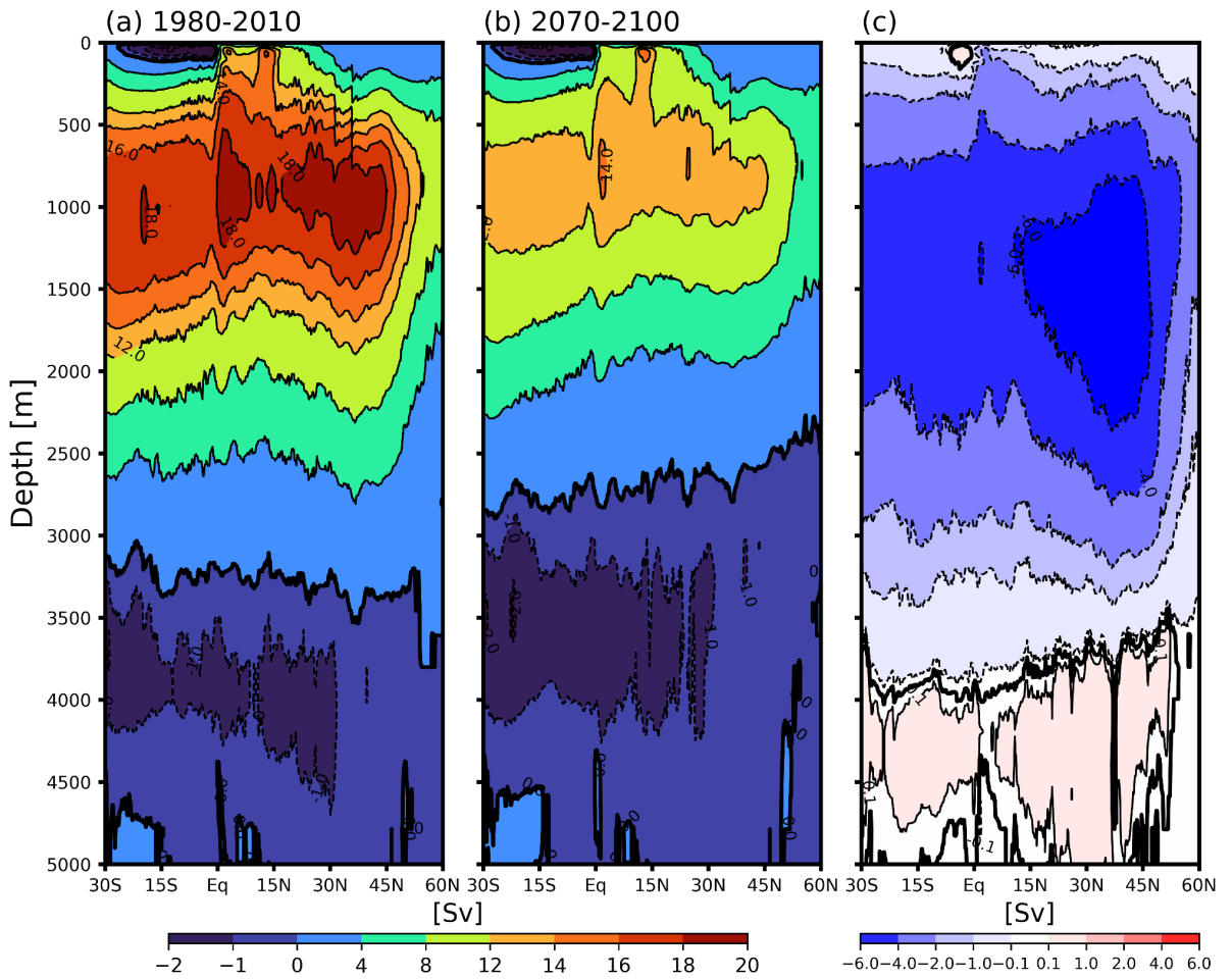
Figure 8. AMOC stream function (Sv) in the depth-latitude space for EC-Earth3-HR, averaged over 1980–2010 (a) and 2070–2100 (b) and the difference between the two periods (c).
