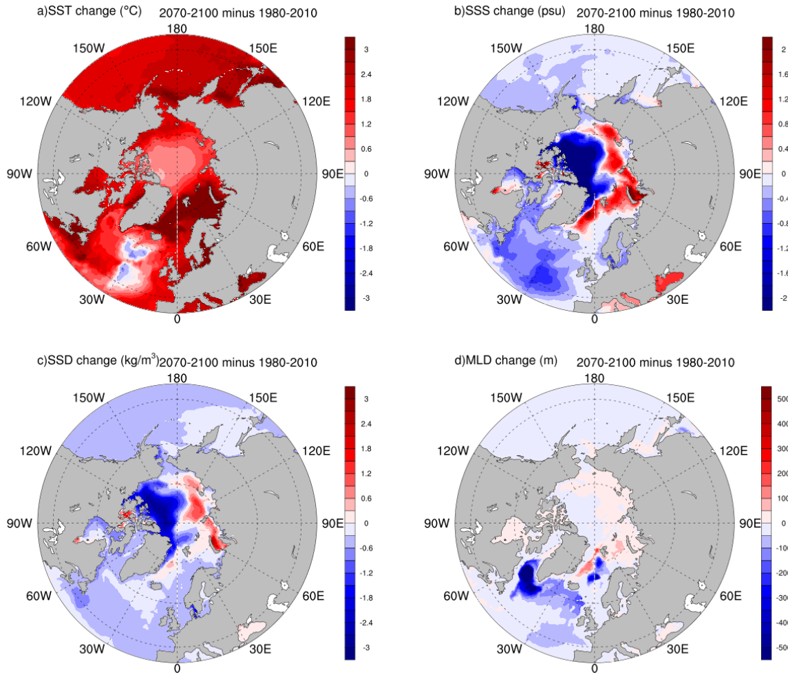
Figure 7. Differences between the 2070–2100 and 1980–2010 periods under the SSP2-4.5 scenario in EC-Earth3-HR for: (a) annual mean sea surface temperature (SST, °C); (b) annual mean sea surface salinity (SSS, psu); (c) winter mean (JFM) sea surface density (SSD, kg/m 3 ); (d) winter mean (JFM) mixed layer depth (MLD, m). All figures are shown for 40°N northward.
