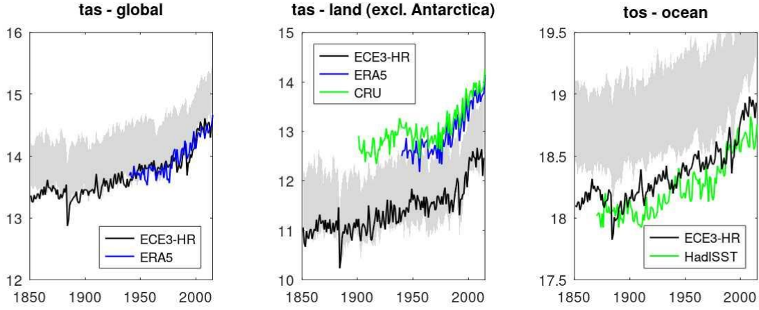
Figure 1. Time series of surface air temperature (TAS, °C) and sea surface temperature (SST, °C) from EC-Earth3-HR (black), ERA5 reanalysis (blue), CRU over land (green), and HadISST over ocean (green) for the historical period. The full range of the EC-Earth3-SR CMIP6 historical ensemble is shown as a grey shaded area. Panels show: a) global mean, b) global mean over land (excluding Antarctica), and c) global mean over ocean.
