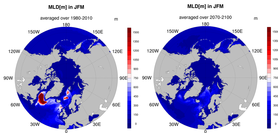
757 Figure A7. EC-Earth3-HR winter mean (JFM) mixed layer depth (MLD, m) averaged over 1980-2010 (left panel) and 758 2070-2100 (right panel).
