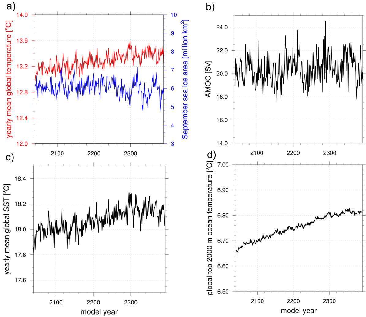
710 Figure A1. Time series from the 350-year EC-Earth3-HR pre-industrial (PI) control run showing: (a) annual-mean 711 global surface air temperature (°C, red) and September sea ice area (million km 2 , blue); (b) annual-mean AMOC 712 strength, defined as the maximum overturning streamfunction between 20°–40°N at 800–1100 m depth. (c) 713 annual-mean global sea-surface temperature (SST); and (d) annual-mean global vertically averaged upper-ocean 714 temperature (0–2000 m).
