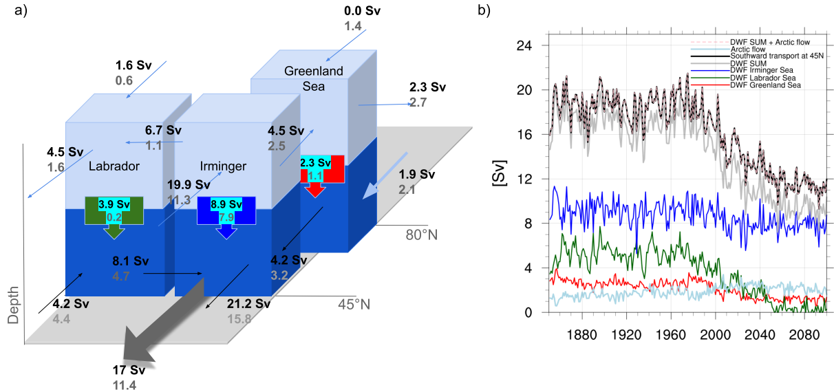
532 533 Figure 12. (a) Illustration of the regions used for DWF calculations: blue thin arrows represent inflows and outflows in 534 the upper layers, and black arrows indicate flows in the lower layers. Colored callouts with the downward arrows 535 display DWF, with values in black corresponding to the 1980–2010 mean and numbers in grey to the 2070–2100 mean. 536 The large grey arrow represents the net flow through 45°N, calculated as the sum of all DWFs and the deep inflow 537 from the Arctic into the Greenland Sea. The thick blue arrow shows the deep outflow from the Arctic into the 538 Greenland Sea. (b) Time series of southward deep transport at 45°N (black) and deep water formation (DWF) rates in 539 the Irminger (blue), Labrador (green), and Greenland (red) seas, Arctic flow below 1000m (light blue), together with 540 sum of all DWFs ( DWF SUM in grey) and DWF SUM plus deep Arctic flow (pink dashed), from 1850 to 2100 in 541 EC-Earth3-HR. The close agreement between the southward transport at 45°N with DWF SUM plus Arctic flow 542 demonstrates volume conservation of the system. All values are in Sverdrups (Sv). A long-term decline is evident in 543 AMOC and DWF, particularly after the year 2000. 544
