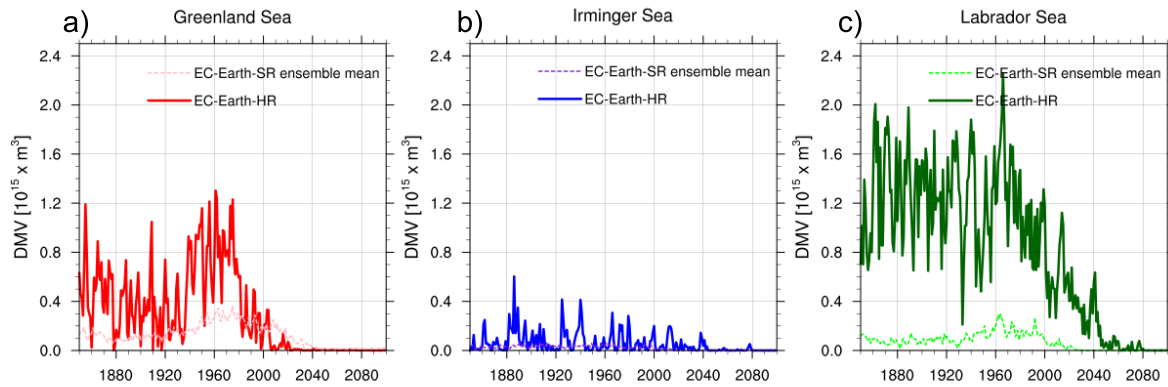
513 Figure 11. Deep Mixed Volume (DMV) in the Greenland (a), Irminger (b), and Labrador (c) Seas from historical and 514 SSP2-4.5 simulations of EC-Earth3-HR (thick lines) and the ensemble mean of EC-Earth3-SR simulations (dashed 515 lines). We chose the reference depth of 1000 m for the Labrador and Irminger Seas and 700 m for the Greenland Sea. 516
