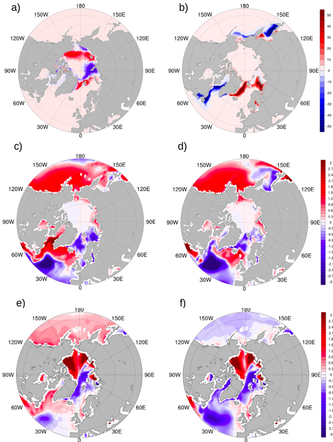
262 Figure 3. (a, b) Difference in sea ice concentration (%) between the EC-Earth3-HR model and satellite observations, 263 averaged over 1980–2010; (a) shows September, (b) shows March. (c, d) Sea surface temperature (SST) bias (°C) 264 compared to HadISST in EC-Earth3-HR and the ensemble mean of EC-Earth3-SR, respectively. (e, f) Sea surface 265 salinity (SSS) bias (psu) compared to the WOA18 climatology in EC-Earth3-HR and the ensemble mean of 266 EC-Earth3-SR, respectively. 267
