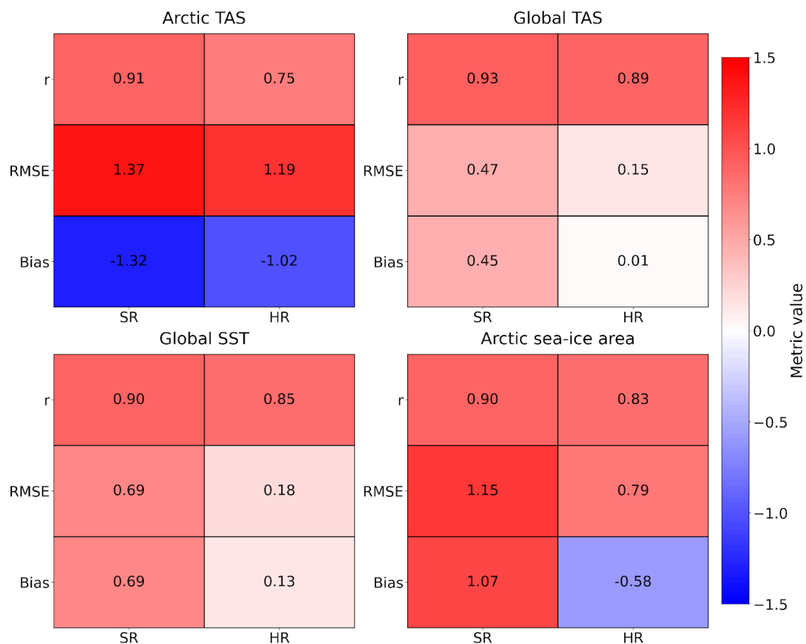
751 Figure A6. Quantitative evaluation of EC-Earth3-SR and EC-Earth3-HR performance relative to observations and 752 reanalysis for Arctic and global surface air temperature (TAS), global sea surface temperature (SST), and 753 sea-ice area. Shown are correlation (r), root-mean-square error (RMSE), and mean bias for each variable. Metrics are 754 computed over the historical period: 1950–2014 for TAS, 1870–2014 for SST, and 1979–2014 for sea ice.
