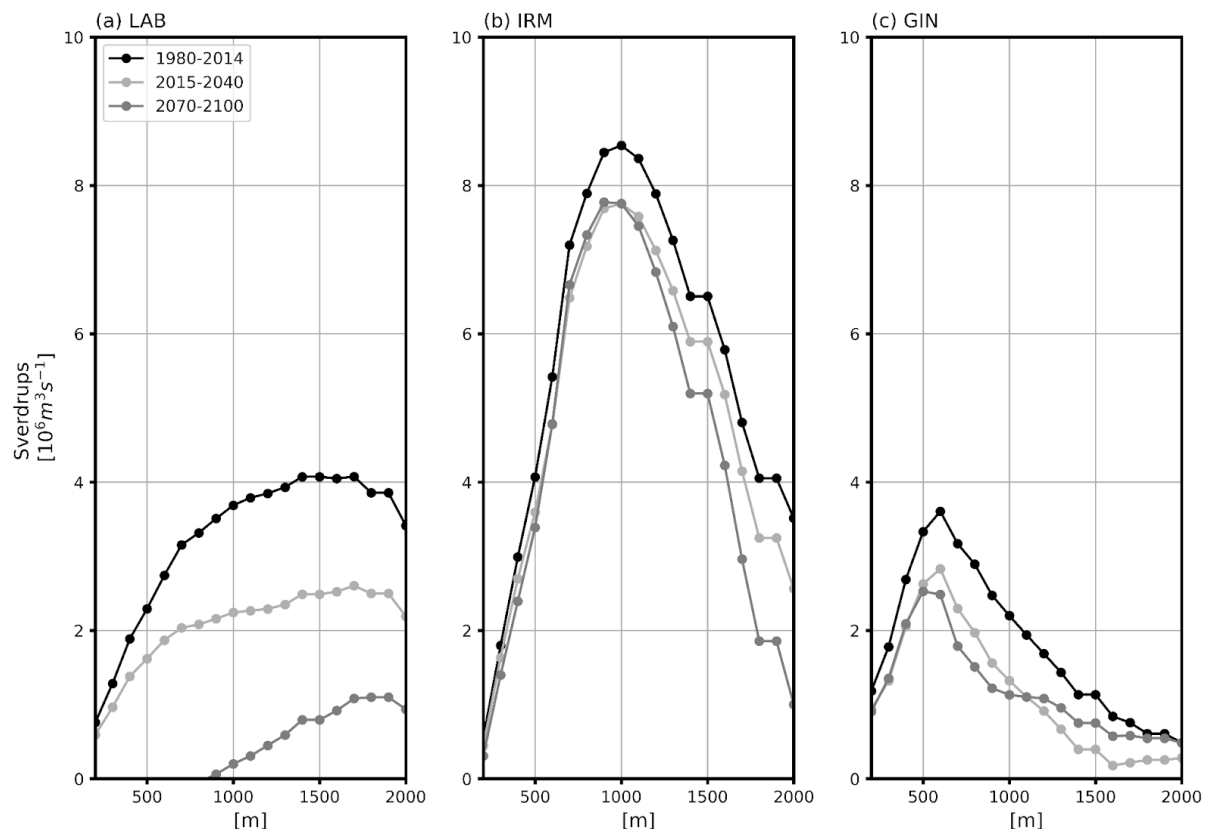
761 Figure A8. Sensitivity of the deep-water formation (DWF) index to the choice of reference depth for the Labrador 762 (LAB), Irminger (IRM), and GIN seas, shown for the historical period (mean over 1980–2014) and two future periods 763 (mean over 2015–2040 and 2070–2100). While the magnitude of the DWF index depends on the reference depth, the 764 relative regional contrasts and projected future changes are robust.
