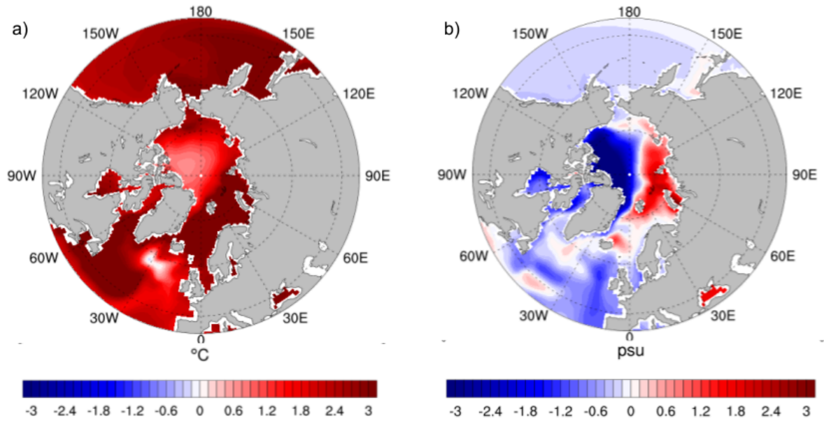
737 Figure A4. Differences between the 2071–2100 and 1980–2100 periods under the SSP2-4.5 scenario for the 738 EC-Earth3-SR ensemble mean: (a) annual mean sea surface temperature (SST, °C); (b) annual mean sea surface 739 salinity (SSS, psu).
