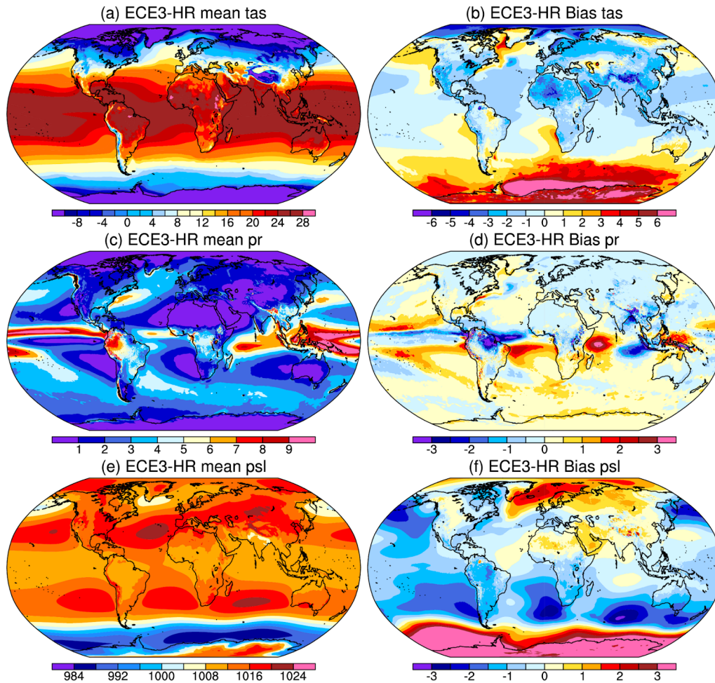
254 Figure 2. Annual mean (a) near-surface temperature (TAS, °C), (c) total precipitations (pr, mm/day) and (e) sea level 255 pressure (psl, hPa) simulated by EC-Earth3-HR for the period 1980-2010, and (b), (d), (f) their respective biases 256 compared to ERA5.
