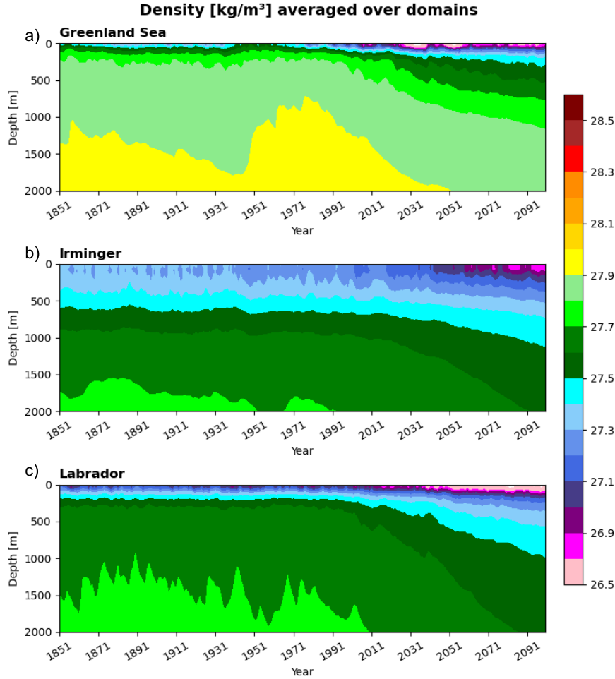
477 Figure 10. Time–depth evolution of winter (JFM) density ( \text{kg m}^{-3} ) averaged over the Greenland, Irminger, and 478 Labrador regions (shown in 9b) from 1850 to 2100. Color shading indicates isopycnal structure. The regions 479 correspond to polygons shown in Figure 9b.
