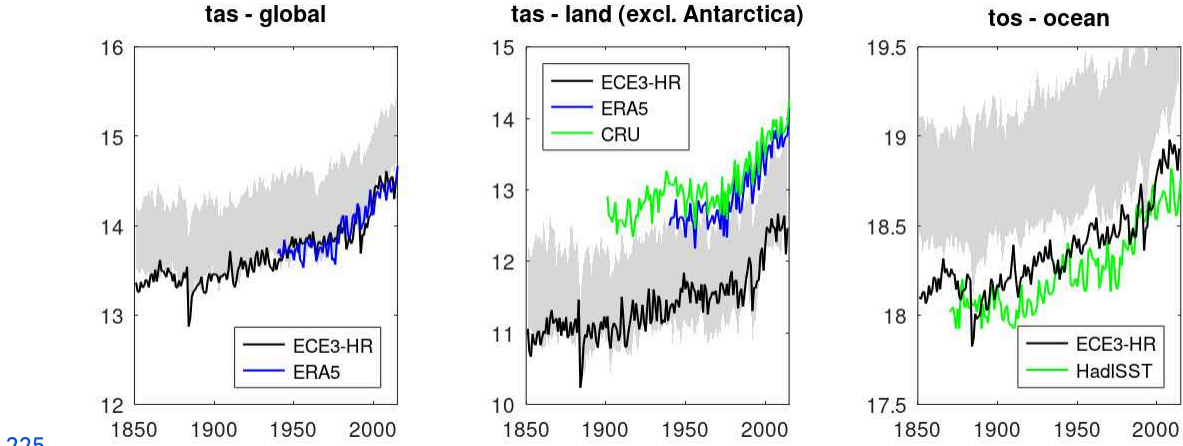
Figure 1. Time series of surface air temperature (TAS, °C) and sea surface temperature (SST, °C) from EC-Earth3-HR (black), ERA5 reanalysis (blue), CRU over land (green), and HadISST over ocean (green) for the historical period. The full range of the EC-Earth3-SR CMIP6 historical ensemble is shown as a grey shaded area. Panels show: a) global mean, b) global mean over land (excluding Antarctica), and c) global mean over ocean.
