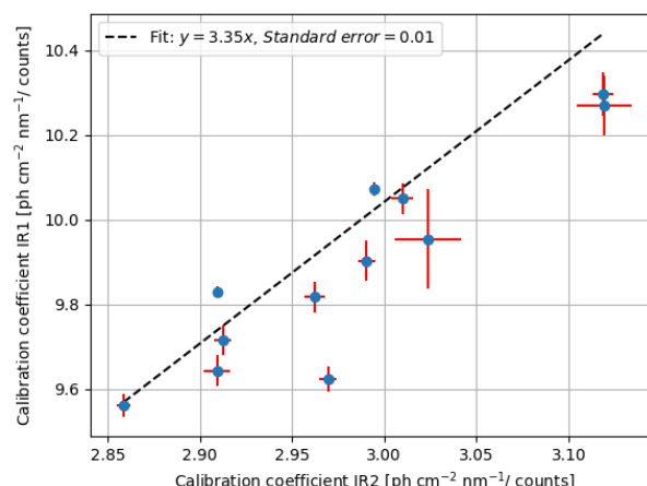
Figure 11. Example of how the relative calibration coefficients, in this case IR1 versus IR2, were determined. Each point marks the absolute calibration coefficients obtained for the two channels for one particular star. The relative calibration factor is given by the slope of the fitted line.
