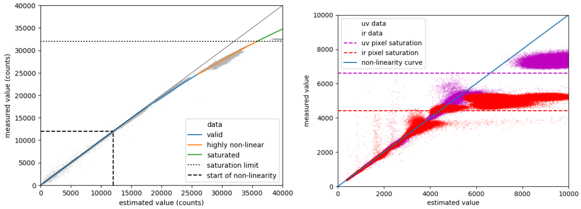
Figure 7. Left: The non-linearity curve from the readout electronics fitted on data from the lab measurements (gray). The second order term in the non-linearity starts at 11 993 (dashed line) and the measured values above 32000 (dotted line) is marked to indicate ADC saturation. Right: Single pixel non-linearity data from IR (red) and UV (magenta) and the corresponding saturation levels (dashed curves).
