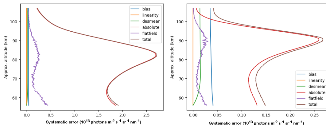
Figure 15. Systematic sources of error for a typical night and dayglow image (IR1 channel).
