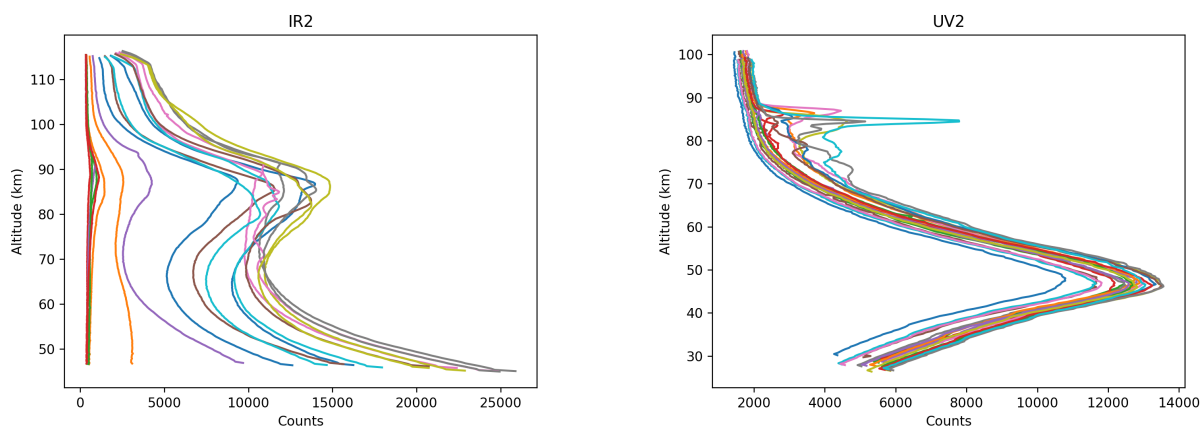
Figure 9. Examples of un-cropped profiles for the IR2 channel and the UV2 channel, used for determining the best function to approximate the data in the cropped part of the image. The profiles of the IR2 channel show similar behaviour to those of the IR1, IR3, IR4 and UV1 channel (not shown). The profiles for UV2 on the other hand, where the CCD field of view is lower, are heavily influenced by ozone absorption and baffle vignetting at lower altitudes 2023-01-09.
