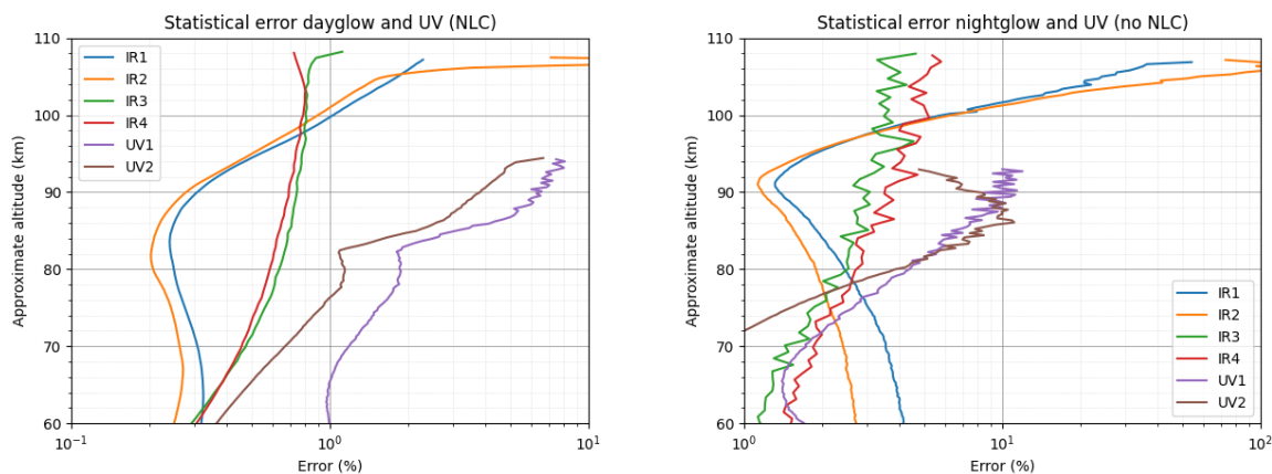
Figure 14. Typical statistical error in relative units. Left: errors during daytime, comprising dayglow in the IR and NLC in the UV. Right: errors during nighttime, comprising nightglow in the IR and no NLC in the UV.
