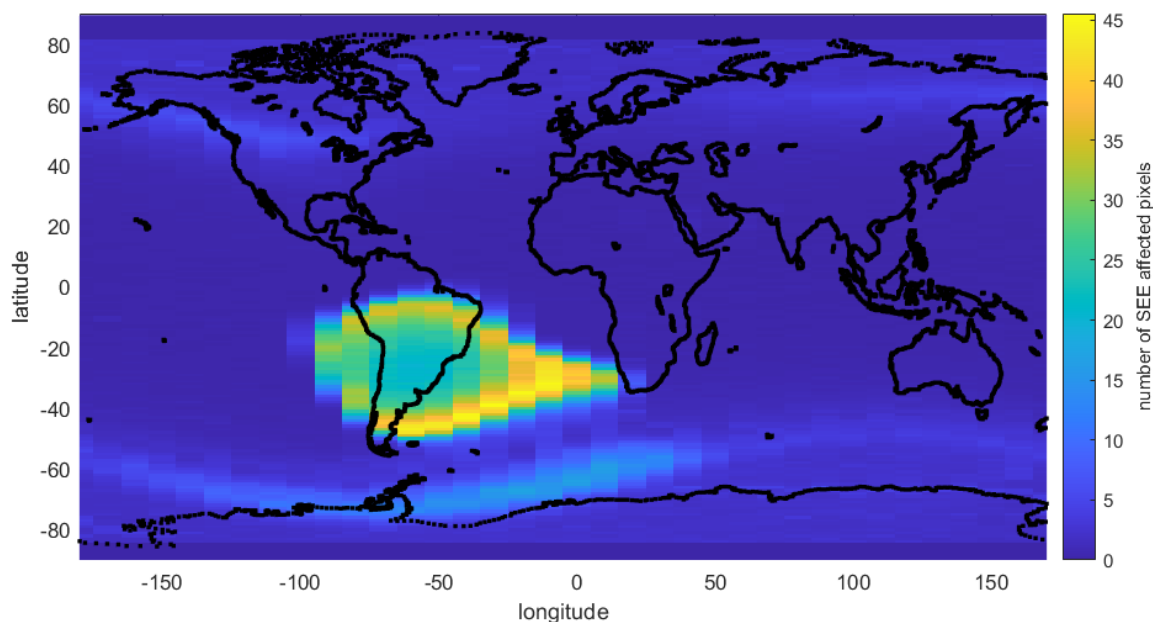
Figure 6. Average number of single event affected pixels per image with count values exceeding 200, for IR1 channel between December 2022 and May 2023. Note that the marked position is the satellite position at the time the image was taken, not the tangent point of the measurement. This means that these single events will impact images of the atmosphere north or south of the marked region, depending on which way the satellite is moving (ascending or descending node).
