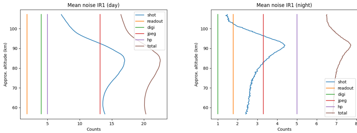
Figure 13. Mean statistical errors for various error types for the IR1 channel, presented for dayglow (left) and nightglow (right).
