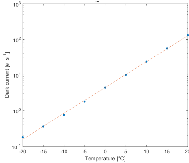
Figure 10. Average dark current in electrons per second, as a function of temperature as measured in the cold chamber for the IR1 channel CCD.
