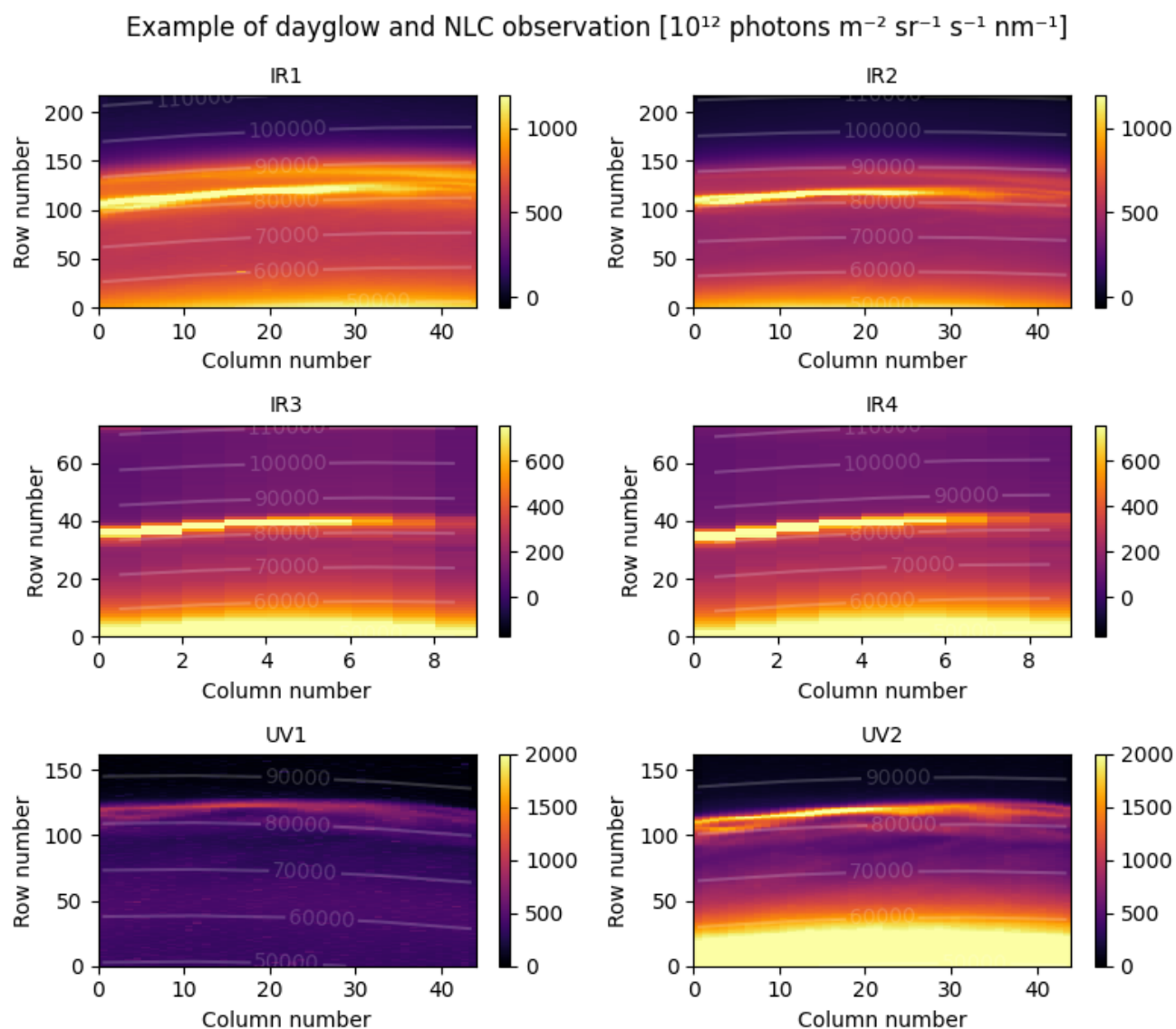
Figure 12. Example of calibrated images for an observation of dayglow and NLC, for the different limb channels. The white lines mark the altitude in metres.
