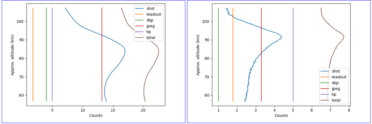
Figure 12. Mean statistical errors uncertainty in counts for various error types for the IR1 channel, presented for dayglow (left) and nightglow (right).
