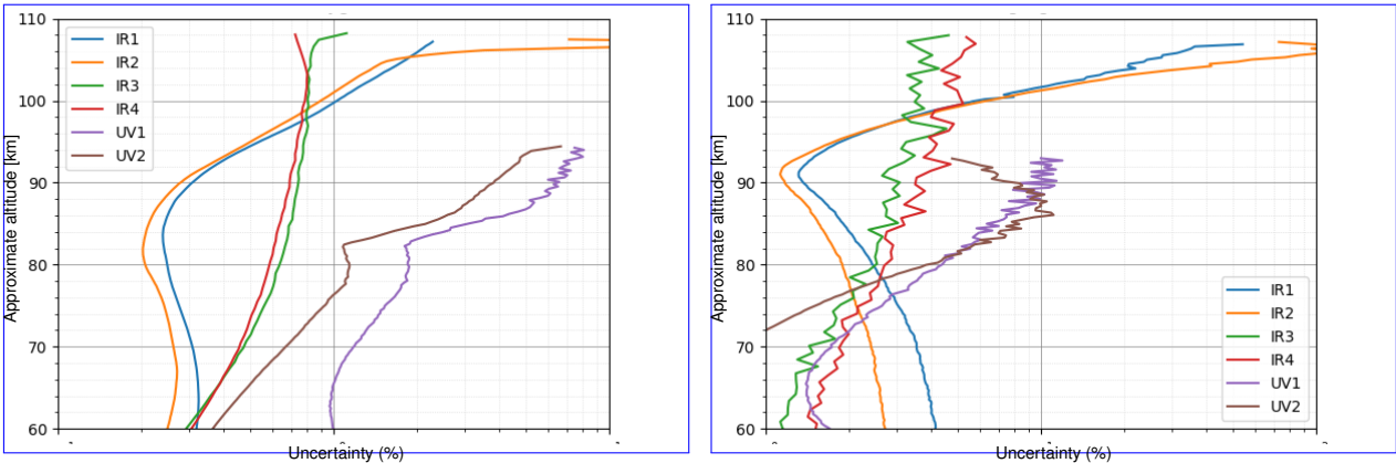
Figure 13. Typical statistical error-uncertainty in relative units. Left: errors-uncertainty during daytime, comprising dayglow in the IR and NLC in the UV. Right: errors-uncertainty during nighttime, comprising nightglow in the IR and no NLC in the UV.
