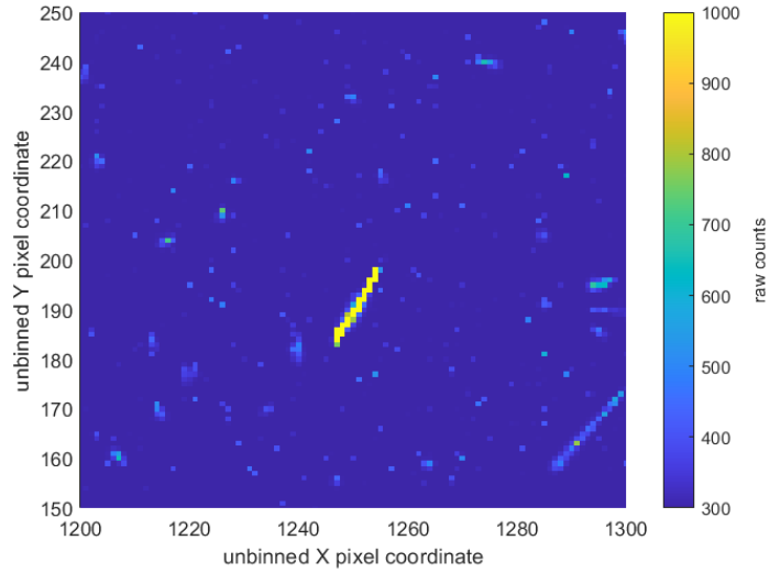
Figure 5. Example of server severe singular event impact on a section of an unbinned image, taken over the problematic region of South Atlantic anomaly (IR1 channel, 2023, August 30, 21:15:02 UT). The colour scale is in raw counts as registered by the detector (thus including bias, dark current etc.) and the axes show the unbinned column and row numbers.
