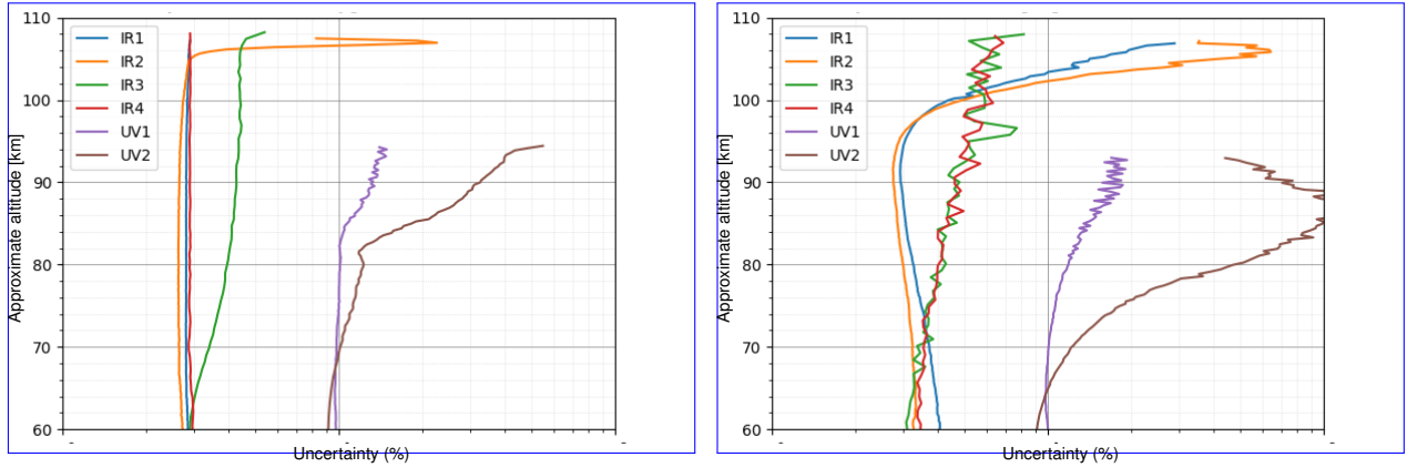
Figure 15. Mean-Typical systematic error (uncertainty in relative to signal) of IR channels for dayglow (left) units. Left: uncertainty during daytime, comprising dayglow in the IR and of all channels for NLC in the UV. Right: uncertainty during nighttime, comprising nightglow (right) in the IR and no NLC in the UV. Mean-Typical systematic error (uncertainty in relative to signal) of IR channels for dayglow (left) units. Left: uncertainty during daytime, comprising dayglow in the IR and of all channels for NLC in the UV. Right: uncertainty during nighttime, comprising nightglow (right) in the IR and no NLC in the UV.
