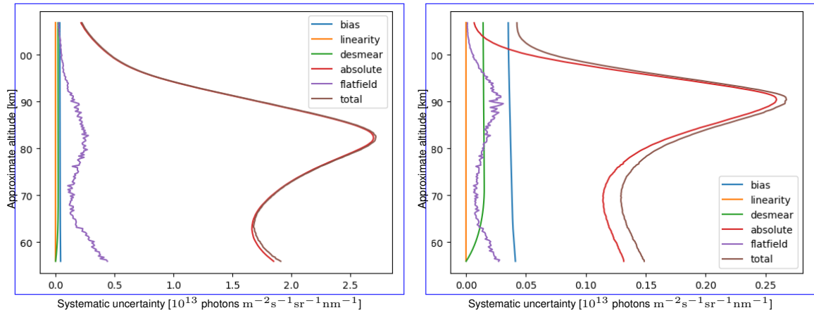
Figure 14. Systematic sources of Mean systematic uncertainty for various error types for a typical night and dayglow image (the IR1 channel, presented for dayglow (left) and nightglow (right)).
