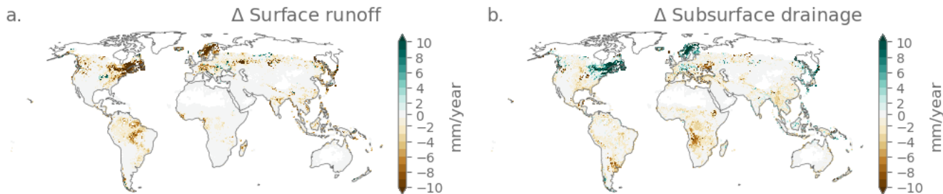
Figure 7. Effect of soil carbon sequestration on runoff. (a.) Difference in the High and CTL scenarios averaged over 20 simulation years for the column hosting crop fraction for surface runoff and (b.) subsurface drainage. Grid cells with organic soils (organic carbon content > 120 g C kg -1 soil) are excluded from the analysis.
