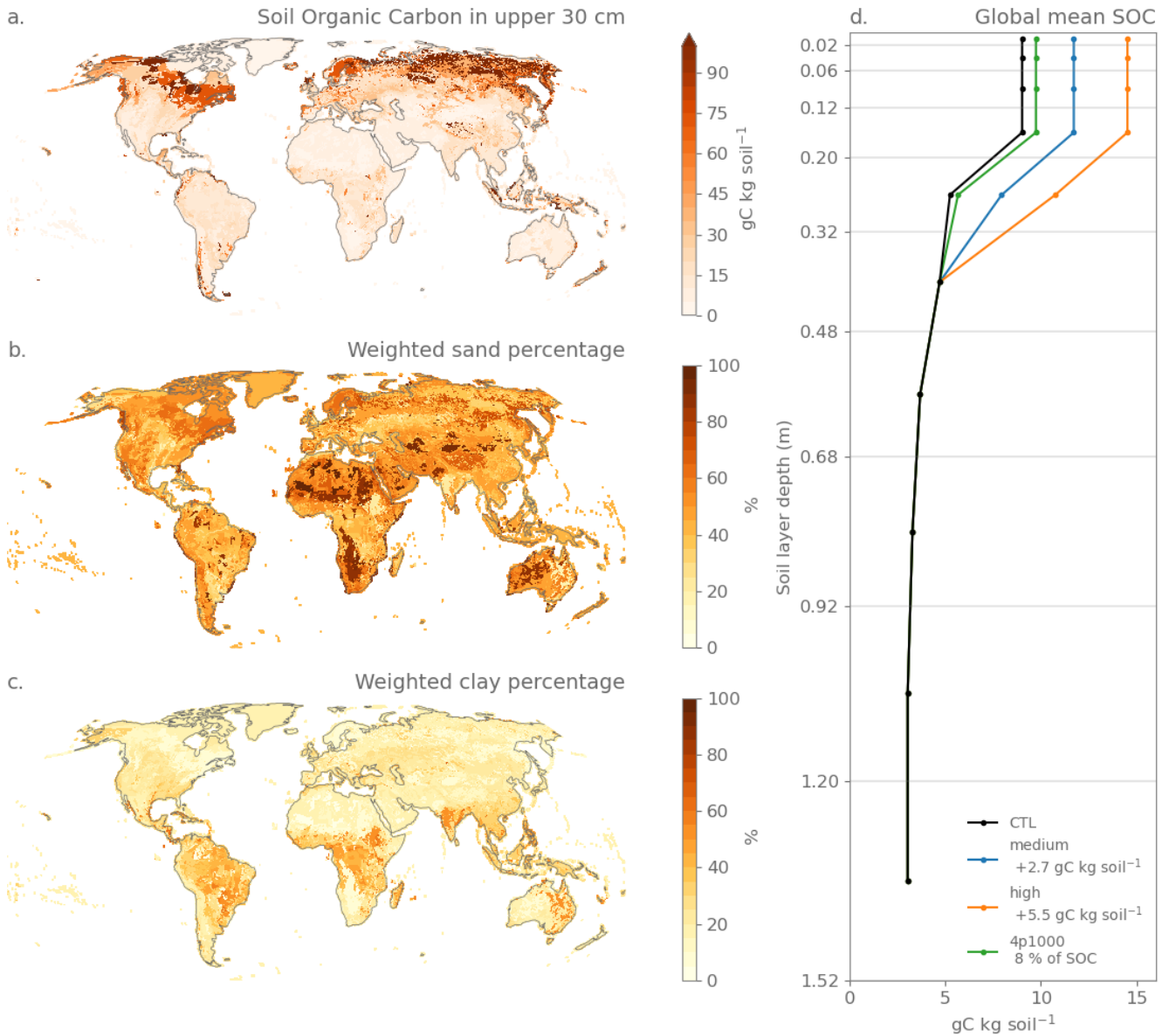
Figure 1. Soil Organic Carbon (SOC), sand and clay percentage and different soil carbon sequestration scenarios used as model input Soil Organic Carbon (SOC), soil textures and different soil carbon sequestration scenarios used as model input Spatial distribution of SOC in the top 30 cm of soil based on the WISE30sec dataset (a), weighted sand percentage sand (b) and clay percentage (c), both based on-weighted over the different soil layers following the WISE30sec dataset. Vertical profiles of global mean SOC in the control simulation (CTL) and the three soil carbon sequestration scenarios: medium, high, and 4p1000 (ed).
