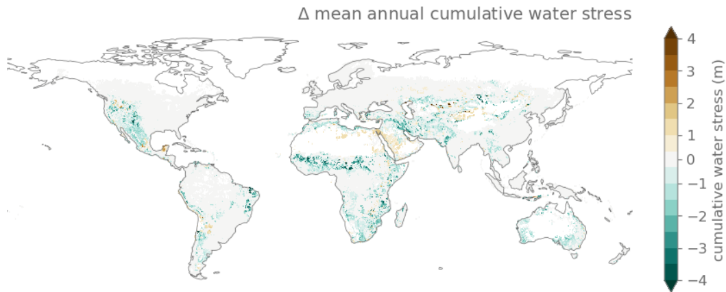
Figure 6. Effect of soil carbon sequestration scenario on water stress. (a.) Difference of annual cumulative water stress in the soil layers above 60 cm and (b.) the mean number of days per year with water stress in the High and Control scenarios for the column hosting crop fraction, annually averaged over a 20 simulation years. Grid cells with organic soils (organic carbon content > 120 g C kg -1 soil) are excluded from the analysis.
