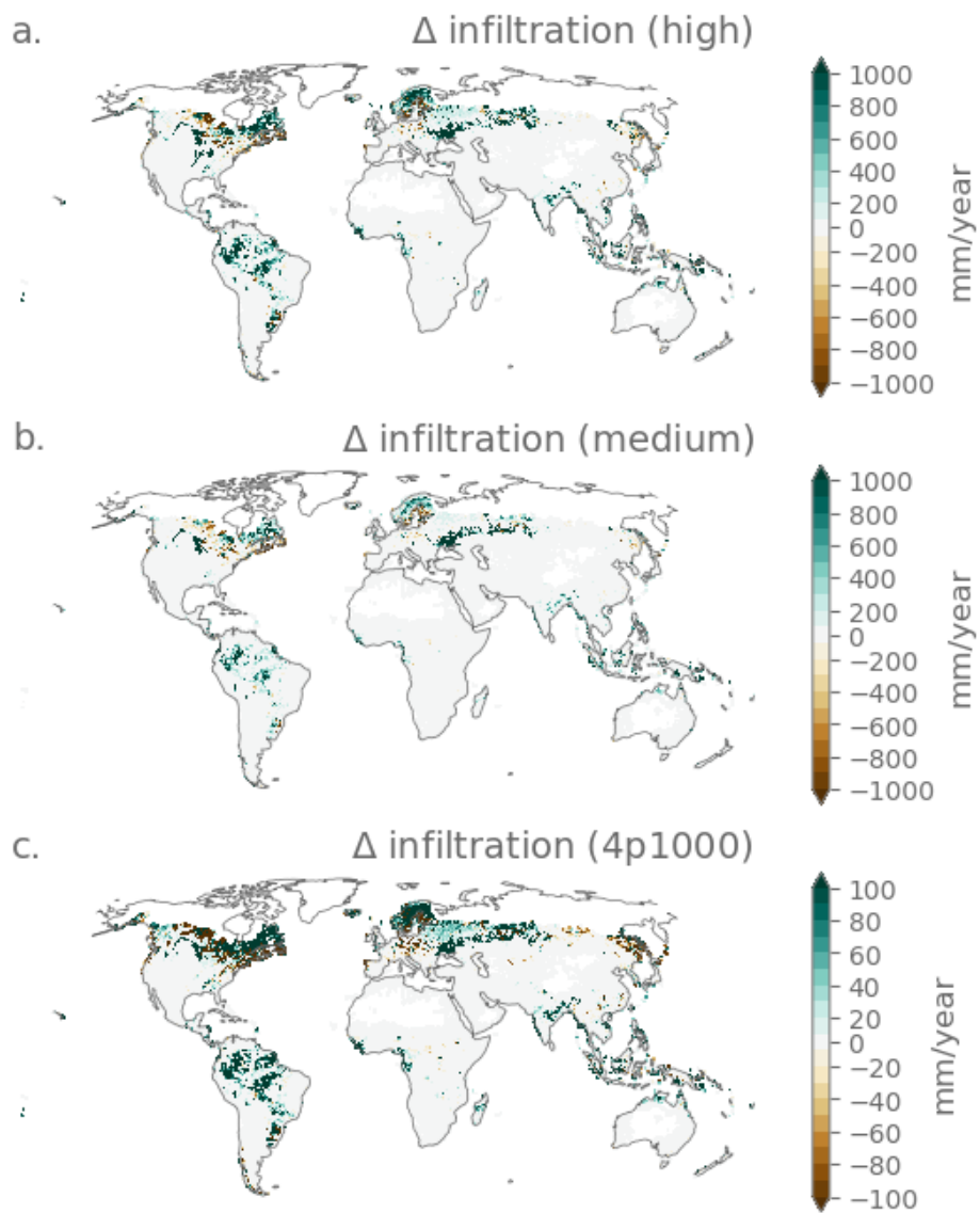
Figure A17. Effect of soil carbon sequestration on infiltration following the (a.) High, (b.) Medium and (c.) 4p1000 scenarios. Grid cells with organic soils (organic carbon content > 120 g C kg -1 soil) are excluded from the analysis.
