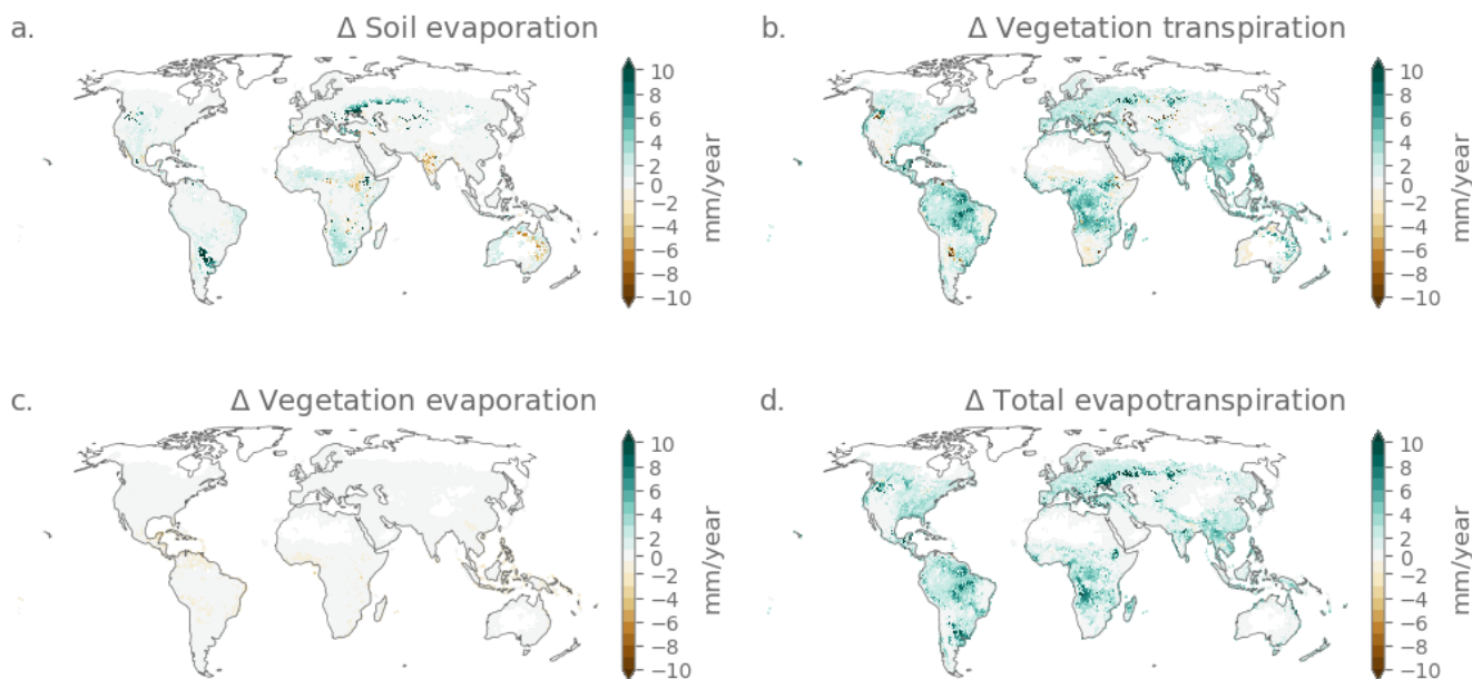
Figure 5. Effect of soil carbon sequestration on evapotranspiration. Difference in High and Control scenarios averaged over 20 simulation years for the column hosting crop fraction for (a.) soil evaporation, (b.) vegetation transpiration, (c.) vegetation evaporation and (d.) total evapotranspiration. Grid cells with organic soils (organic carbon content > 120 g C kg -1 soil) are excluded from the analysis.
