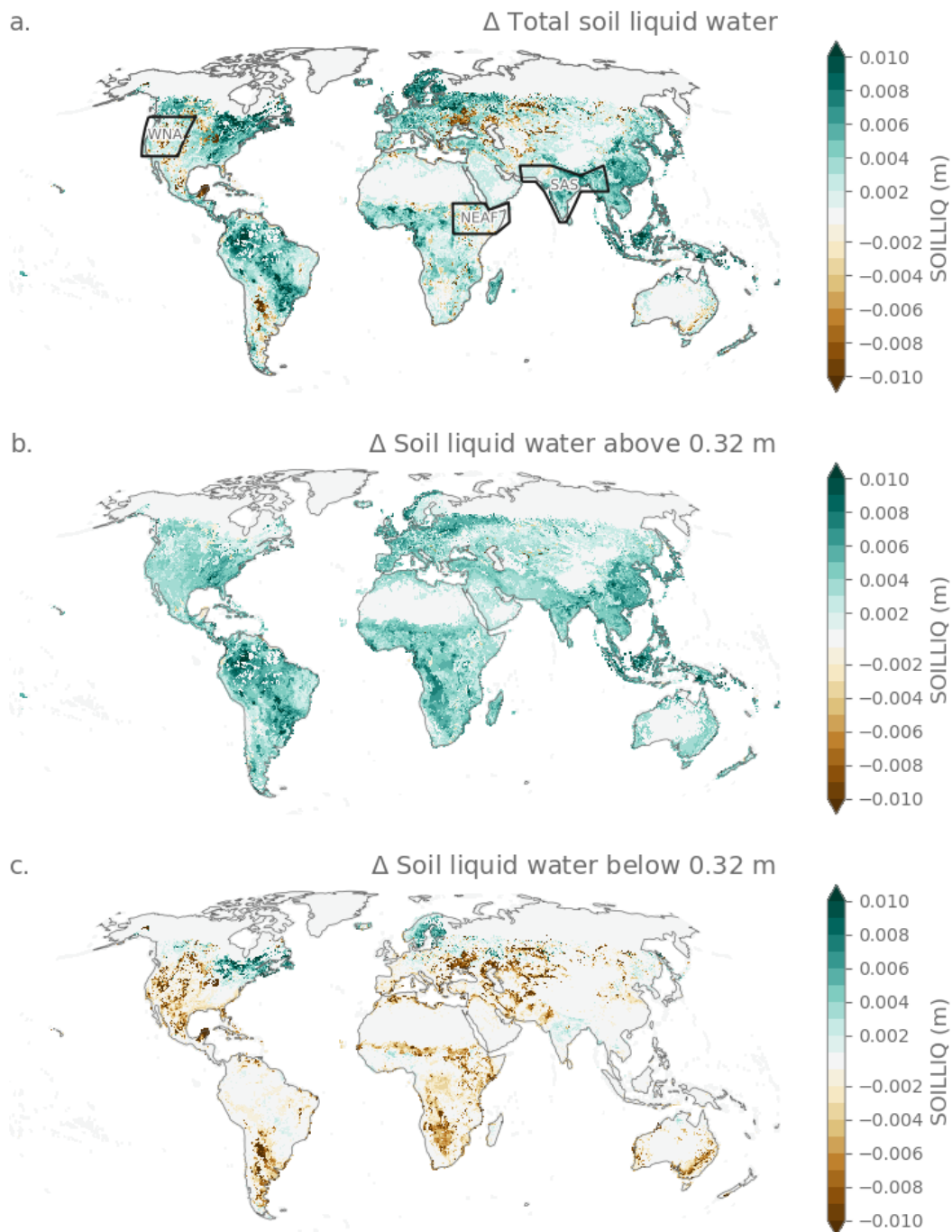
Figure 3. Effect of soil carbon sequestration scenario on soil liquid water content. Effect of soil carbon sequestration scenario on soil water content. Difference in High and CTL scenarios averaged over 20 simulation years for the column hosting crop fraction for total soil water content over the whole soil column. Black contours refer to the regions showed in Fig. A8 (a), liquid -water content above 32 cm, corresponding to the first five soil layers in CTSM (b) and liquid -water content below 32 cm (c). Grid cells with organic soils (organic carbon content > 120 g C kg -1 soil) are excluded from the analysis.
