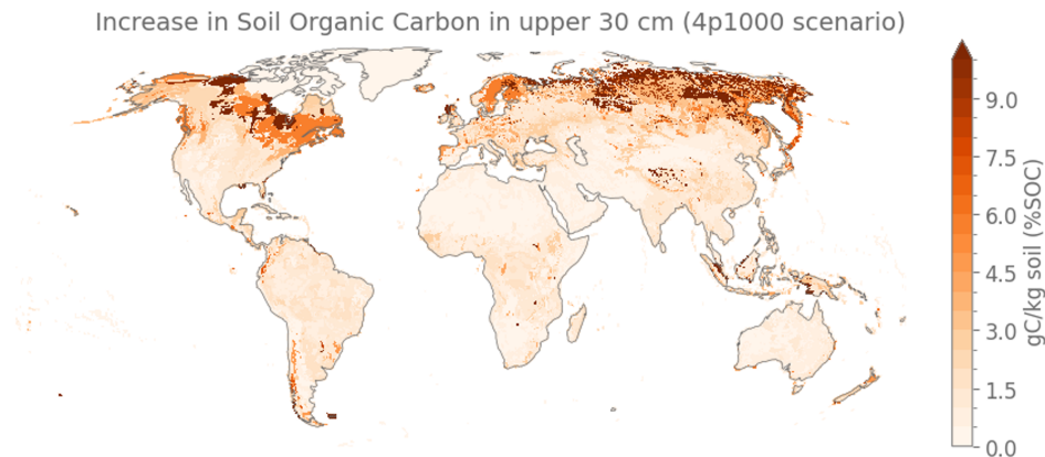
Illustration 4: Increase in SOC in the top 30 cm following the 4p1000 scenario, assuming a 0.4% annual increase of the current carbon stocks over a period of 20 years, corresponding to an 8% increase of present-day SOC
