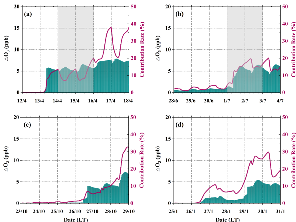
Fig 5. Hourly variations of near-surface \Delta O_3 (ppb, blue-filled areas) during the period of SI events (a) EP1, (b) EP2, (c) EP3 and (d) EP4 with their relative contribution proportions (RC) to the ambient atmosphere (dark red curve) averaged over the SCB. The gray shade indicates the regional O_3 pollution period.
