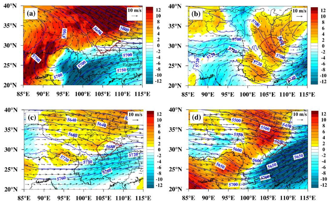
Fig 7. Geopotential height (in gpm; blue contours), wind vectors and vertical velocity ( \text{pa s}^{-1} ; shaded contours) at 500 hPa on (a) 16 April, (b) 1 July, (c) 26 October and (d) 29 January 2017. Positive values of vertical velocity denote subsidence.
