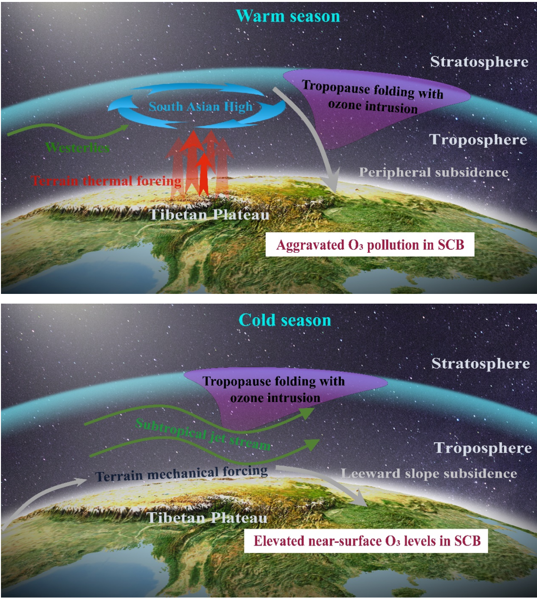
Fig 9. Diagram on the cross-layer transport of stratospheric O 3 on regional atmospheric environmental changes over SCB driven by multi-scale atmospheric circulation pattern with the seasonally discrepant terrain effects of TP.
