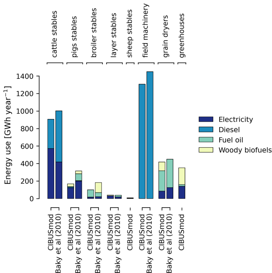
500 Figure 8. Energy use in stables, field machinery, grain dryers and greenhouses subdivided by energy source estimated in CIBUSmod compared to estimates by Baky et al. (2010).
