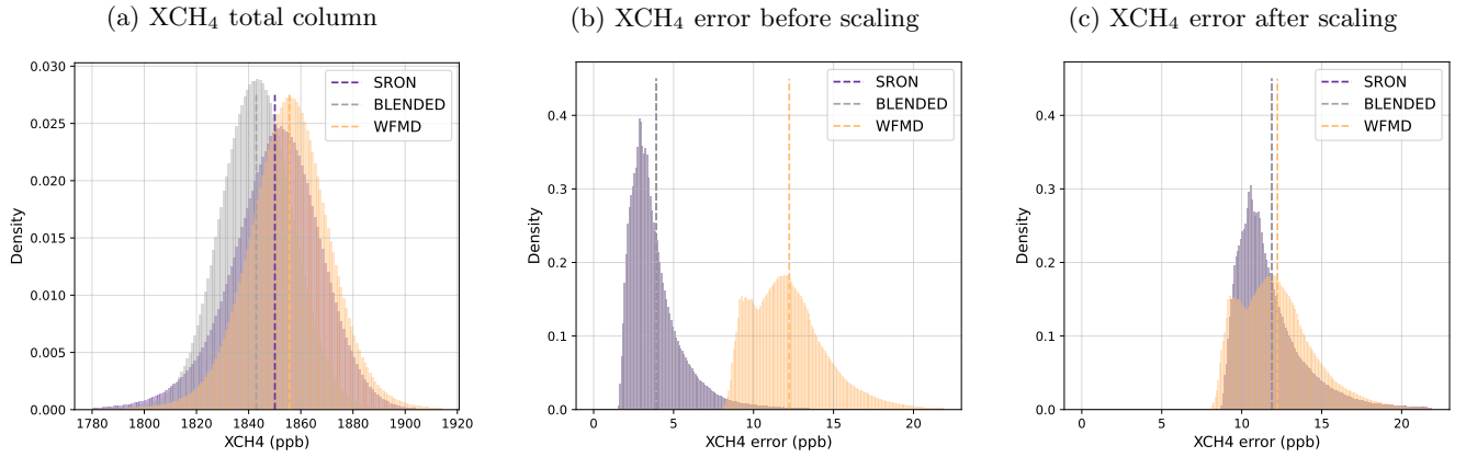
Figure 3. Distributions of observations and observation errors (both in ppb) for the three TROPOMI products. For the error, panel (b) shows the raw errors, while panel (c) shows the same histogram after error scaling for the SRON and BLENDED products. SRON and BLENDED errors are exactly similar, as BLENDED errors are directly retrieved from the SRON product.
