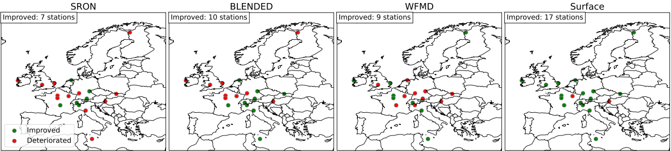
Figure D2. Evaluation map of the satellite-based and surface-based inversions: green (resp. red) circles are the surface stations for which the posterior simulated concentrations are in average closer (resp. further away) to the observations than the prior ones.
