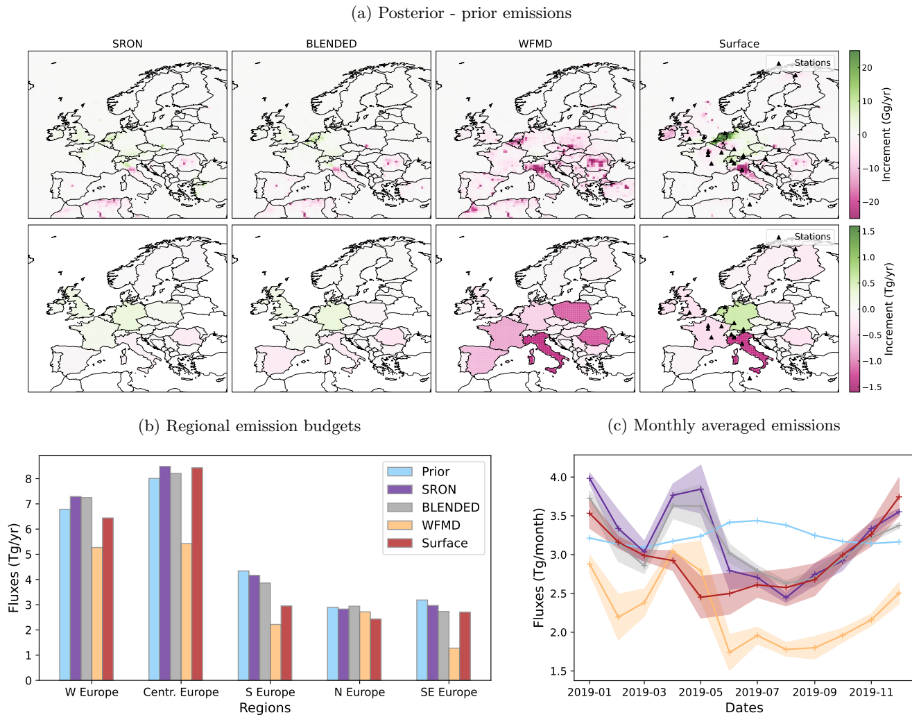
Figure 10. (a) Spatial distributions of the increments to the prior \text{CH}_4 emissions from the inversions, in \text{Gg/yr} at the grid-cell resolution (first row) and in \text{Tg/yr} at the national resolution (second row). (b) Total emissions for the regions described in Table B1, in \text{Tg/yr} . (c) Monthly variations of the \text{CH}_4 emissions in the domain in 2019, in \text{Tg/month} . The shaded areas show the standard deviation within each month.
