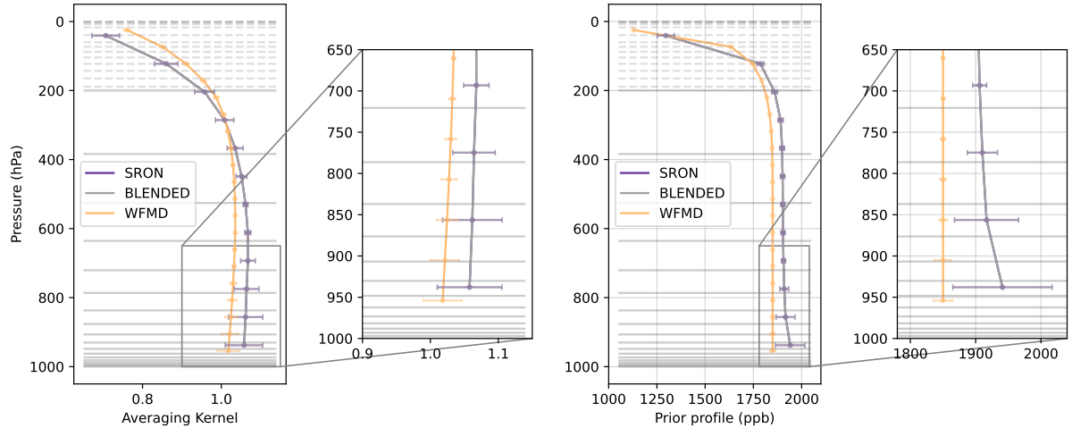
Figure 4. Column averaging kernels (left, unitless) and prior profiles (right, in ppb) averaged between the common observations of the TROPOMI products (dataset described in Section 2.1.1). The zoomed windows show the lower levels. SRON and BLENDED have exactly the same profile, since the only difference in the co-located dataset is the XCH 4 value. Horizontal lines are CHIMERE pressure levels (plain lines) and CAMS pressure levels in the stratosphere (dashed lines, for pressures lower than 200 hPa), for a surface pressure of 1000 hPa.
