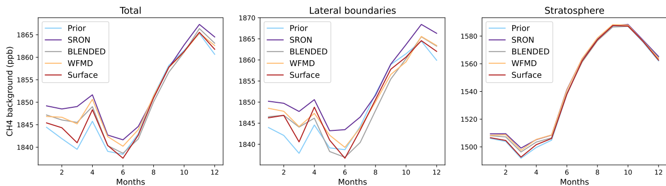
Figure D4. Time series of monthly averaged increments of the components of the background, for the 4 inversions presented in Section 2.4.2. The first panel shows the time series of averaged total columns, the second panel those with only the pixels used as lateral boundary conditions, and the third panel shows the time series of average stratosphere column (for pressures > 200 hPa).
