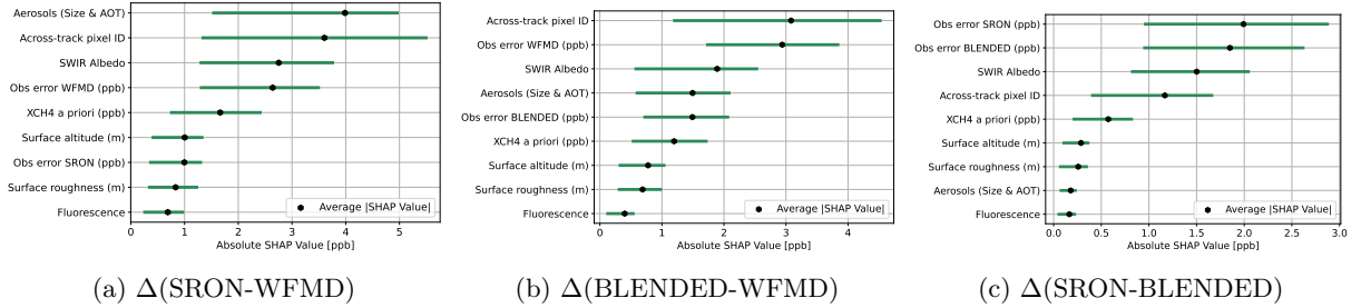
Figure 7. Contributions of the individual features to the \Delta XCH_4 predictions between pairs of TROPOMI products. The 9 most impacting predictors are ranked in order of importance. The contribution of a feature is defined as the average of absolute SHAP values, with the green bar showing the interquartile range.
