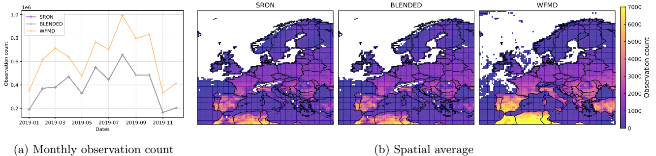
Figure 1. Number of observations per month (panel a ) and per 0.5^\circ longitude \times 0.5^\circ latitude cell 2019 (panel b ) for the three TROPOMI products SRON, BLENDED and WFMD used in this study. The covered period includes the change in pixel size (7.2 km to 5.6 km) in the along track direction, starting on the 6th of August 2019.
