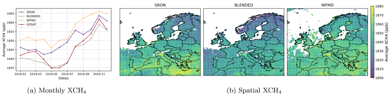
Figure 2. Average XCH_4 observation per month (Panel a ) and per 0.5^\circ \times 0.5^\circ cell in 2019 (Panel b ) for the three TROPOMI products.
