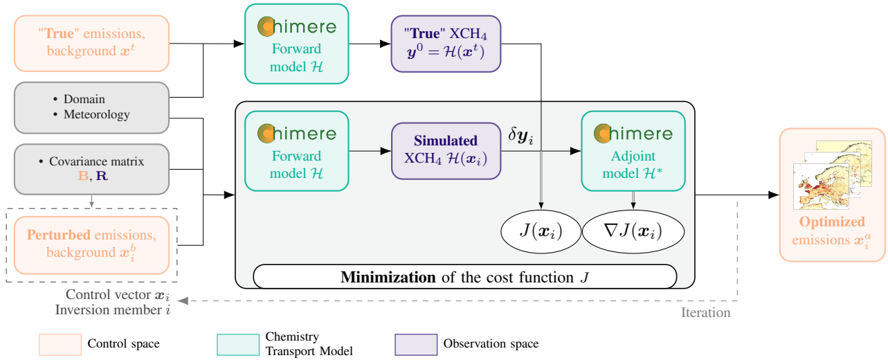
Figure 6. OSSE structure within the CIF. "True" pseudo-observations \mathbf{y}^0 are synthesized from the prior emissions \mathbf{x}^t and then assimilated in an ensemble of inversions using perturbed prior fluxes \mathbf{x}_i^b . See http://community-inversion.eu .
