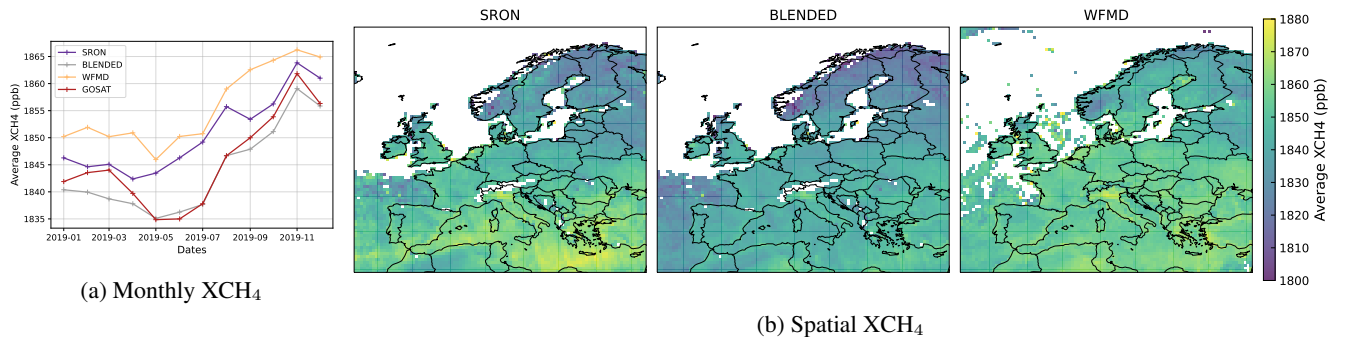
Figure 2. Average \text{XCH}_4 observation per month (Panel a ) and per 0.5^\circ \times 0.5^\circ cell in 2019 (Panel b ) for the three TROPOMI products.
