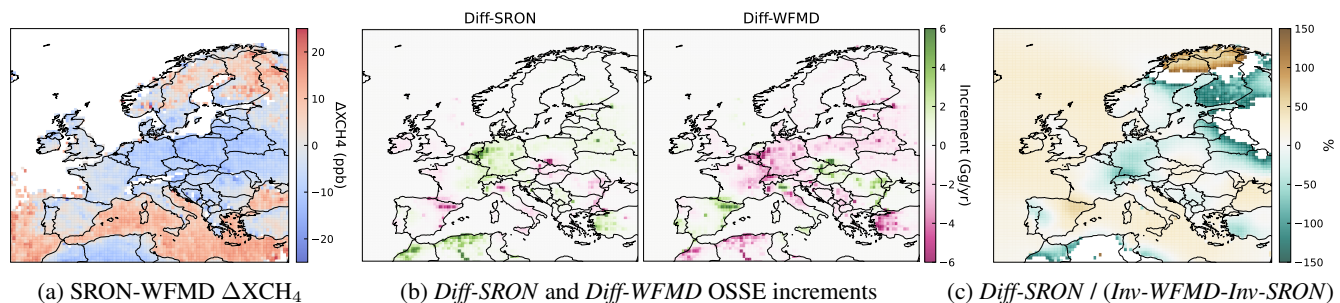
Figure 12. Spatial averages of (a) the \text{XCH}_4 difference SRON-WFMD (in ppb), (b) the increments of the Diff-SRON and Diff-WFMD OSSEs (in Gg/yr) and (c) of the ratio between the increments of Diff-SRON by the difference of increments between inversions Inv-WFMD and Inv-SRON (in %). For the last map (c), pixels with ratios above 150% (corresponding to very close increments in Inv-WFMD and Inv-SRON ) were filtered out.
