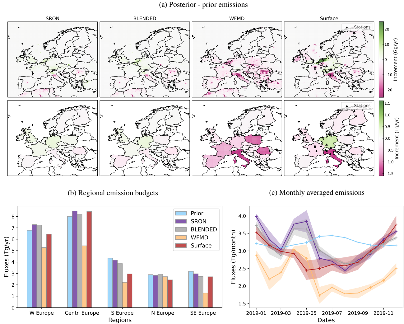
Figure 10. (a) Spatial distributions of the increments to the prior CH 4 emissions from the inversions, in Gg/yr at the grid-cell resolution (first row) and in Tg/yr at the national resolution (second row). (b) Total emissions for the regions described in Table B1, in Tg/yr. (c) Monthly variations of the CH 4 emissions in the domain in 2019, in Tg/month. The shaded areas show the standard deviation within each month.
