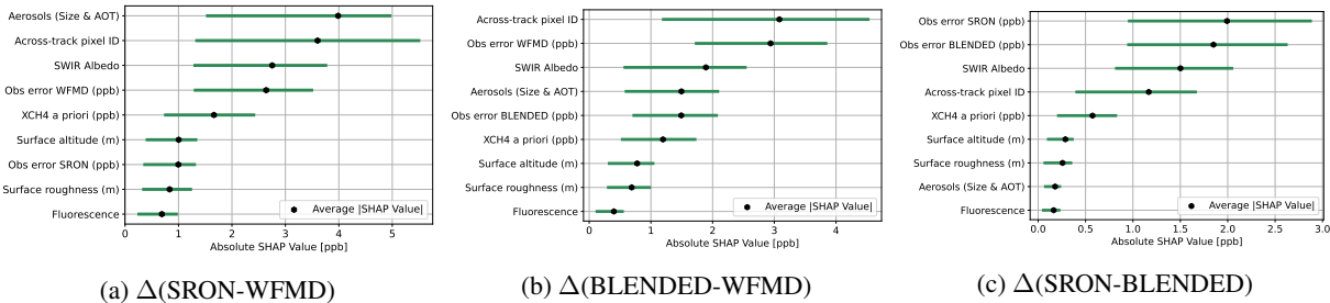
Figure 7. Contributions of the individual features to the \Delta\text{XCH}_4 predictions between pairs of TROPOMI products. The 9 most impacting predictors are ranked in order of importance. The contribution of a feature is defined as the average of absolute SHAP values, with the green bar showing the interquartile range.
