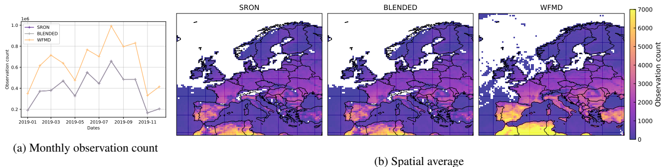
Figure 1. Number of observations per month (panel a ) and per 0.5^\circ longitude \times 0.5^\circ latitude cell 2019 (panel b ) for the three TROPOMI products SRON, BLENDED and WFMD used in this study. The covered period includes the change in pixel size (7.2 km to 5.6 km) in the along track direction, starting on the 6th of August 2019.
