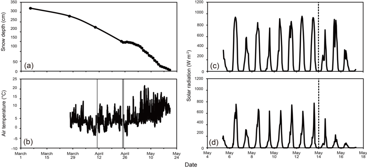
Figure 3: Meteorological conditions recorded at the study site. (a) Snow depth and (b) air temperature in the tree-covered area during the study period (March 1 to May 24). Gray-shaded periods represent intervals of missing data caused by instrument maintenance. Hourly mean intensity of solar radiation on the snow surface in the (c) tree-free and (d) tree-covered areas from May 4 to May 16. The timing of beech tree budburst is indicated by the dashed lines in (c) and (d).
